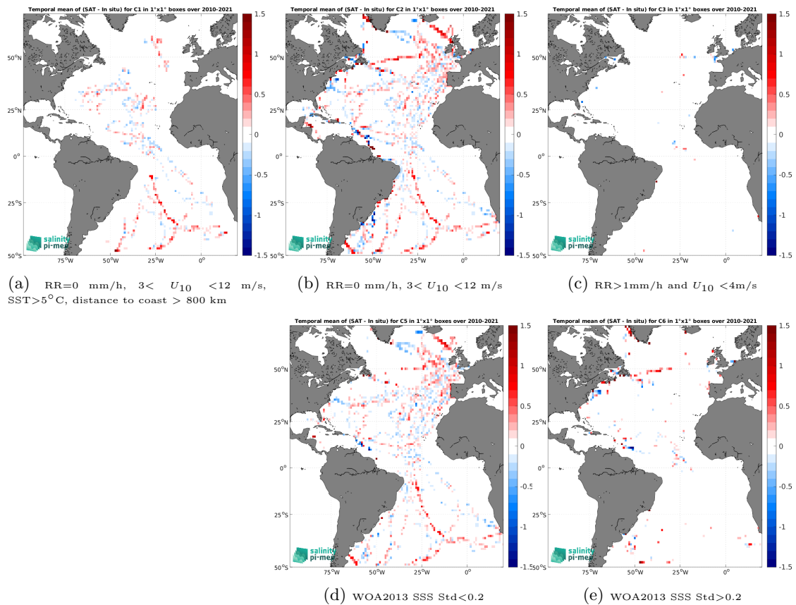
Figure 14: Temporal mean gridded over spatial boxes of size 1^\circ \times 1^\circ of \Delta\text{SSS} (SMOS SSS L3 v9 - 9 Days (CATDS-CEC-LOCEAN) - TSG (GOSUD-Sailing-ship)) for 5 different subdatasets corresponding to:RR=0 mm/h, 3 < U_{10} < 12 m/s, SST>5°C, distance to coast > 800 km (a), RR=0 mm/h, 3 < U_{10} < 12 m/s (b), RR>1mm/h and U_{10} < 4 m/s (c), WOA2013 SSS Std<0.2 (d), WOA2013 SSS Std>0.2 (e).
