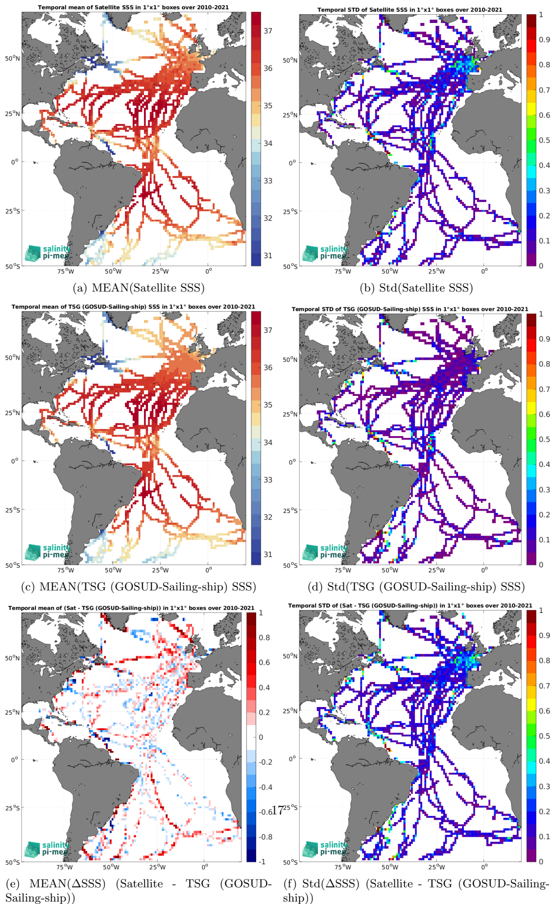
Figure 7: Temporal mean (left) and Std (right) of SSS from SMOS SSS L3 v9 - 9 Days (CATDS-CEC-LOCEAN) (top), TSG (GOSUD-Sailing-ship) (middle), and of \Delta SSS (Satellite - TSG (GOSUD-Sailing-ship)). Only match-up pairs are used to generate these maps.
