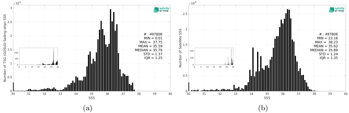
Figure 3: Histograms of SSS from TSG (GOSUD-Sailing-ship) (a) and SMOS SSS L3 v9 - 9 Days (CATDS-CEC-LOCEAN) (b) considering all match-up pairs per bins of 0.1 over the Atlantic Ocean Pi-MEP region and for the full satellite product period.
