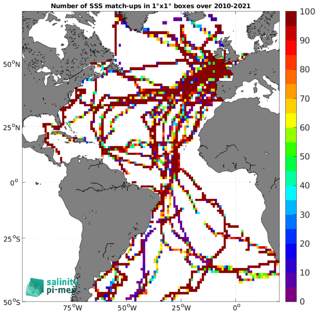
Figure 5: Number of SSS match-ups between TSG (GOSUD-Sailing-ship) SSS and the SMOS SSS L3 v9 - 9 Days (CATDS-CEC-LOCEAN) SSS product for the Atlantic Ocean Pi-MEP region over 1^{\circ} \times 1^{\circ} boxes and for the full satellite product period.
