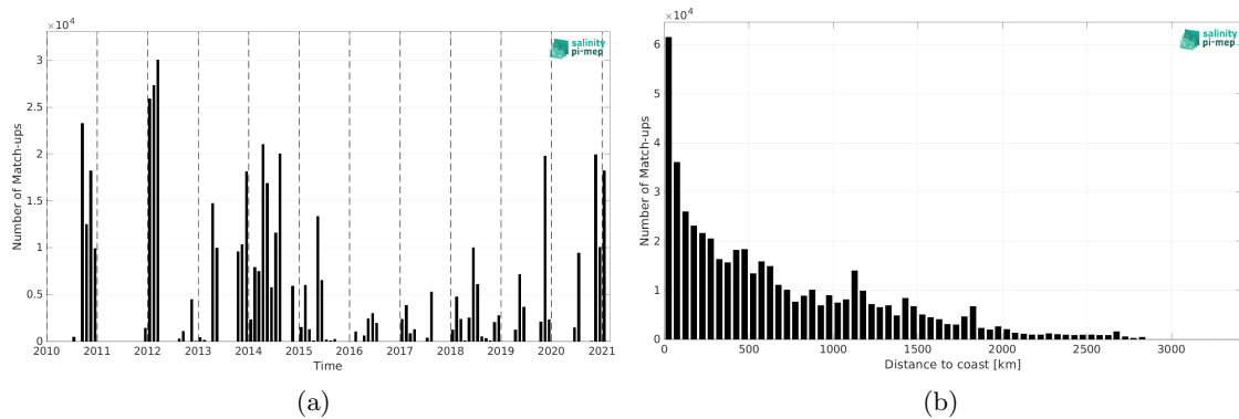
Figure 2: Number of match-ups between TSG (GOSUD-Sailing-ship) and SMOS SSS L3 v9 - 9 Days (CATDS-CEC-LOCEAN) SSS as a function of time (a) and as function of the distance to coast (b) over the Atlantic Ocean Pi-MEP region and for the full satellite product period.
