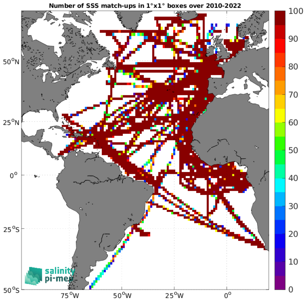
Figure 5: Number of SSS match-ups between TSG (GOSUD-Research-vessel) SSS and the SMOS SSS L3 v9 - 9 Days (CATDS-CEC-LOCEAN) SSS product for the Atlantic Ocean Pi-MEP region over 1^{\circ} \times 1^{\circ} boxes and for the full satellite product period.
