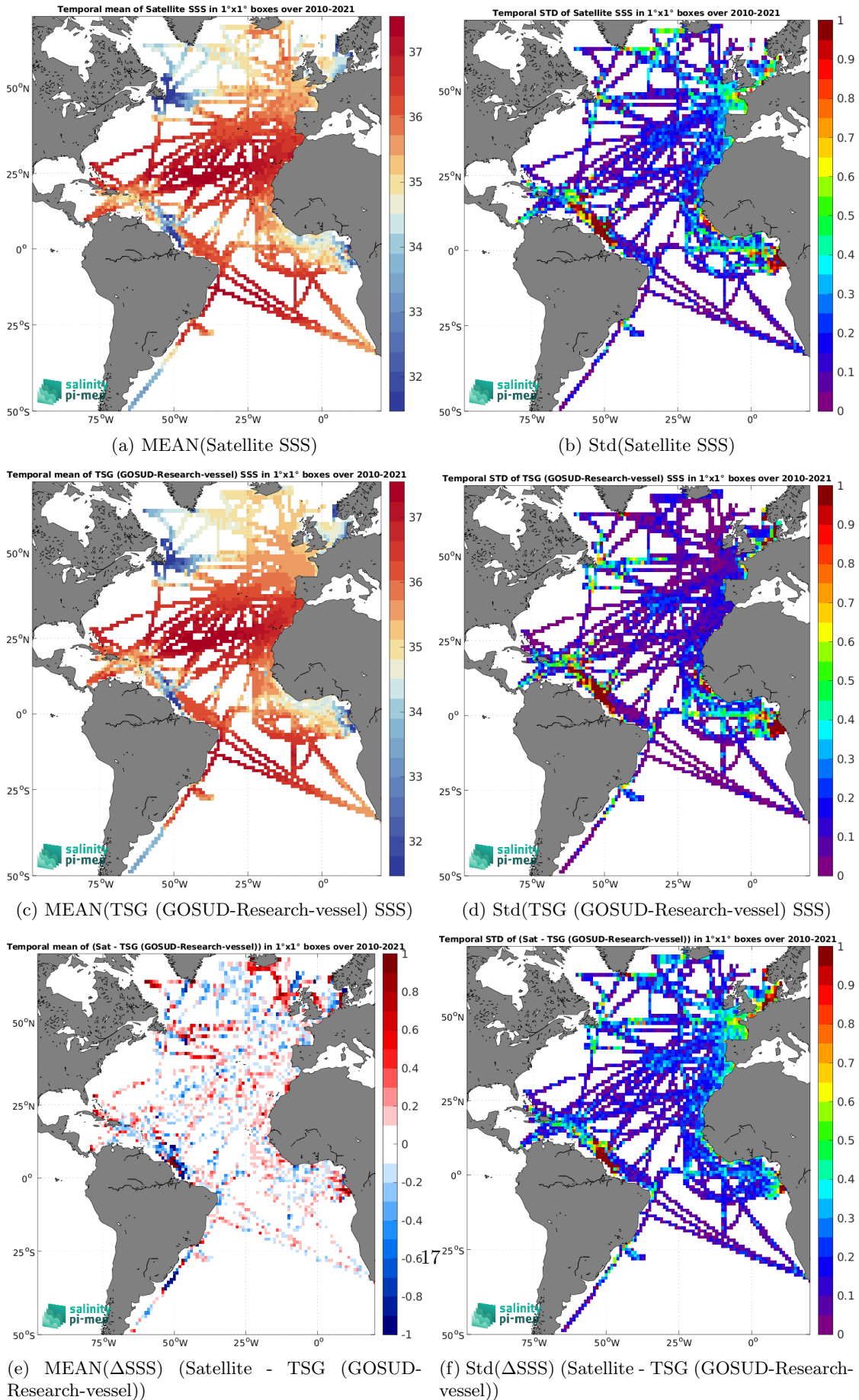
Figure 6: Temporal mean (left) and Std (right) of SSS from SMOS SSS L3 v9 - 9 Days (CATDS-CEC-LOCEAN) (top), TSG (GOSUD-Research-vessel) (middle), and of \Delta SSS (Satellite - TSG (GOSUD-Research-vessel)). Only match-up pairs are used to generate these maps.
