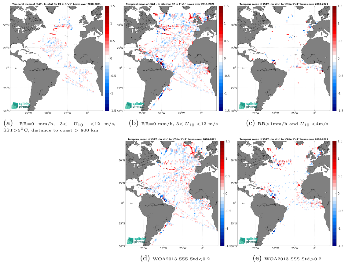
Figure 12: Temporal mean gridded over spatial boxes of size 1^\circ \times 1^\circ of \Delta\text{SSS} (SMOS SSS L3 v9 - 9 Days (CATDS-CEC-LOCEAN) - TSG (GOSUD-Research-vessel)) for 5 different subdatasets corresponding to:RR=0 mm/h, 3 < U_{10} < 12 m/s, SST>5°C, distance to coast > 800 km (a), RR=0 mm/h, 3 < U_{10} < 12 m/s (b), RR>1mm/h and U_{10} < 4 m/s (c), WOA2013 SSS Std<0.2 (d), WOA2013 SSS Std>0.2 (e).
