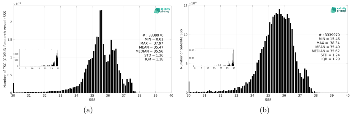
Figure 2: Histograms of SSS from TSG (GOSUD-Research-vessel) (a) and SMOS SSS L3 v9 - 9 Days (CATDS-CEC-LOCEAN) (b) considering all match-up pairs per bins of 0.1 over the Atlantic Ocean Pi-MEP region and for the full satellite product period.
