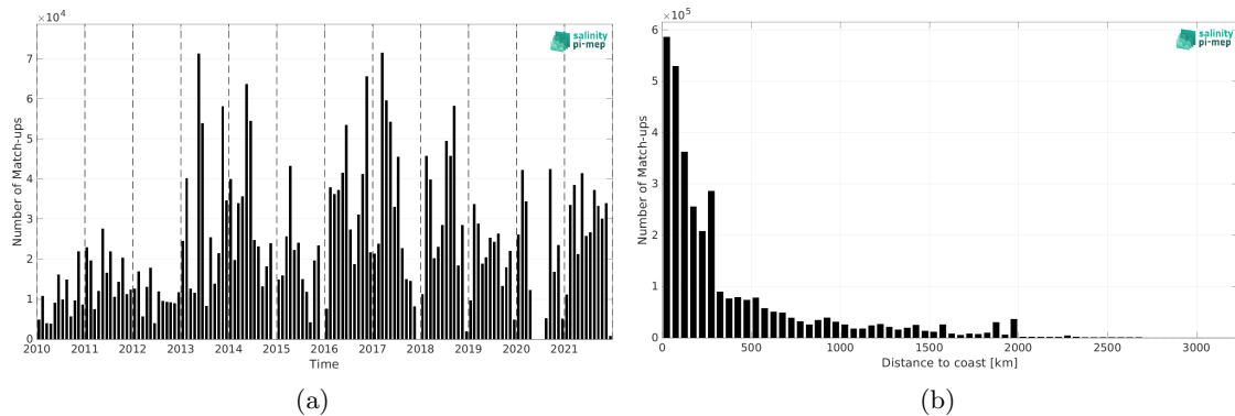
Figure 1: Number of match-ups between TSG (GOSUD-Research-vessel) and SMOS SSS L3 v9 - 9 Days (CATDS-CEC-LOCEAN) SSS as a function of time (a) and as function of the distance to coast (b) over the Atlantic Ocean Pi-MEP region and for the full satellite product period.
