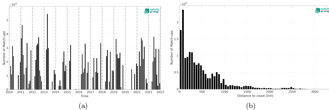
Figure 1: Number of match-ups between TSG (CSIC-UTM) and SMOS SSS L3 v9 - 9 Days (CATDS-CEC-LOCEAN) SSS as a function of time (a) and as function of the distance to coast (b) over the Atlantic Ocean Pi-MEP region and for the full satellite product period.
