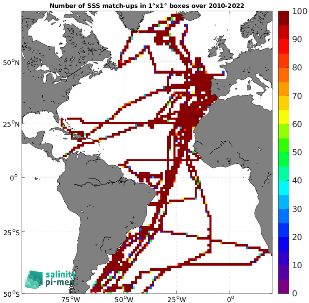
Figure 4: Number of SSS match-ups between TSG (CSIC-UTM) SSS and the SMOS SSS L3 v9 - 9 Days (CATDS-CEC-LOCEAN) SSS product for the Atlantic Ocean Pi-MEP region over 1^\circ \times 1^\circ boxes and for the full satellite product period.
