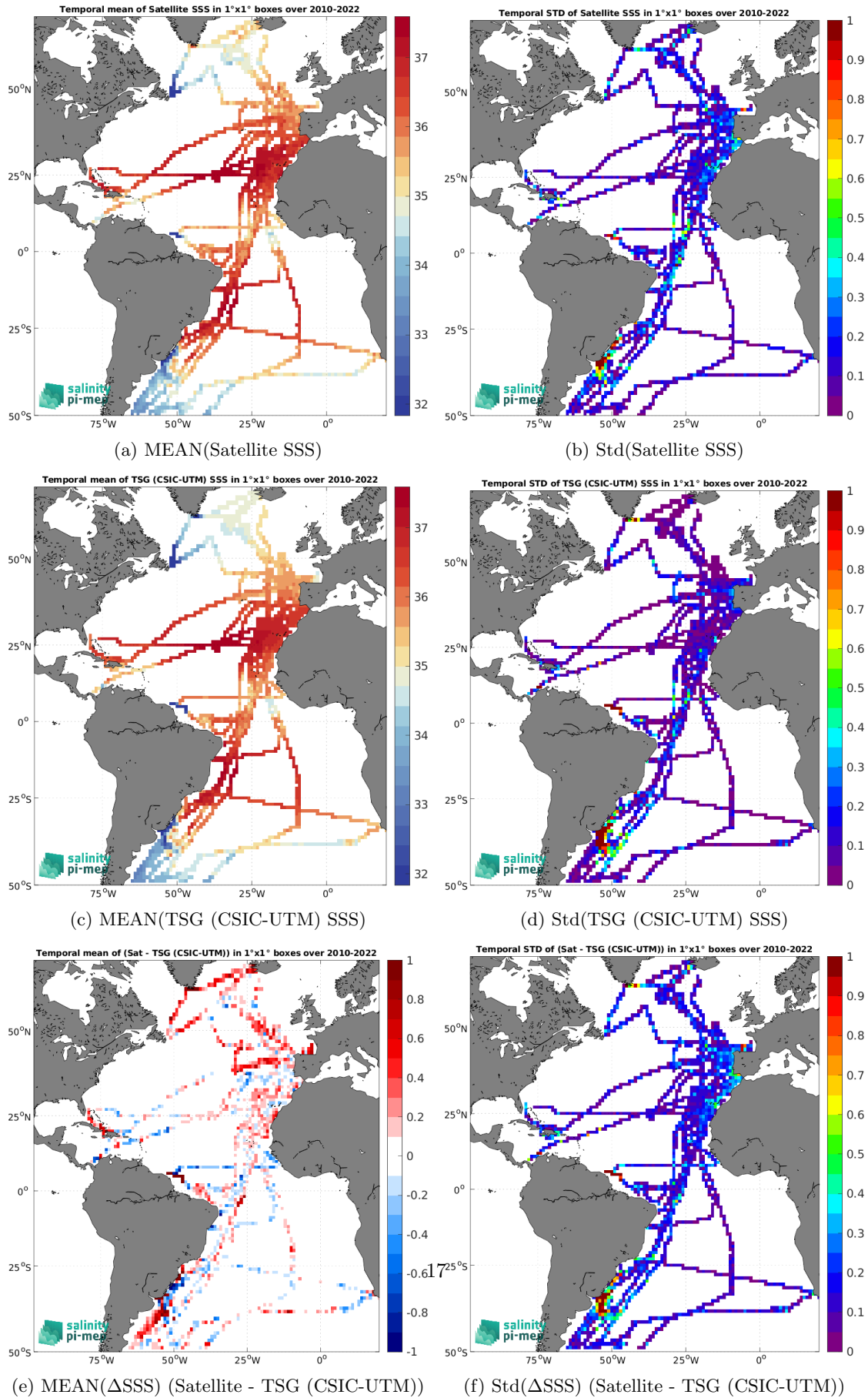
Figure 6: Temporal mean (left) and Std (right) of SSS from SMOS SSS L3 v9 - 9 Days (CATDS-CEC-LOCEAN) (top), TSG (CSIC-UTM) (middle), and of \Delta SSS (Satellite - TSG (CSIC-UTM)). Only match-up pairs are used to generate these maps.
