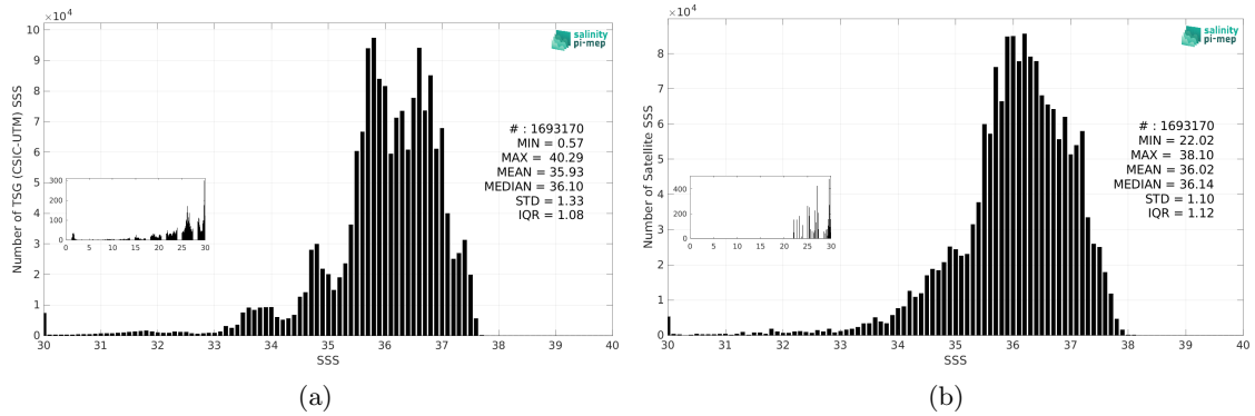
Figure 2: Histograms of SSS from TSG (CSIC-UTM) (a) and SMOS SSS L3 v9 - 9 Days (CATDS-CEC-LOCEAN) (b) considering all match-up pairs per bins of 0.1 over the Atlantic Ocean Pi-MEP region and for the full satellite product period.
