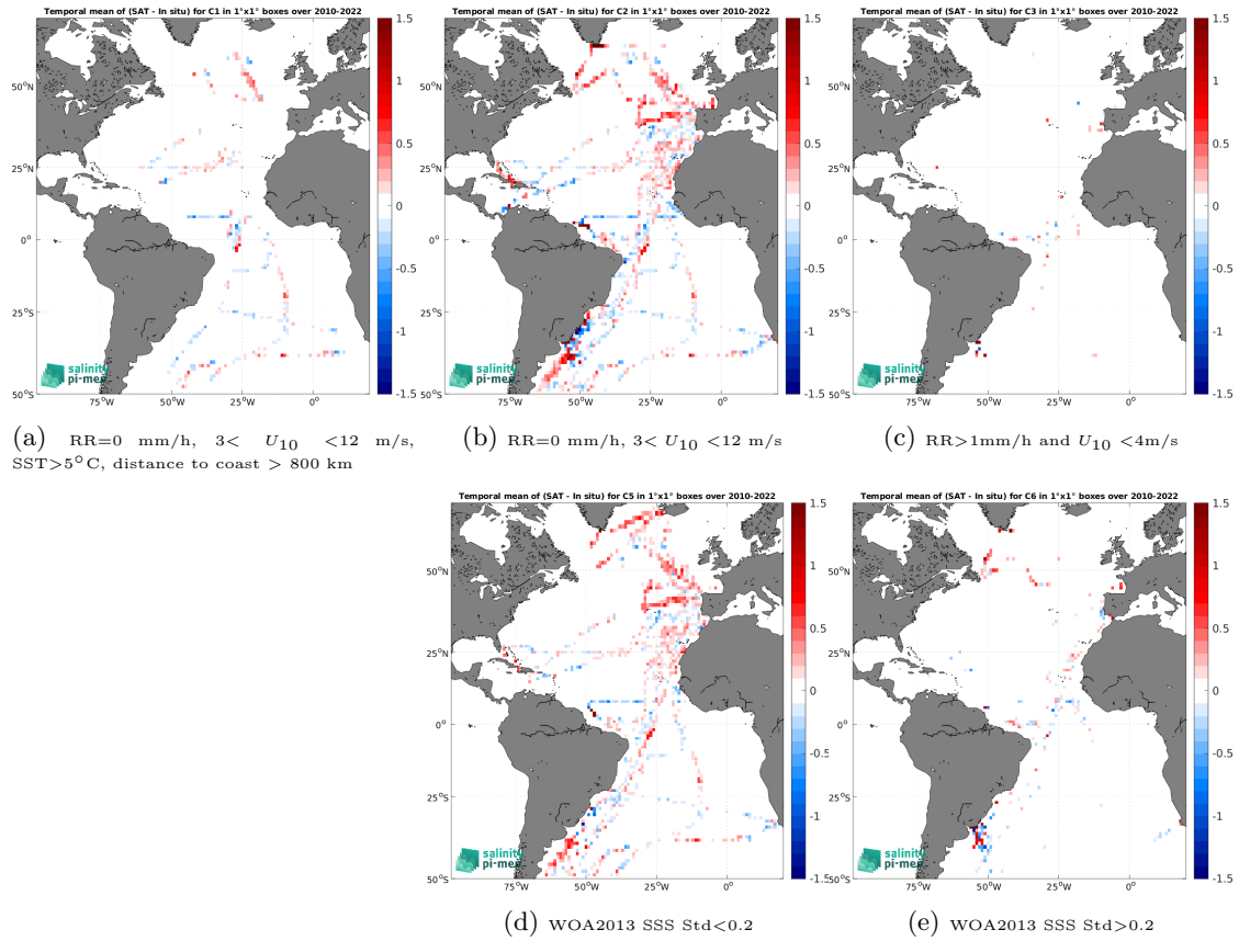
Figure 12: Temporal mean gridded over spatial boxes of size 1^\circ \times 1^\circ of \Delta SSS (SMOS SSS L3 v9 - 9 Days (CATDS-CEC-LOCEAN) - TSG (CSIC-UTM)) for 5 different subdatasets corresponding to:RR=0 mm/h, 3 < U_{10} < 12 m/s, SST >5^\circ\text{C} , distance to coast > 800 km (a), RR=0 mm/h, 3 < U_{10} < 12 m/s (b), RR >1 mm/h and U_{10} < 4 m/s (c), WOA2013 SSS Std <0.2 (d), WOA2013 SSS Std >0.2 (e).
