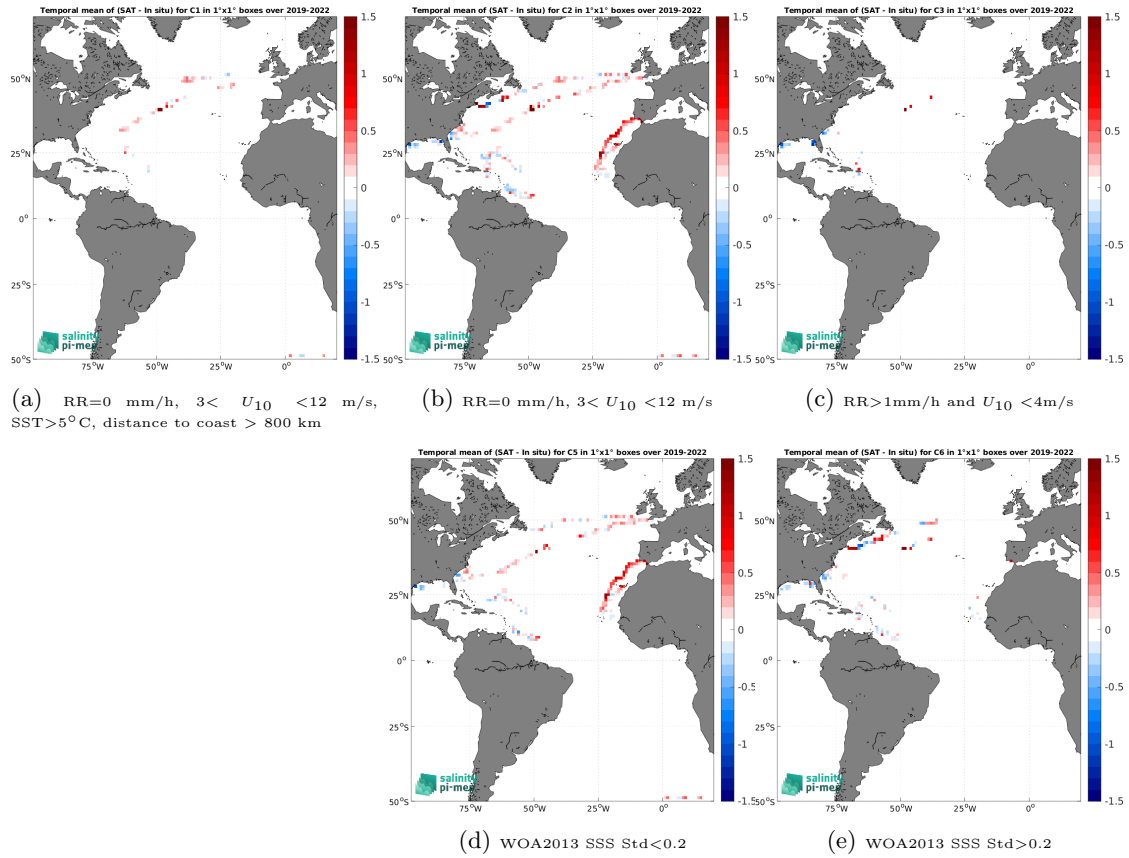
Figure 12: Temporal mean gridded over spatial boxes of size 1^\circ \times 1^\circ of \Delta SSS (SMOS SSS L3 v9 - 9 Days (CATDS-CEC-LOCEAN) - Saildrone) for 5 different subdatasets corresponding to:RR=0 mm/h, 3 < U_{10} < 12 m/s, SST >5^\circ\text{C} , distance to coast > 800 km (a), RR=0 mm/h, 3 < U_{10} < 12 m/s (b), RR >1 mm/h and U_{10} < 4 m/s (c), WOA2013 SSS Std <0.2 (d), WOA2013 SSS Std >0.2 (e).
