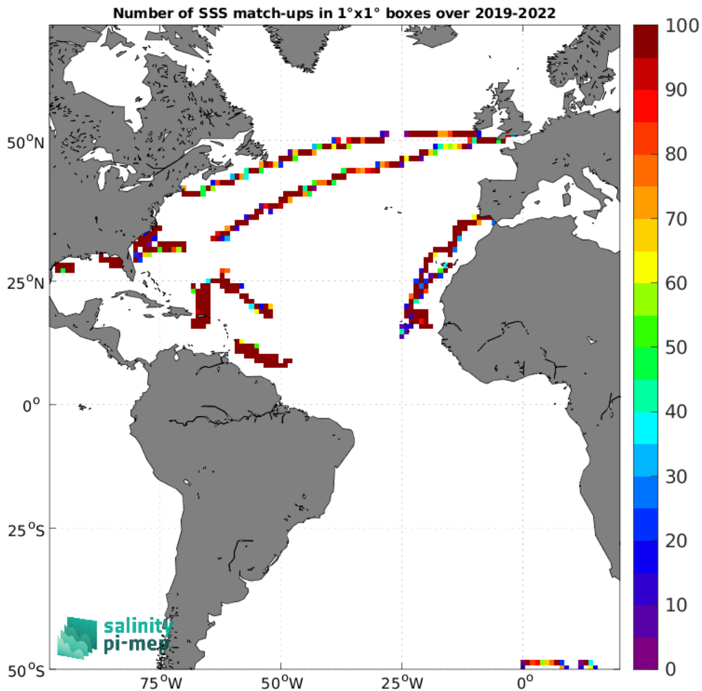
Figure 4: Number of SSS match-ups between Saildrone SSS and the SMOS SSS L3 v9 - 9 Days (CATDS-CEC-LOCEAN) SSS product for the Atlantic Ocean Pi-MEP region over 1^\circ \times 1^\circ boxes and for the full satellite product period.
