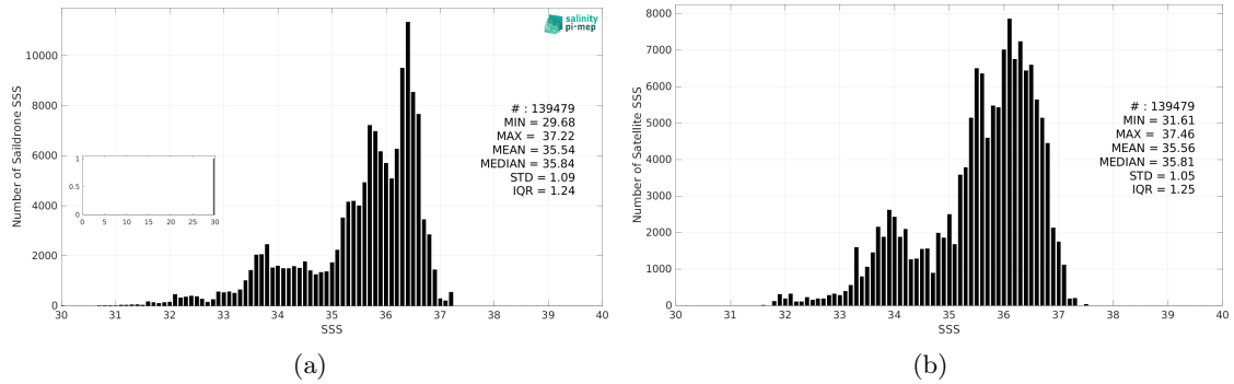
Figure 2: Histograms of SSS from Sairdrone (a) and SMOS SSS L3 v9 - 9 Days (CATDS-CEC-LOCEAN) (b) considering all match-up pairs per bins of 0.1 over the Atlantic Ocean Pi-MEP region and for the full satellite product period.
