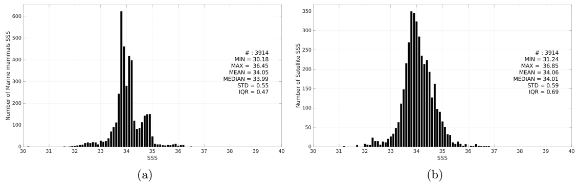
Figure 3: Histograms of SSS from Marine mammals (a) and SMOS SSS L3 v9 - 9 Days (CATDS-CEC-LOCEAN) (b) considering all match-up pairs per bins of 0.1 over the Atlantic Ocean Pi-MEP region and for the full satellite product period.
