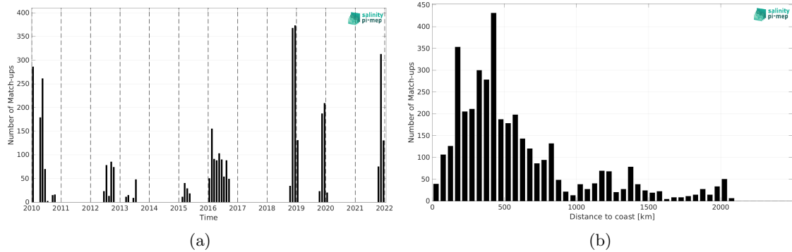
Figure 2: Number of match-ups between Marine mammals and SMOS SSS L3 v9 - 9 Days (CATDS-CEC-LOCEAN) SSS as a function of time (a) and as function of the distance to coast (b) over the Atlantic Ocean Pi-MEP region and for the full satellite product period.
