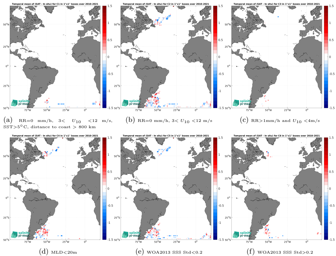
Figure 14: Temporal mean gridded over spatial boxes of size 1^\circ \times 1^\circ of \Delta SSS (SMOS SSS L3 v9 - 9 Days (CATDS-CEC-LOCEAN) - Marine mammals) for 6 different subdatasets corresponding to:RR=0 mm/h, 3 < U_{10} < 12 m/s, SST>5°C, distance to coast > 800 km (a), RR=0 mm/h, 3 < U_{10} < 12 m/s (b), RR>1mm/h and U_{10} < 4 m/s (c),MLD<20m (d),WOA2013 SSS Std<0.2 (e),WOA2013 SSS Std>0.2 (f).
