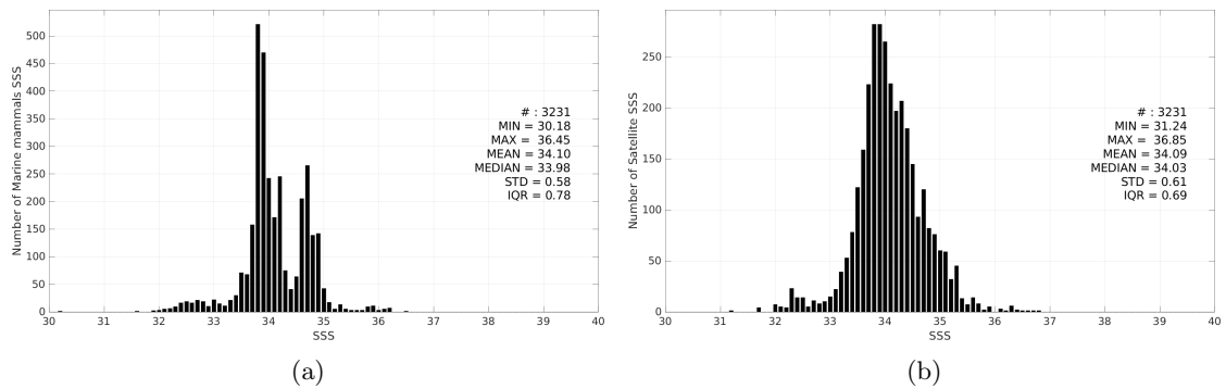
Figure 2: Histograms of SSS from Marine mammals (a) and SMOS SSS L3 v9 - 9 Days (CATDS-CEC-LOCEAN) (b) considering all match-up pairs per bins of 0.1 over the Atlantic Ocean Pi-MEP region and for the full satellite product period.
