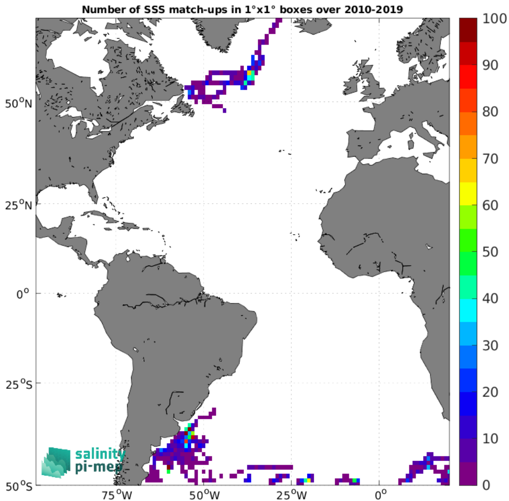
Figure 4: Number of SSS match-ups between Marine mammals SSS and the SMOS SSS L3 v9 - 9 Days (CATDS-CEC-LOCEAN) SSS product for the Atlantic Ocean Pi-MEP region over 1°x1° boxes and for the full satellite product period.
