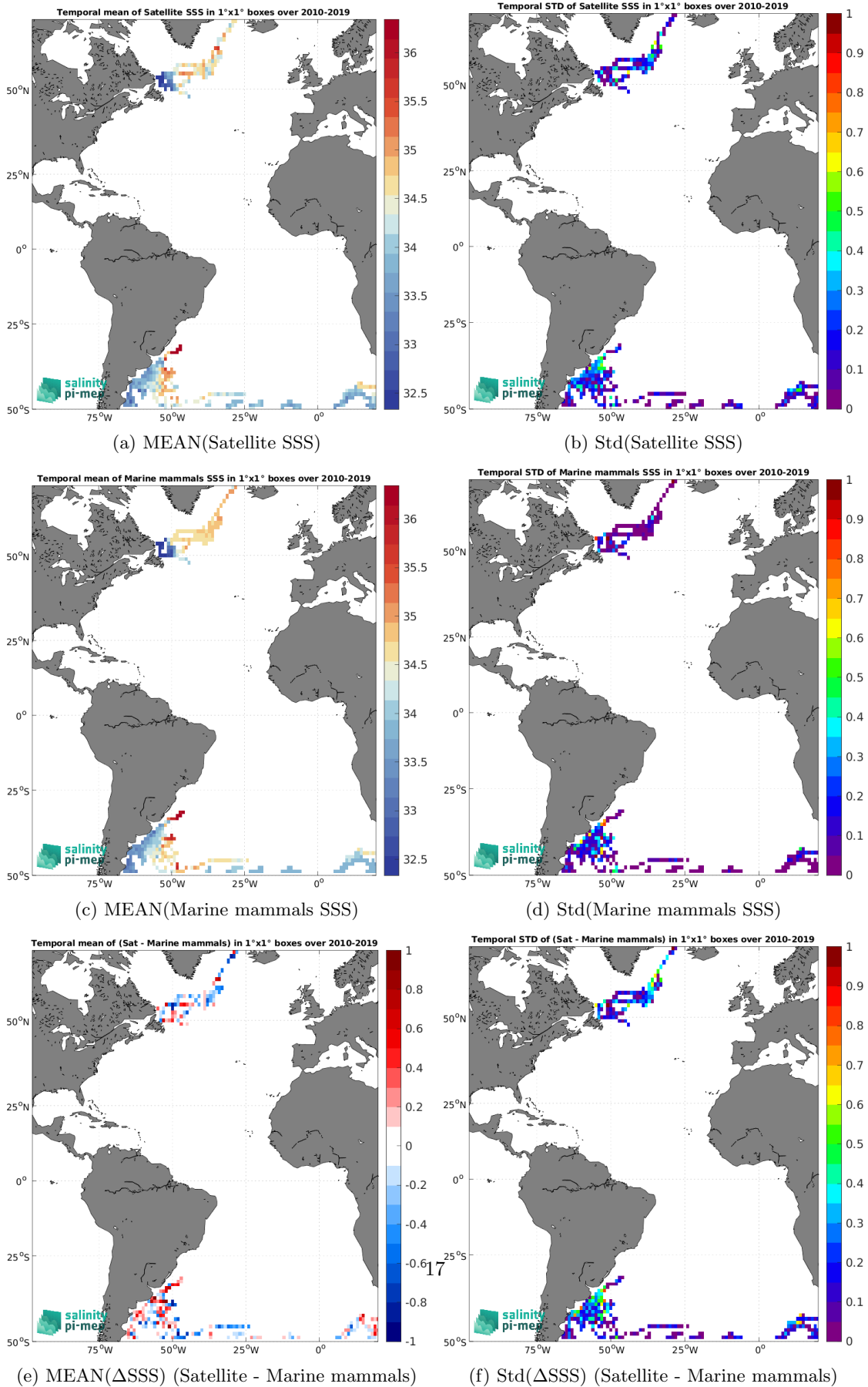
Figure 6: Temporal mean (left) and Std (right) of SSS from SMOS SSS L3 v9 - 9 Days (CATDS-CEC-LOCEAN) (top), Marine mammals (middle), and of \Delta SSS (Satellite - Marine mammals). Only match-up pairs are used to generate these maps.
