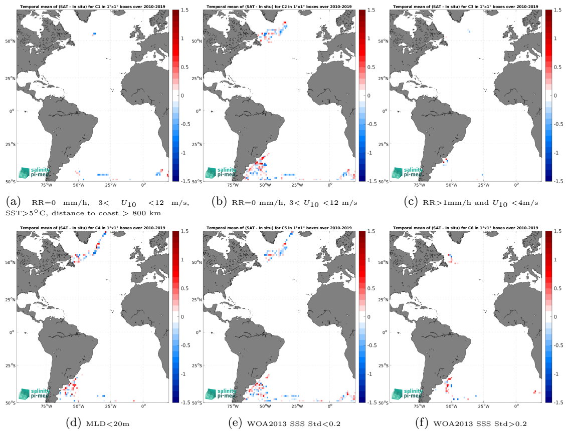
Figure 12: Temporal mean gridded over spatial boxes of size 1^\circ \times 1^\circ of \Delta SSS (SMOS SSS L3 v9 - 9 Days (CATDS-CEC-LOCEAN) - Marine mammals) for 6 different subdatasets corresponding to: RR=0 mm/h, 3 < U_{10} < 12 m/s, SST > 5°C, distance to coast > 800 km (a), RR=0 mm/h, 3 < U_{10} < 12 m/s (b), RR > 1mm/h and U_{10} < 4 m/s (c), MLD < 20m (d), WOA2013 SSS Std < 0.2 (e), WOA2013 SSS Std > 0.2 (f).
