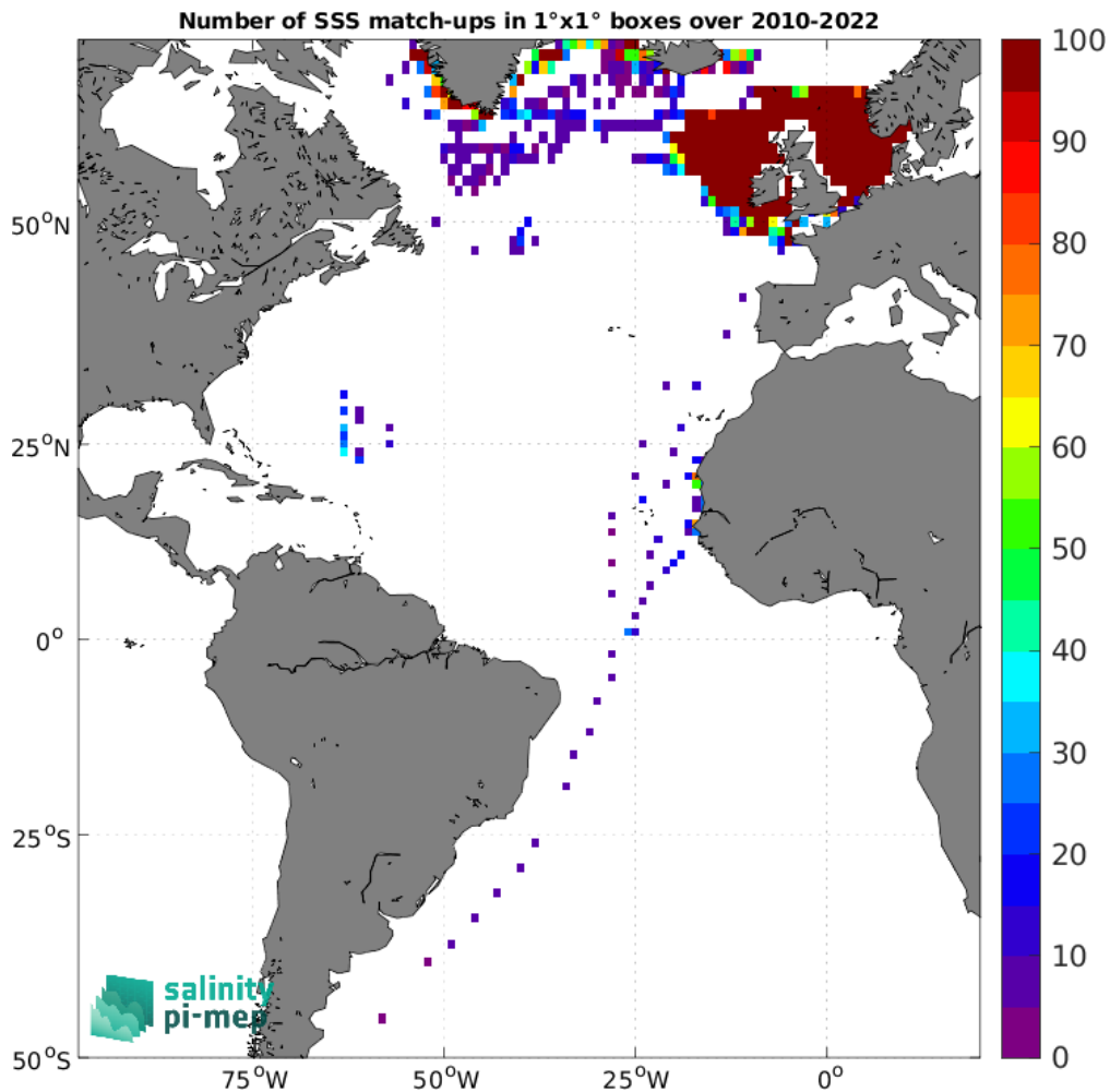
Figure 5: Number of SSS match-ups between ICES SSS and the SMOS SSS L3 v9 - 9 Days (CATDS-CEC-LOCEAN) SSS product for the Atlantic Ocean Pi-MEP region over 1^\circ \times 1^\circ boxes and for the full satellite product period.
