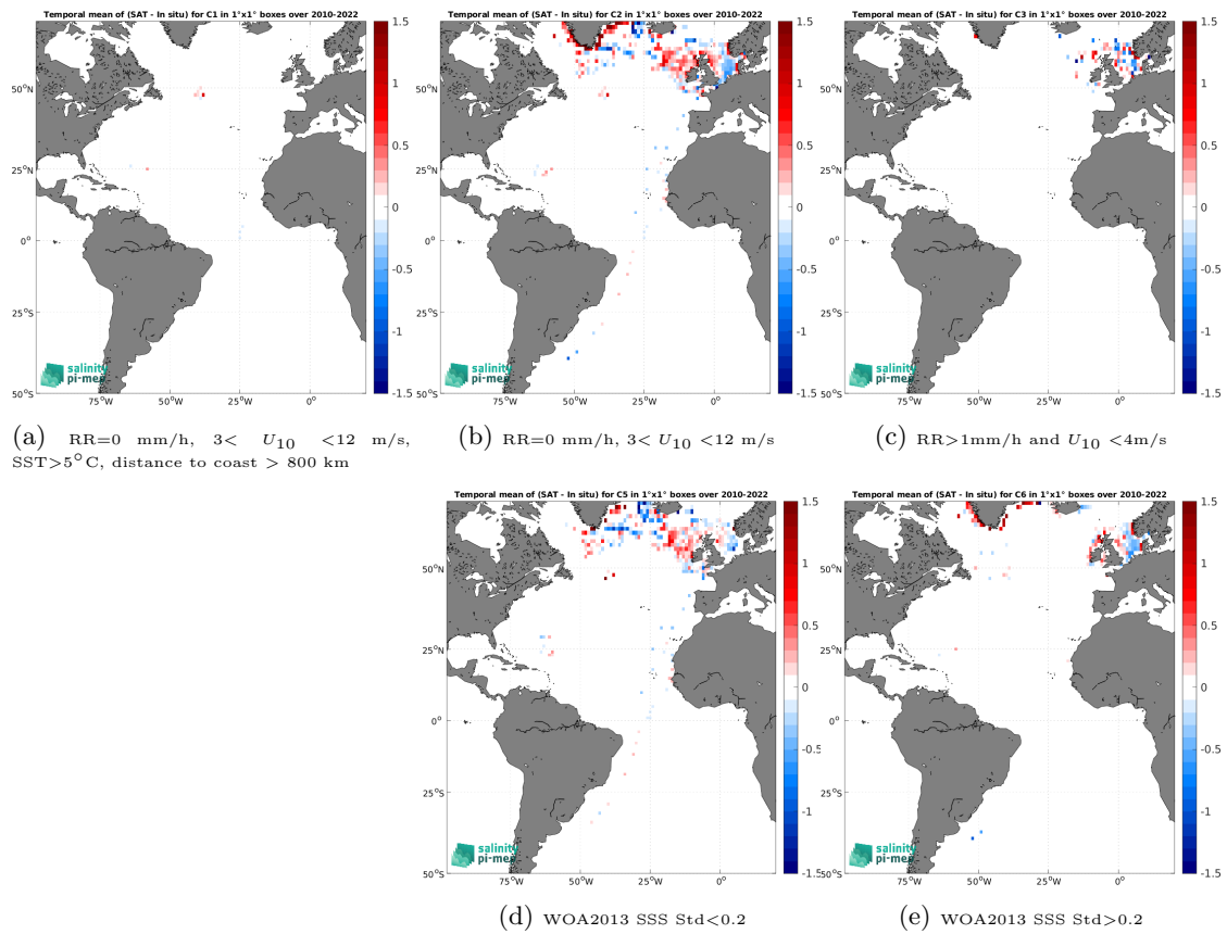
Figure 14: Temporal mean gridded over spatial boxes of size 1^\circ \times 1^\circ of \Delta\text{SSS} (SMOS SSS L3 v9 - 9 Days (CATDS-CEC-LOCEAN) - ICES) for 5 different subdatasets corresponding to:RR=0 mm/h, 3 < U_{10} < 12 m/s, SST>5°C, distance to coast > 800 km (a), RR=0 mm/h, 3 < U_{10} < 12 m/s (b), RR>1mm/h and U_{10} < 4 m/s (c), WOA2013 SSS Std<0.2 (d), WOA2013 SSS Std>0.2 (e).
