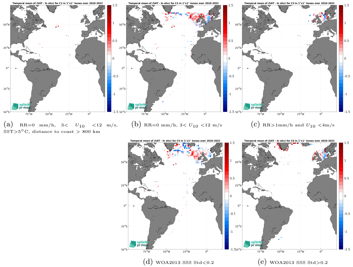
Figure 12: Temporal mean gridded over spatial boxes of size 1^\circ \times 1^\circ of \Delta SSS (SMOS SSS L3 v9 - 9 Days (CATDS-CEC-LOCEAN) - ICES) for 5 different subdatasets corresponding to:RR=0 mm/h, 3 < U_{10} < 12 m/s, SST >5^\circ\text{C} , distance to coast > 800 km (a), RR=0 mm/h, 3 < U_{10} < 12 m/s (b), RR >1 mm/h and U_{10} < 4 m/s (c), WOA2013 SSS Std <0.2 (d), WOA2013 SSS Std >0.2 (e).
