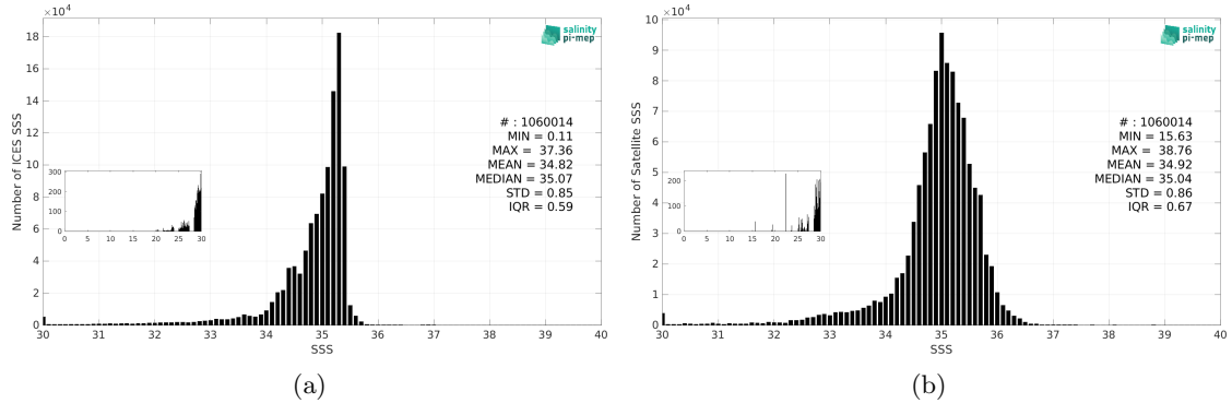
Figure 2: Histograms of SSS from ICES (a) and SMOS SSS L3 v9 - 9 Days (CATDS-CEC-LOCEAN) (b) considering all match-up pairs per bins of 0.1 over the Atlantic Ocean Pi-MEP region and for the full satellite product period.
