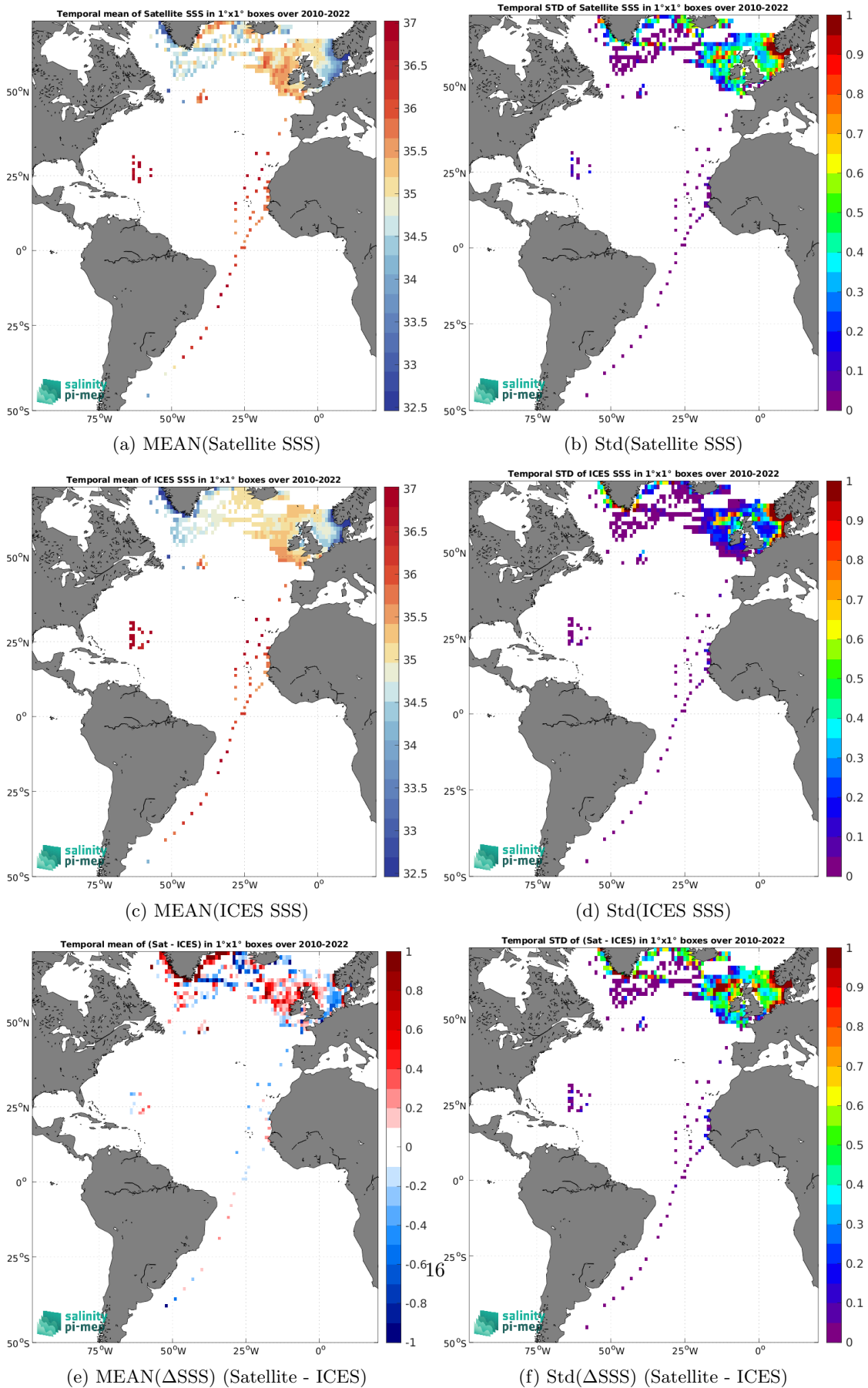
Figure 6: Temporal mean (left) and Std (right) of SSS from SMOS SSS L3 v9 - 9 Days (CATDS-CEC-LOCEAN) (top), ICES (middle), and of \Delta SSS (Satellite - ICES). Only match-up pairs are used to generate these maps.
