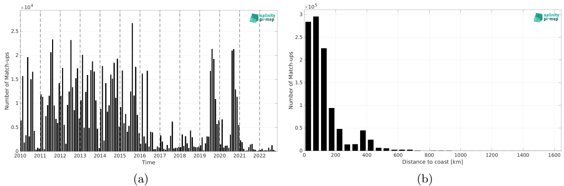
Figure 1: Number of match-ups between ICES and SMOS SSS L3 v9 - 9 Days (CATDS-CEC-LOCEAN) SSS as a function of time (a) and as function of the distance to coast (b) over the Atlantic Ocean Pi-MEP region and for the full satellite product period.
