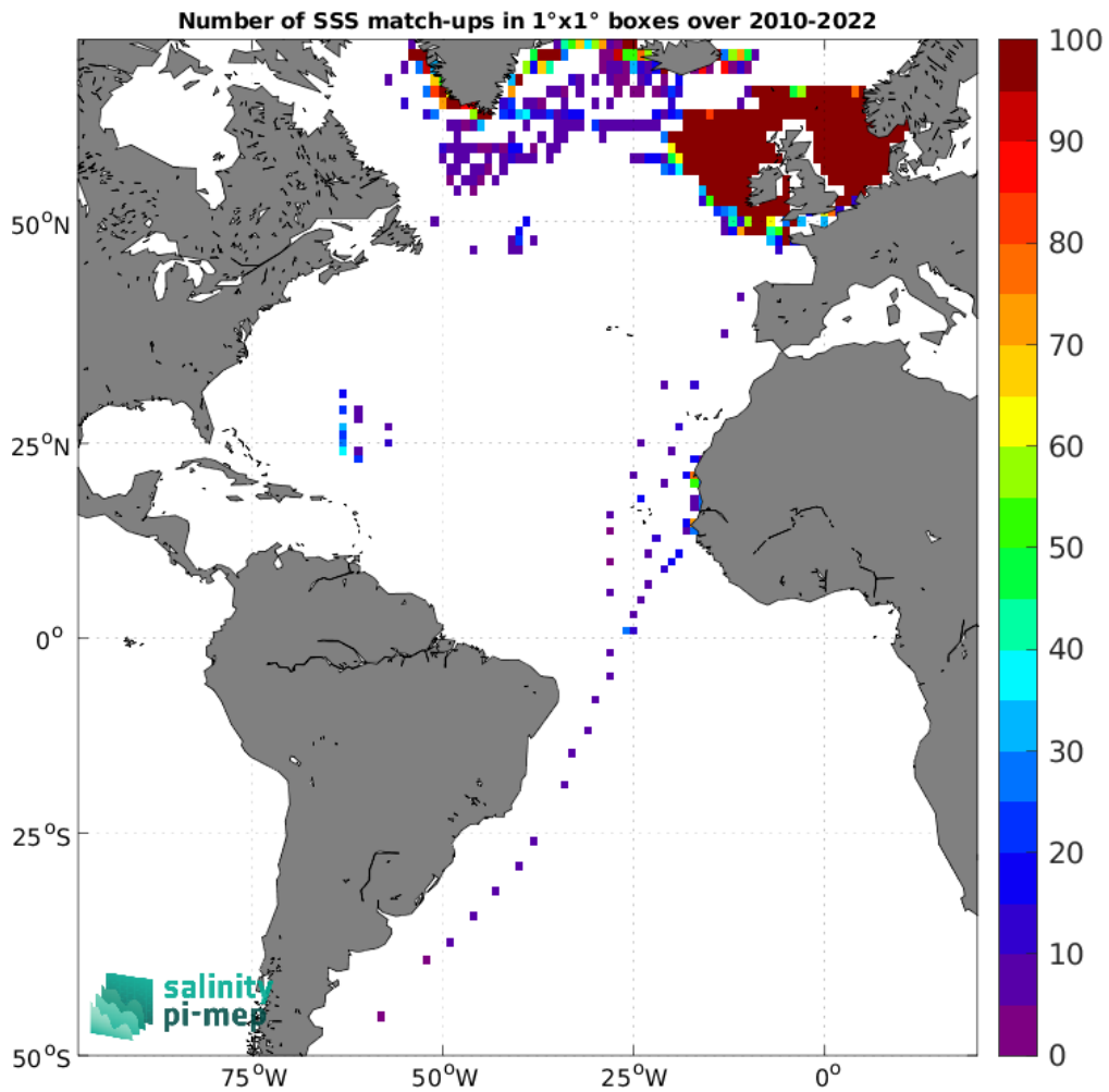
Figure 4: Number of SSS match-ups between ICES SSS and the SMOS SSS L3 v9 - 9 Days (CATDS-CEC-LOCEAN) SSS product for the Atlantic Ocean Pi-MEP region over 1^\circ \times 1^\circ boxes and for the full satellite product period.
