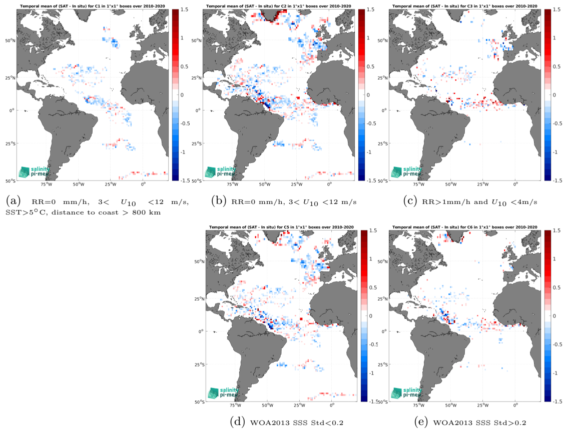
Figure 13: Temporal mean gridded over spatial boxes of size 1^\circ \times 1^\circ of \Delta\text{SSS} (SMOS SSS L3 v9 - 9 Days (CATDS-CEC-LOCEAN) - Surface drifters) for 5 different subdatasets corresponding to:RR=0 mm/h, 3 < U_{10} < 12 m/s, SST >5^\circ\text{C} , distance to coast > 800 km (a), RR=0 mm/h, 3 < U_{10} < 12 m/s (b), RR >1 mm/h and U_{10} < 4 m/s (c), WOA2013 SSS Std <0.2 (d), WOA2013 SSS Std >0.2 (e).
