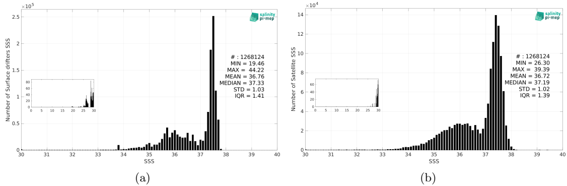
Figure 3: Histograms of SSS from Surface drifters (a) and SMOS SSS L3 v9 - 9 Days (CATDS-CEC-LOCEAN) (b) considering all match-up pairs per bins of 0.1 over the Atlantic Ocean Pi-MEP region and for the full satellite product period.
