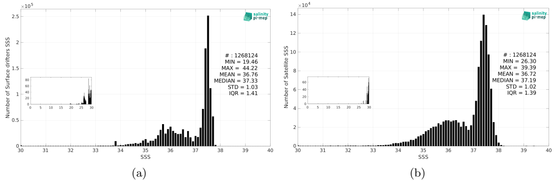
Figure 2: Histograms of SSS from Surface drifters (a) and SMOS SSS L3 v9 - 9 Days (CATDS-CEC-LOCEAN) (b) considering all match-up pairs per bins of 0.1 over the Atlantic Ocean Pi-MEP region and for the full satellite product period.
