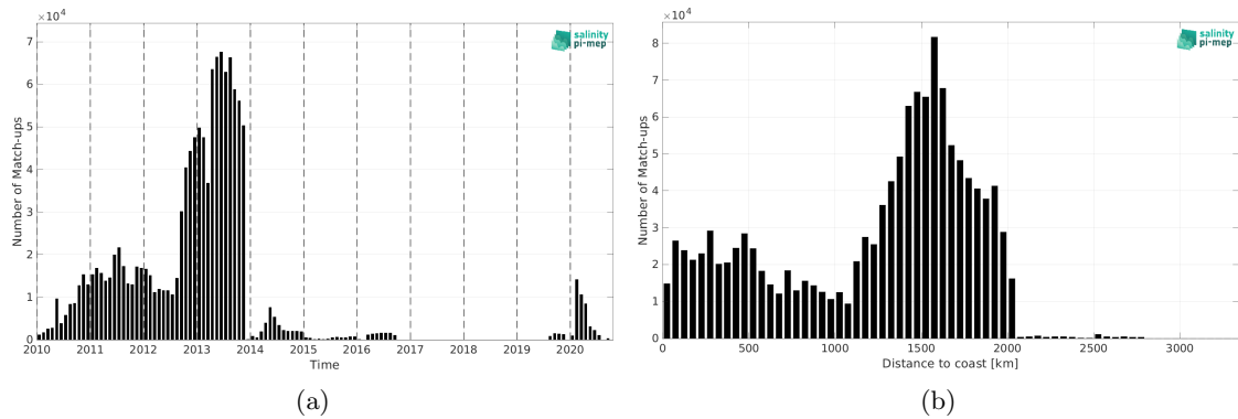
Figure 1: Number of match-ups between Surface drifters and SMOS SSS L3 v9 - 9 Days (CATDS-CEC-LOCEAN) SSS as a function of time (a) and as function of the distance to coast (b) over the Atlantic Ocean Pi-MEP region and for the full satellite product period.
