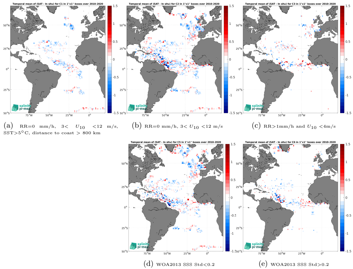
Figure 11: Temporal mean gridded over spatial boxes of size 1^\circ \times 1^\circ of \Delta SSS (SMOS SSS L3 v9 - 9 Days (CATDS-CEC-LOCEAN) - Surface drifters) for 5 different subdatasets corresponding to:RR=0 mm/h, 3 < U_{10} < 12 m/s, SST >5^\circ\text{C} , distance to coast > 800 km (a), RR=0 mm/h, 3 < U_{10} < 12 m/s (b), RR >1 mm/h and U_{10} < 4 m/s (c), WOA2013 SSS Std <0.2 (d), WOA2013 SSS Std >0.2 (e).
