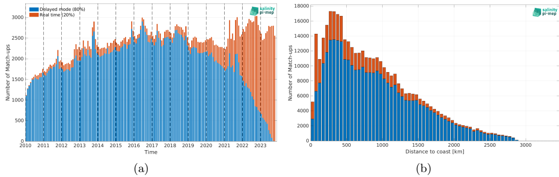
Figure 1: Number of match-ups between Argo and SMOS SSS L3 v9 - 9 Days (CATDS-CEC-LOCEAN) SSS as a function of time (a) and as function of the distance to coast (b) over the Atlantic Ocean Pi-MEP region and for the full satellite product period.
