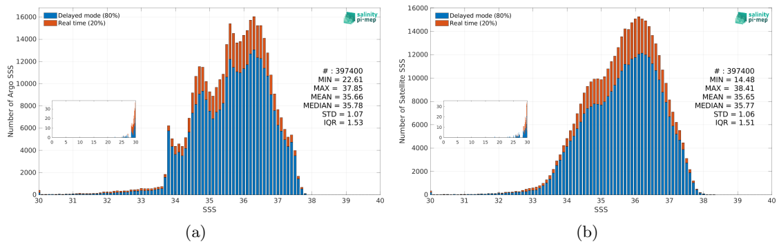
Figure 2: Histograms of SSS from Argo (a) and SMOS SSS L3 v9 - 9 Days (CATDS-CEC-LOCEAN) (b) considering all match-up pairs per bins of 0.1 over the Atlantic Ocean Pi-MEP region and for the full satellite product period.
