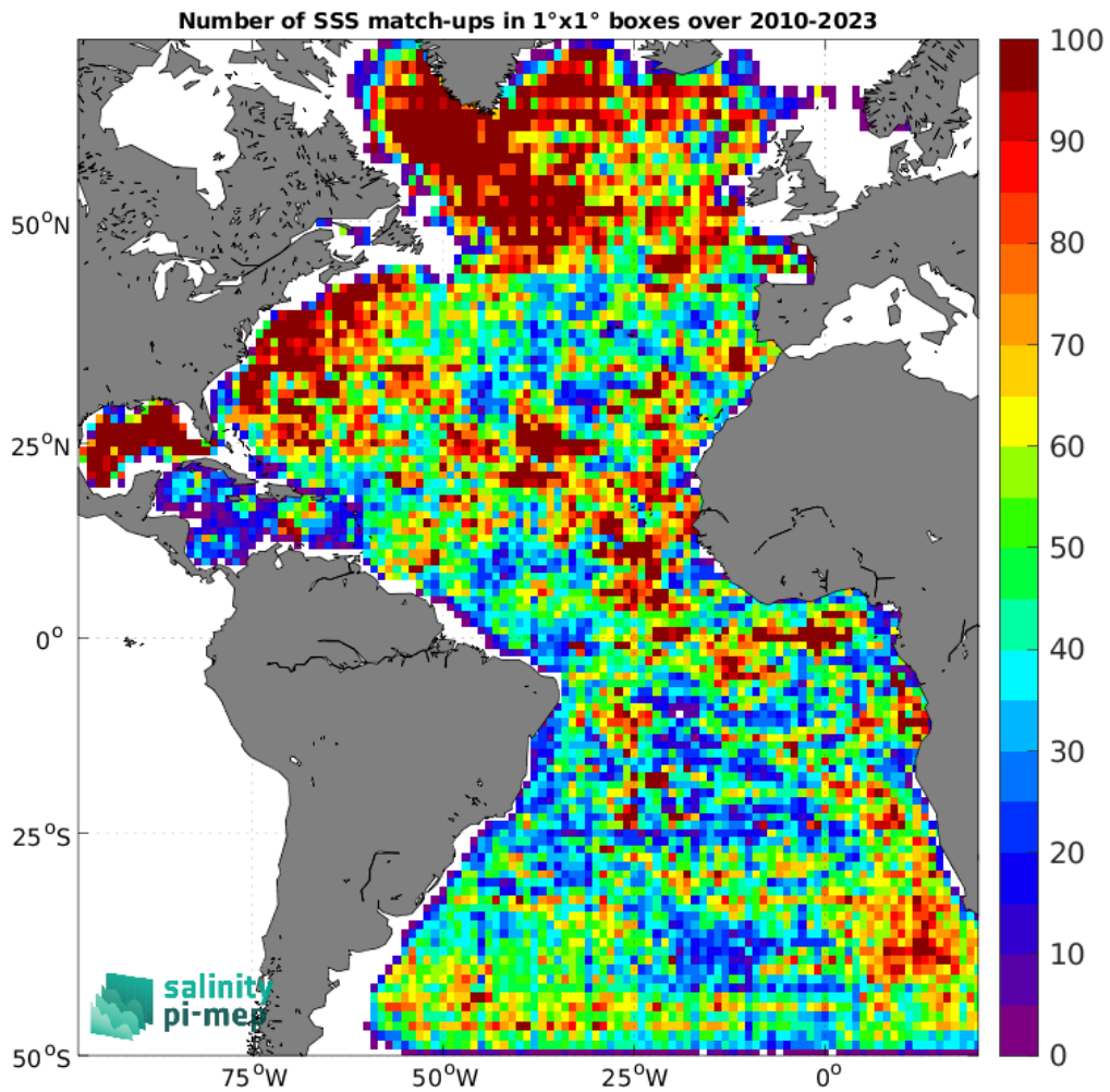
Figure 4: Number of SSS match-ups between Argo SSS and the SMOS SSS L3 v9 - 9 Days (CATDS-CEC-LOCEAN) SSS product for the Atlantic Ocean Pi-MEP region over 1^\circ \times 1^\circ boxes and for the full satellite product period.
