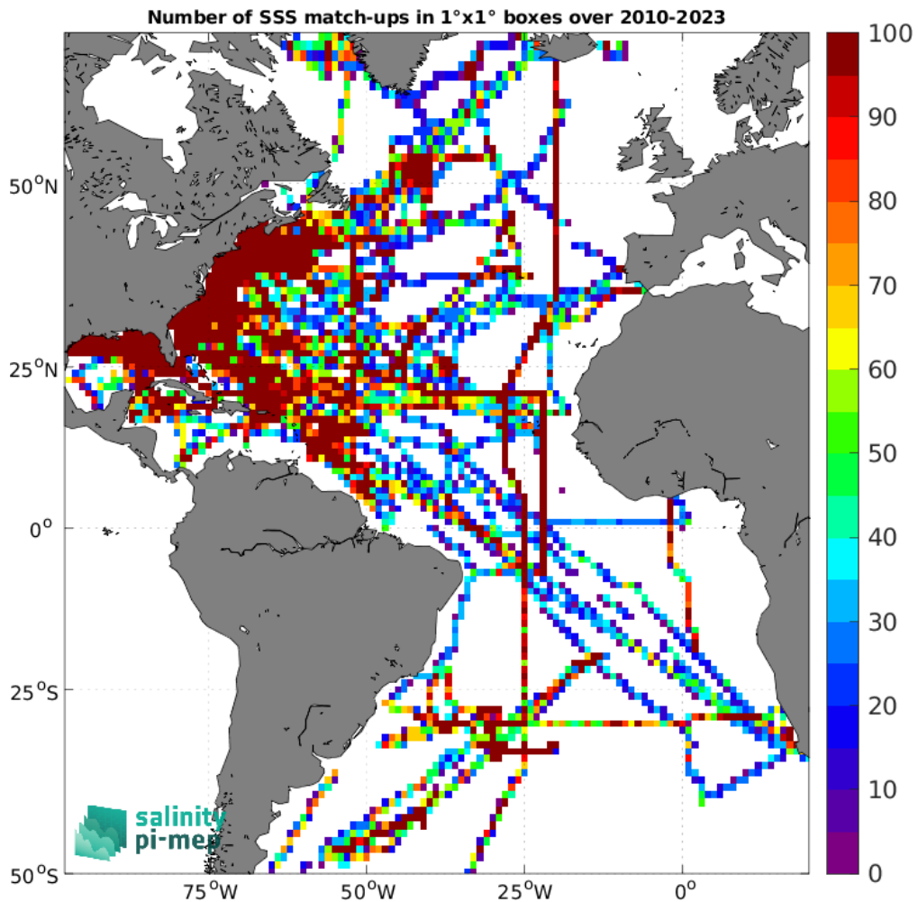
Figure 5: Number of SSS match-ups between TSG (SAMOS) SSS and the SMOS SSS L3 v9 - 18 Days (CATDS-CEC-LOCEAN) SSS product for the Atlantic Ocean Pi-MEP region over 1^\circ \times 1^\circ boxes and for the full satellite product period.
