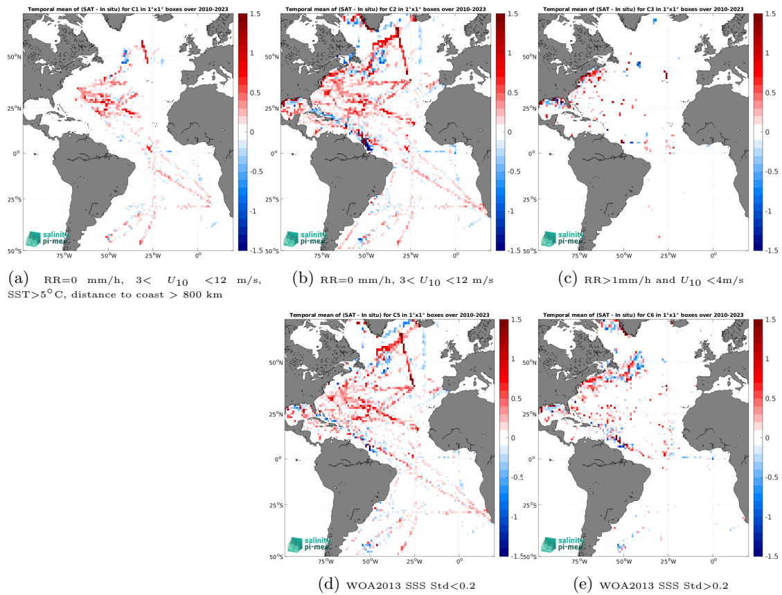
Figure 14: Temporal mean gridded over spatial boxes of size 1^\circ \times 1^\circ of \Delta\text{SSS} (SMOS SSS L3 v9 - 18 Days (CATDS-CEC-LOCEAN) - TSG (SAMOS)) for 5 different subdatasets corresponding to:RR=0 mm/h, 3 < U_{10} < 12 m/s, SST>5°C, distance to coast > 800 km (a), RR=0 mm/h, 3 < U_{10} < 12 m/s (b), RR>1mm/h and U_{10} < 4 m/s (c), WOA2013 SSS Std<0.2 (d), WOA2013 SSS Std>0.2 (e).
