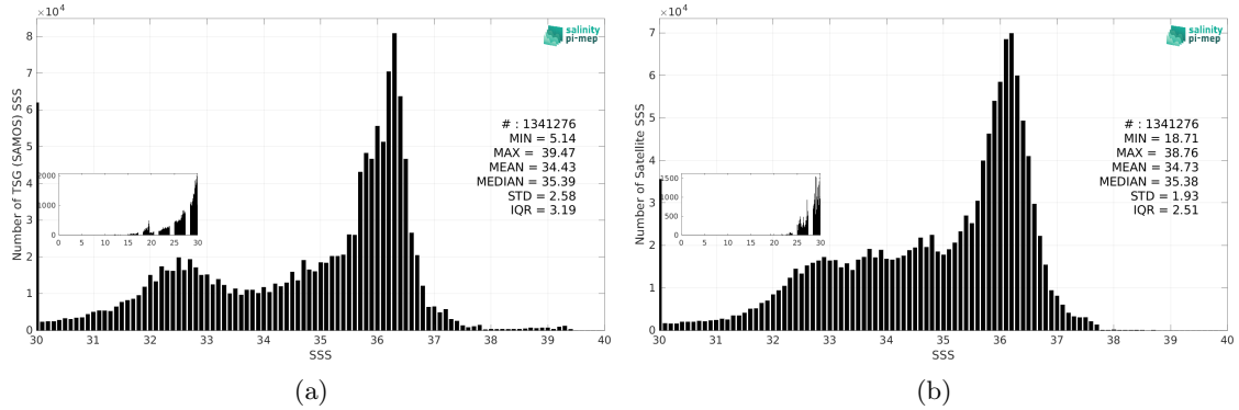
Figure 3: Histograms of SSS from TSG (SAMOS) (a) and SMOS SSS L3 v9 - 18 Days (CATDS-CEC-LOCEAN) (b) considering all match-up pairs per bins of 0.1 over the Atlantic Ocean Pi-MEP region and for the full satellite product period.
