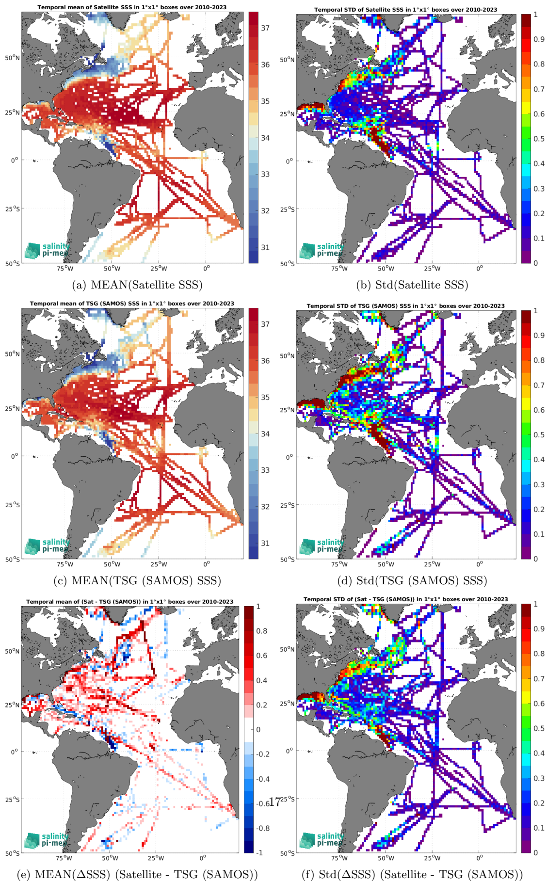
Figure 7: Temporal mean (left) and Std (right) of SSS from SMOS SSS L3 v9 - 18 Days (CATDS-CEC-LOCEAN) (top), TSG (SAMOS) (middle), and of \Delta SSS (Satellite - TSG (SAMOS)). Only match-up pairs are used to generate these maps.
