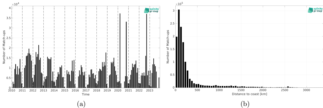
Figure 2: Number of match-ups between TSG (SAMOS) and SMOS SSS L3 v9 - 18 Days (CATDS-CEC-LOCEAN) SSS as a function of time (a) and as function of the distance to coast (b) over the Atlantic Ocean Pi-MEP region and for the full satellite product period.
