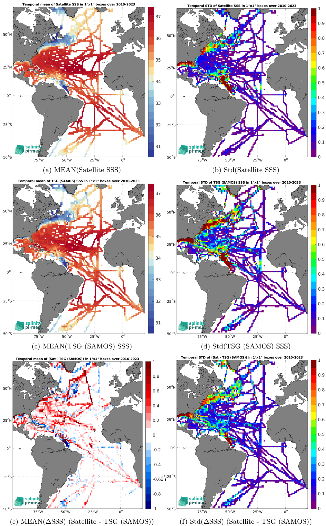
Figure 6: Temporal mean (left) and Std (right) of SSS from SMOS SSS L3 v9 - 18 Days (CATDS-CEC-LOCEAN) (top), TSG (SAMOS) (middle), and of \Delta SSS (Satellite - TSG (SAMOS)). Only match-up pairs are used to generate these maps.
