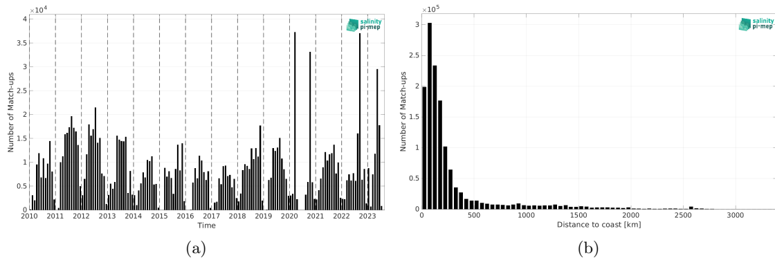
Figure 1: Number of match-ups between TSG (SAMOS) and SMOS SSS L3 v9 - 18 Days (CATDS-CEC-LOCEAN) SSS as a function of time (a) and as function of the distance to coast (b) over the Atlantic Ocean Pi-MEP region and for the full satellite product period.
