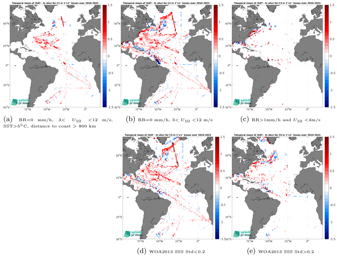
Figure 12: Temporal mean gridded over spatial boxes of size 1^\circ \times 1^\circ of \Delta\text{SSS} (SMOS SSS L3 v9 - 18 Days (CATDS-CEC-LOCEAN) - TSG (SAMOS)) for 5 different subdatasets corresponding to:RR=0 mm/h, 3 < U_{10} < 12 m/s, SST >5^\circ\text{C} , distance to coast > 800 km (a), RR=0 mm/h, 3 < U_{10} < 12 m/s (b), RR >1 mm/h and U_{10} < 4 m/s (c), WOA2013 SSS Std <0.2 (d), WOA2013 SSS Std >0.2 (e).
