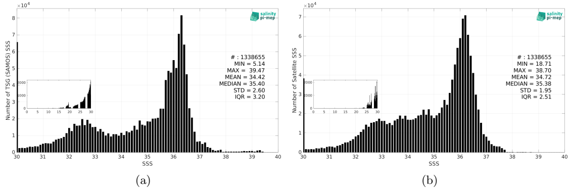
Figure 2: Histograms of SSS from TSG (SAMOS) (a) and SMOS SSS L3 v9 - 18 Days (CATDS-CEC-LOCEAN) (b) considering all match-up pairs per bins of 0.1 over the Atlantic Ocean Pi-MEP region and for the full satellite product period.
