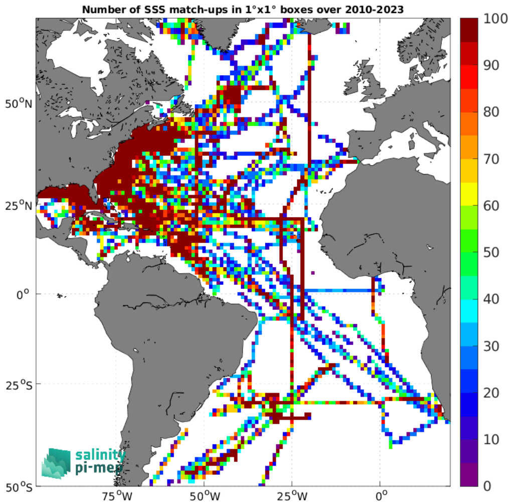
Figure 4: Number of SSS match-ups between TSG (SAMOS) SSS and the SMOS SSS L3 v9 - 18 Days (CATDS-CEC-LOCEAN) SSS product for the Atlantic Ocean Pi-MEP region over 1°x1° boxes and for the full satellite product period.
