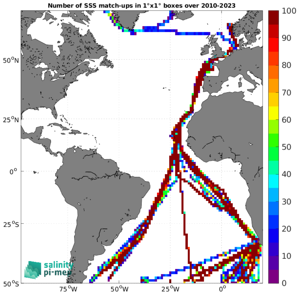
Figure 5: Number of SSS match-ups between TSG (Polarstern) SSS and the SMOS SSS L3 v9 - 18 Days (CATDS-CEC-LOCEAN) SSS product for the Atlantic Ocean Pi-MEP region over 1°×1° boxes and for the full satellite product period.
