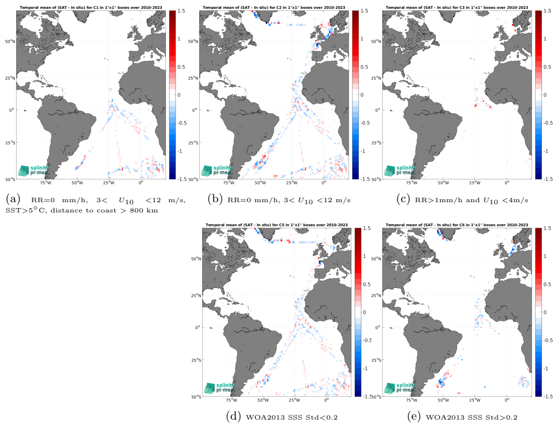
Figure 14: Temporal mean gridded over spatial boxes of size 1^\circ \times 1^\circ of \Delta SSS (SMOS SSS L3 v9 - 18 Days (CATDS-CEC-LOCEAN) - TSG (Polarstern)) for 5 different subdatasets corresponding to:RR=0 mm/h, 3 < U_{10} < 12 m/s, SST >5^\circ\text{C} , distance to coast > 800 km (a), RR=0 mm/h, 3 < U_{10} < 12 m/s (b), RR >1 mm/h and U_{10} < 4 m/s (c), WOA2013 SSS Std <0.2 (d), WOA2013 SSS Std >0.2 (e).
