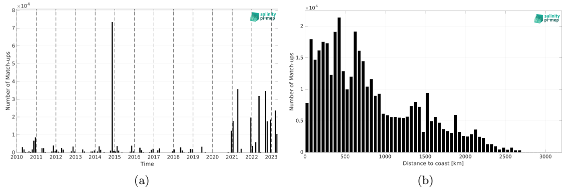
Figure 2: Number of match-ups between TSG (Polarstern) and SMOS SSS L3 v9 - 18 Days (CATDS-CEC-LOCEAN) SSS as a function of time (a) and as function of the distance to coast (b) over the Atlantic Ocean Pi-MEP region and for the full satellite product period.
