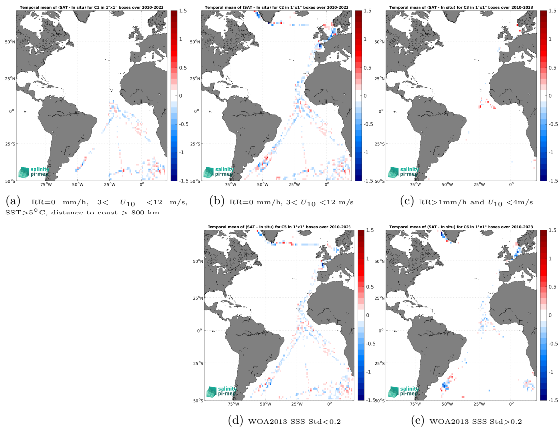
Figure 14: Temporal mean gridded over spatial boxes of size 1^\circ \times 1^\circ of \Delta\text{SSS} (SMOS SSS L3 v9 - 18 Days (CATDS-CEC-LOCEAN) - TSG (Polarstern)) for 5 different subdatasets corresponding to:RR=0 mm/h, 3 < U_{10} < 12 m/s, SST>5°C, distance to coast > 800 km (a), RR=0 mm/h, 3 < U_{10} < 12 m/s (b), RR>1mm/h and U_{10} < 4 m/s (c), WOA2013 SSS Std<0.2 (d), WOA2013 SSS Std>0.2 (e).
