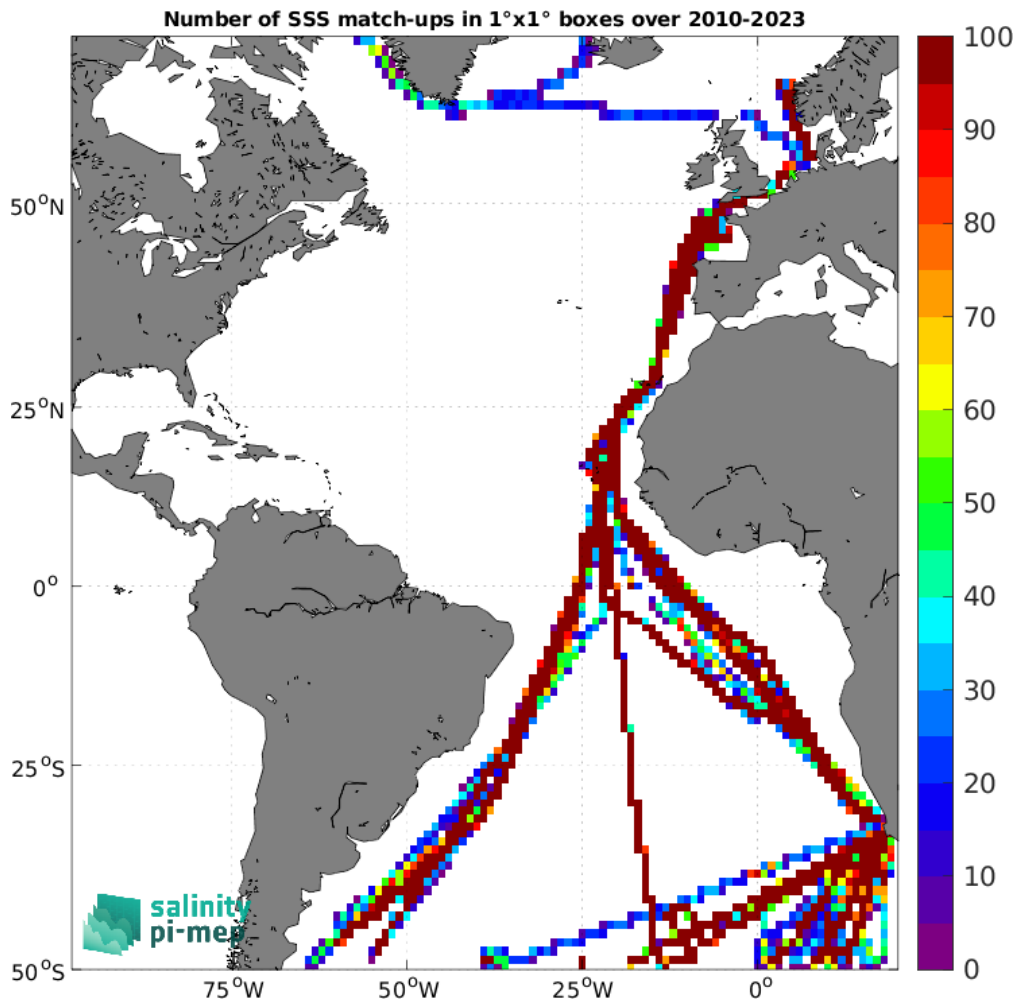
Figure 5: Number of SSS match-ups between TSG (Polarstern) SSS and the SMOS SSS L3 v9 - 18 Days (CATDS-CEC-LOCEAN) SSS product for the Atlantic Ocean Pi-MEP region over 1^\circ \times 1^\circ boxes and for the full satellite product period.
