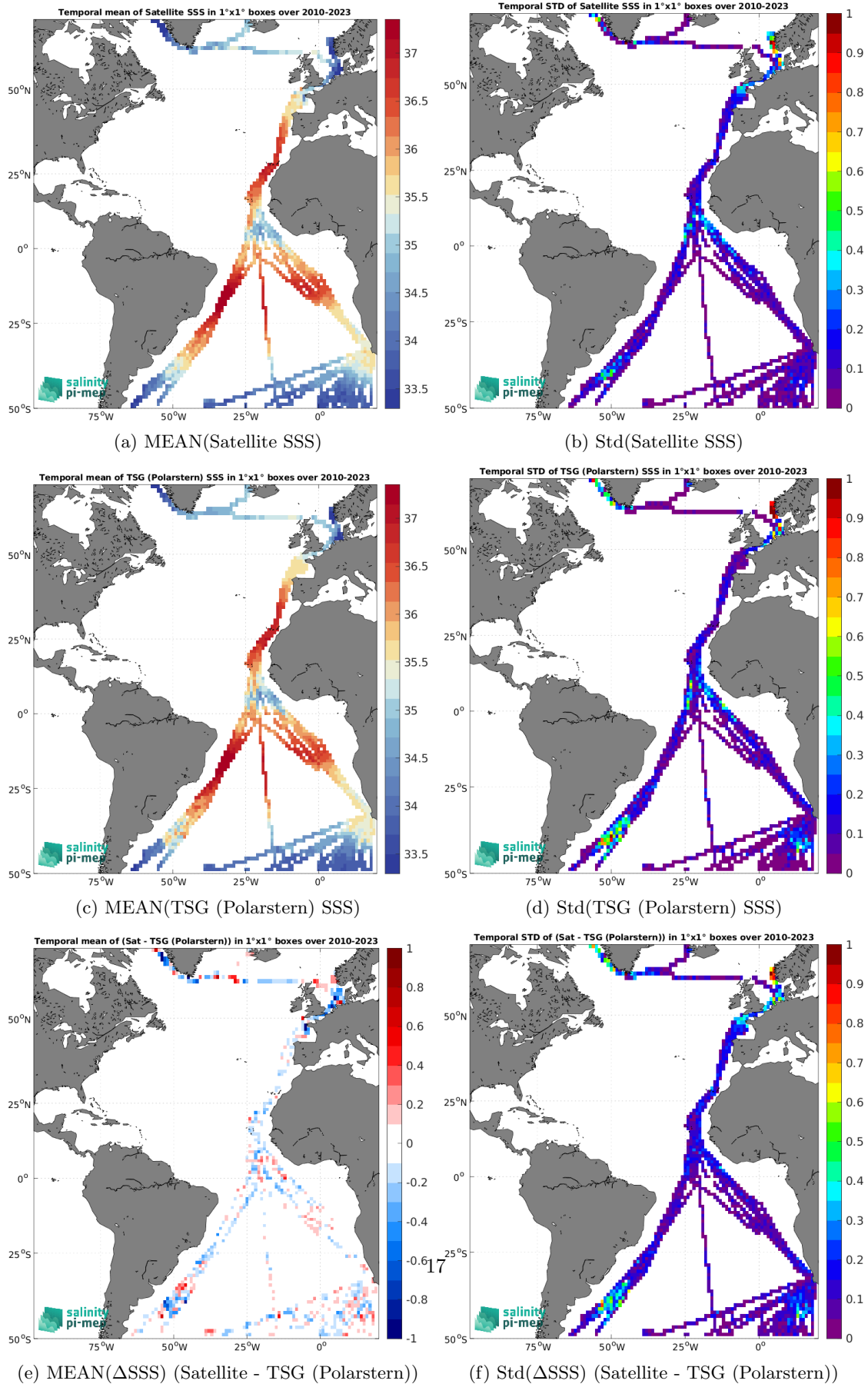
Figure 7: Temporal mean (left) and Std (right) of SSS from SMOS SSS L3 v9 - 18 Days (CATDS-CEC-LOCEAN) (top), TSG (Polarstern) (middle), and of \Delta SSS (Satellite - TSG (Polarstern)). Only match-up pairs are used to generate these maps.
