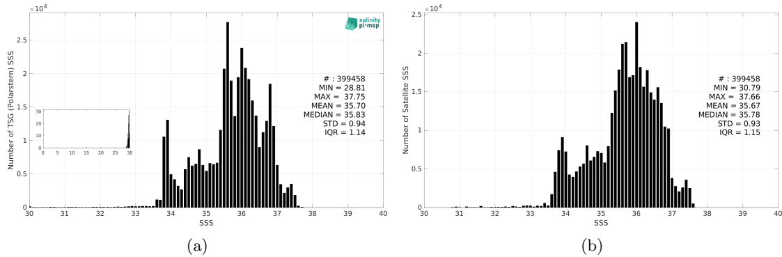
Figure 3: Histograms of SSS from TSG (Polarstern) (a) and SMOS SSS L3 v9 - 18 Days (CATDS-CEC-LOCEAN) (b) considering all match-up pairs per bins of 0.1 over the Atlantic Ocean Pi-MEP region and for the full satellite product period.
