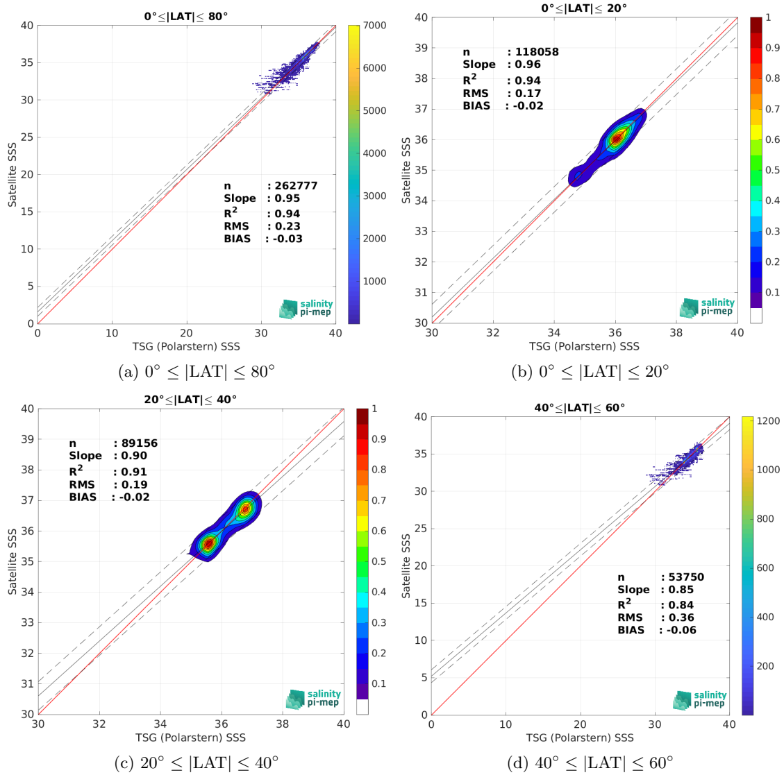
Figure 9: Contour maps of the concentration of SMOS SSS L3 v9 - 18 Days (CATDS-CEC-LOCEAN) SSS (y-axis) versus TSG (Polarstern) SSS (x-axis) at match-up pairs for different latitude bands. For each plot, the red line shows x=y . The black thin and dashed lines indicate a linear fit through the data cloud and the \pm 95\% confidence levels, respectively. The number match-up pairs n , the slope and R^2 coefficient of the linear fit, the root mean square (RMS) and the mean bias between satellite and in situ data are indicated for each latitude band in each plots.
