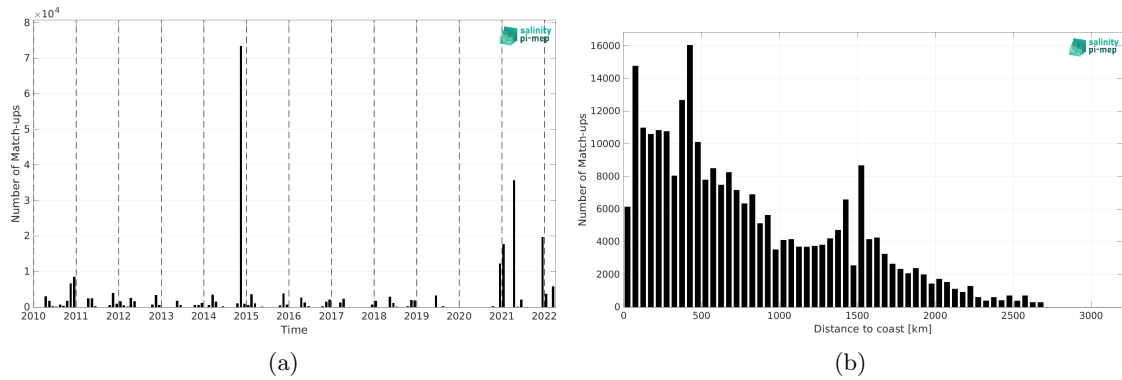
Figure 1: Number of match-ups between TSG (Polarstern) and SMOS SSS L3 v9 - 18 Days (CATDS-CEC-LOCEAN) SSS as a function of time (a) and as function of the distance to coast (b) over the Atlantic Ocean Pi-MEP region and for the full satellite product period.
