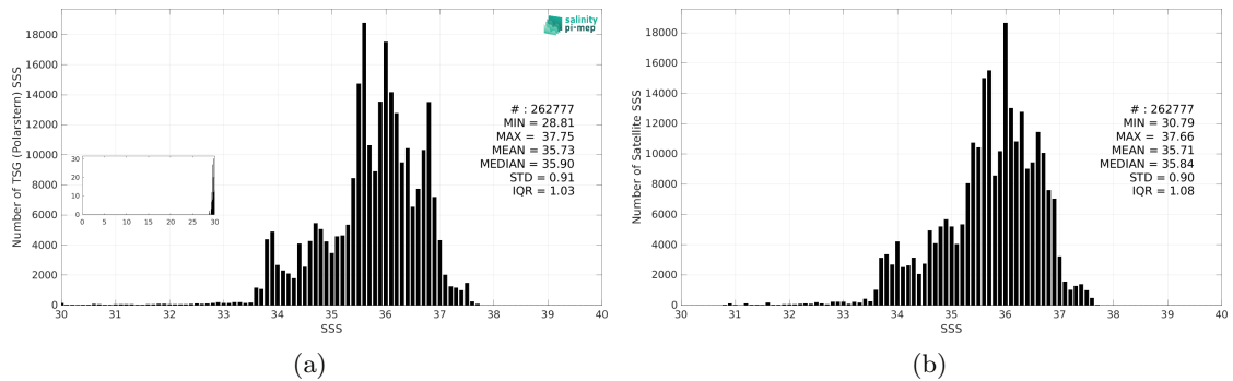
Figure 2: Histograms of SSS from TSG (Polarstern) (a) and SMOS SSS L3 v9 - 18 Days (CATDS-CEC-LOCEAN) (b) considering all match-up pairs per bins of 0.1 over the Atlantic Ocean Pi-MEP region and for the full satellite product period.
