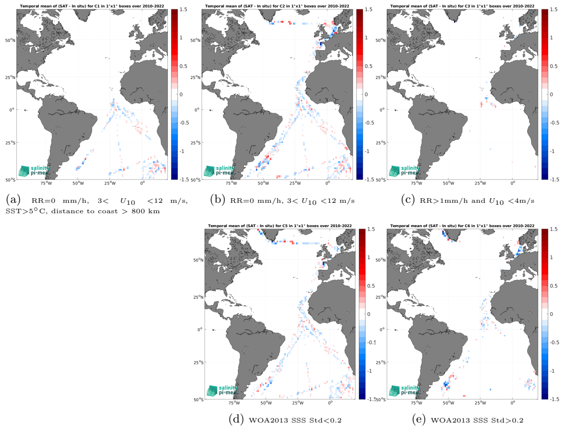
Figure 12: Temporal mean gridded over spatial boxes of size 1^\circ \times 1^\circ of \Delta SSS (SMOS SSS L3 v9 - 18 Days (CATDS-CEC-LOCEAN) - TSG (Polarstern)) for 5 different subdatasets corresponding to:RR=0 mm/h, 3 < U_{10} < 12 m/s, SST >5^\circ\text{C} , distance to coast > 800 km (a), RR=0 mm/h, 3 < U_{10} < 12 m/s (b), RR >1 mm/h and U_{10} < 4 m/s (c), WOA2013 SSS Std <0.2 (d), WOA2013 SSS Std >0.2 (e).
