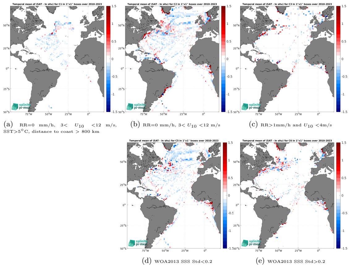
Figure 14: Temporal mean gridded over spatial boxes of size 1^\circ \times 1^\circ of \Delta\text{SSS} (SMOS SSS L3 v9 - 18 Days (CATDS-CEC-LOCEAN) - TSG (LEGOS-DM)) for 5 different subdatasets corresponding to:RR=0 mm/h, 3 < U_{10} < 12 m/s, SST>5°C, distance to coast > 800 km (a), RR=0 mm/h, 3 < U_{10} < 12 m/s (b), RR>1mm/h and U_{10} < 4 m/s (c), WOA2013 SSS Std<0.2 (d), WOA2013 SSS Std>0.2 (e).
