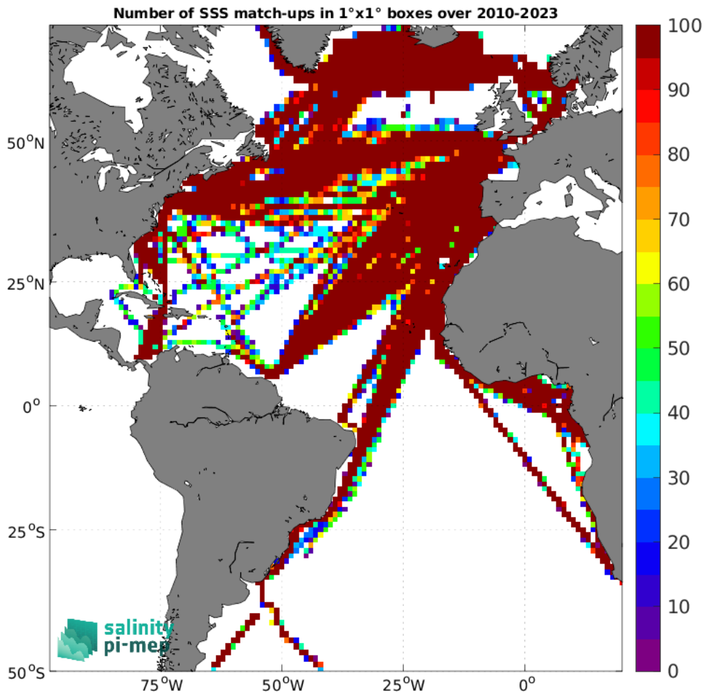
Figure 5: Number of SSS match-ups between TSG (LEGOS-DM) SSS and the SMOS SSS L3 v9 - 18 Days (CATDS-CEC-LOCEAN) SSS product for the Atlantic Ocean Pi-MEP region over 1^\circ \times 1^\circ boxes and for the full satellite product period.
