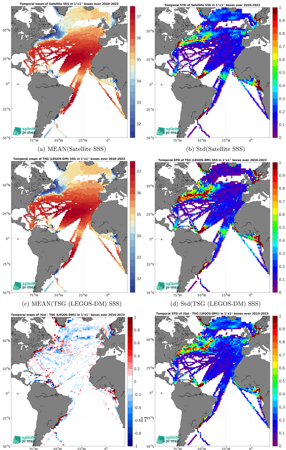
(e) MEAN( \Delta SSS) (Satellite - TSG (LEGOS-DM)) (f) Std( \Delta SSS) (Satellite - TSG (LEGOS-DM)) Figure 7: Temporal mean (left) and Std (right) of SSS from SMOS SSS L3 v9 - 18 Days (CATDS-CEC-LOCEAN) (top), TSG (LEGOS-DM) (middle), and of \Delta SSS (Satellite - TSG (LEGOS-DM)). Only match-up pairs are used to generate these maps.
