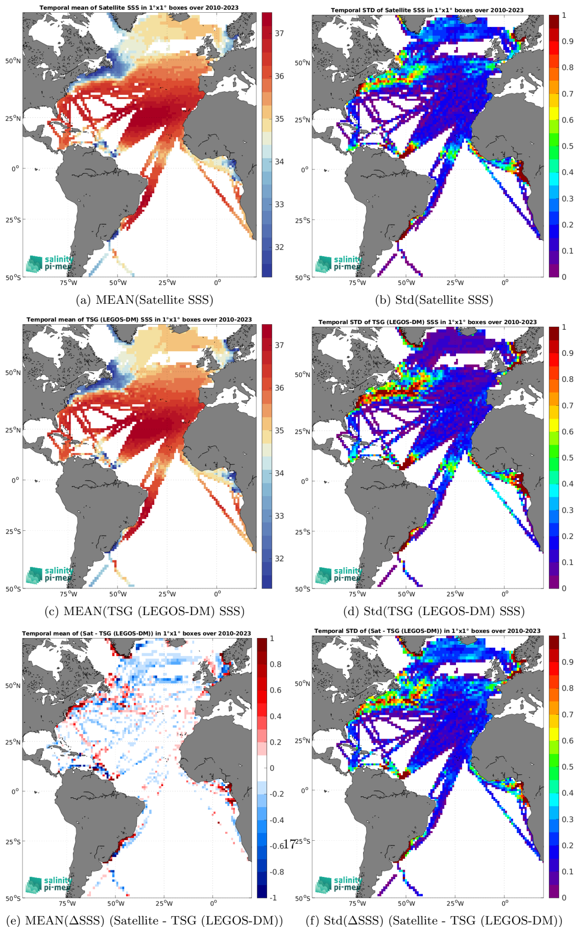
Figure 6: Temporal mean (left) and Std (right) of SSS from SMOS SSS L3 v9 - 18 Days (CATDS-CEC-LOCEAN) (top), TSG (LEGOS-DM) (middle), and of \Delta SSS (Satellite - TSG (LEGOS-DM)). Only match-up pairs are used to generate these maps.
