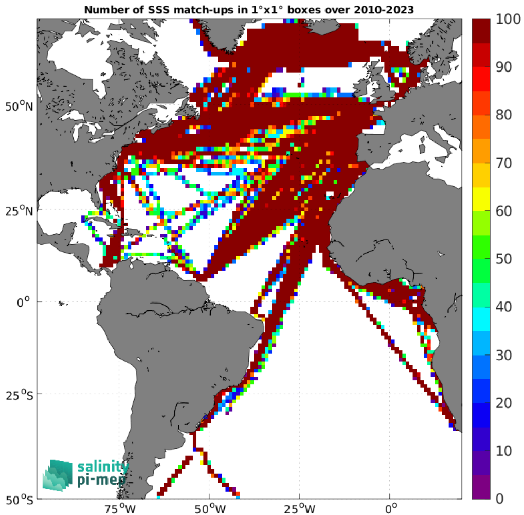
Figure 4: Number of SSS match-ups between TSG (LEGOS-DM) SSS and the SMOS SSS L3 v9 - 18 Days (CATDS-CEC-LOCEAN) SSS product for the Atlantic Ocean Pi-MEP region over 1° × 1° boxes and for the full satellite product period.
