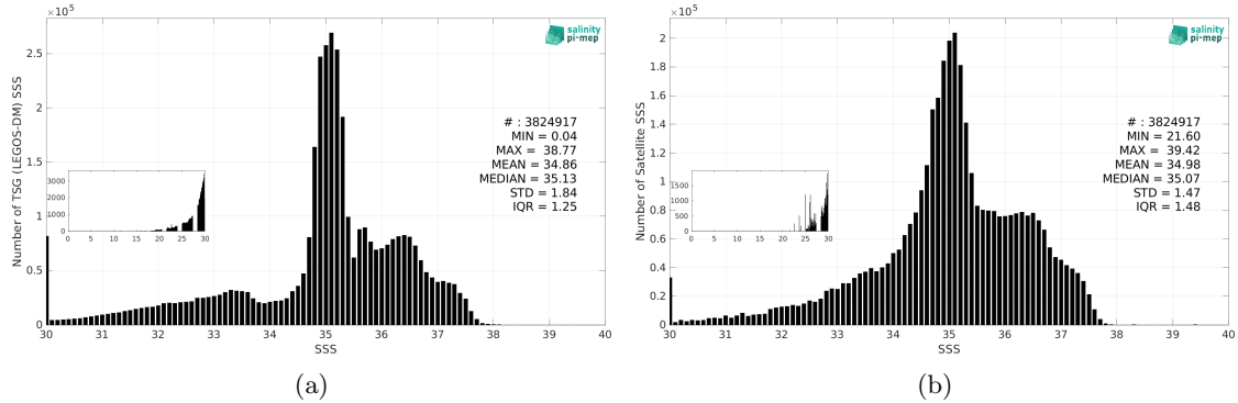
Figure 2: Histograms of SSS from TSG (LEGOS-DM) (a) and SMOS SSS L3 v9 - 18 Days (CATDS-CEC-LOCEAN) (b) considering all match-up pairs per bins of 0.1 over the Atlantic Ocean Pi-MEP region and for the full satellite product period.
