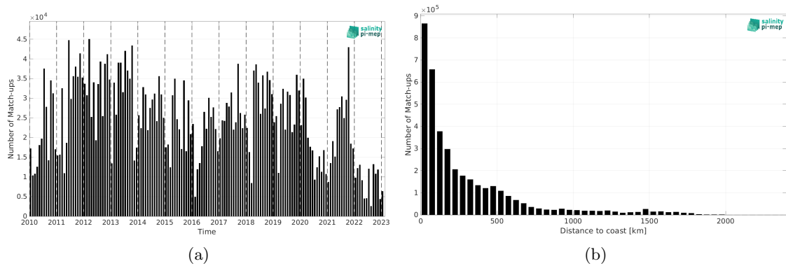
Figure 1: Number of match-ups between TSG (LEGOS-DM) and SMOS SSS L3 v9 - 18 Days (CATDS-CEC-LOCEAN) SSS as a function of time (a) and as function of the distance to coast (b) over the Atlantic Ocean Pi-MEP region and for the full satellite product period.
