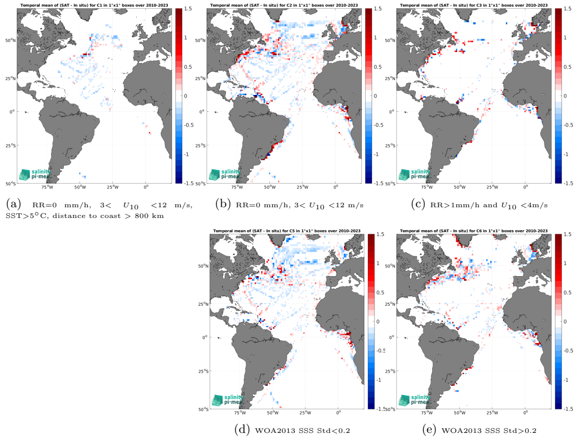
Figure 12: Temporal mean gridded over spatial boxes of size 1^\circ \times 1^\circ of \Delta SSS (SMOS SSS L3 v9 - 18 Days (CATDS-CEC-LOCEAN) - TSG (LEGOS-DM)) for 5 different subdatasets corresponding to:RR=0 mm/h, 3 < U_{10} < 12 m/s, SST >5^\circ\text{C} , distance to coast > 800 km (a), RR=0 mm/h, 3 < U_{10} < 12 m/s (b), RR >1 mm/h and U_{10} < 4 m/s (c), WOA2013 SSS Std <0.2 (d), WOA2013 SSS Std >0.2 (e).
