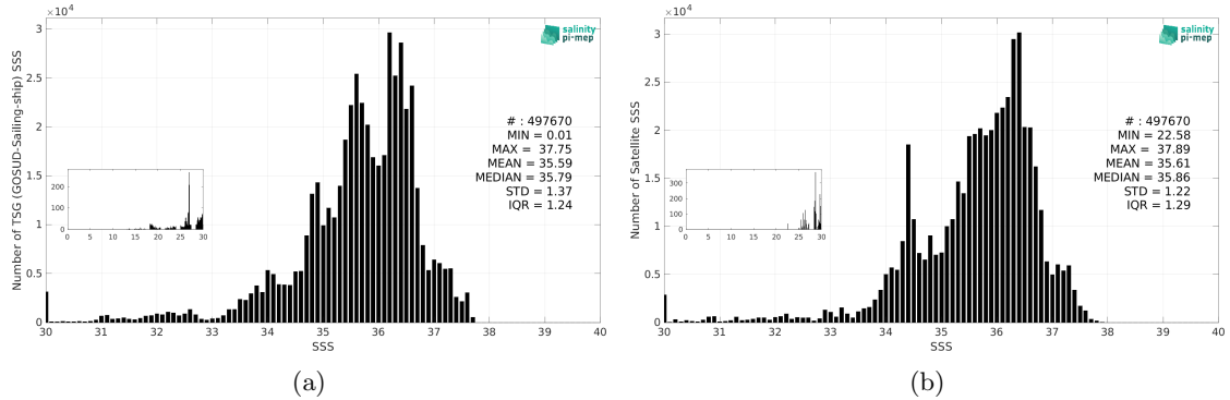
Figure 2: Histograms of SSS from TSG (GOSUD-Sailing-ship) (a) and SMOS SSS L3 v9 - 18 Days (CATDS-CEC-LOCEAN) (b) considering all match-up pairs per bins of 0.1 over the Atlantic Ocean Pi-MEP region and for the full satellite product period.
