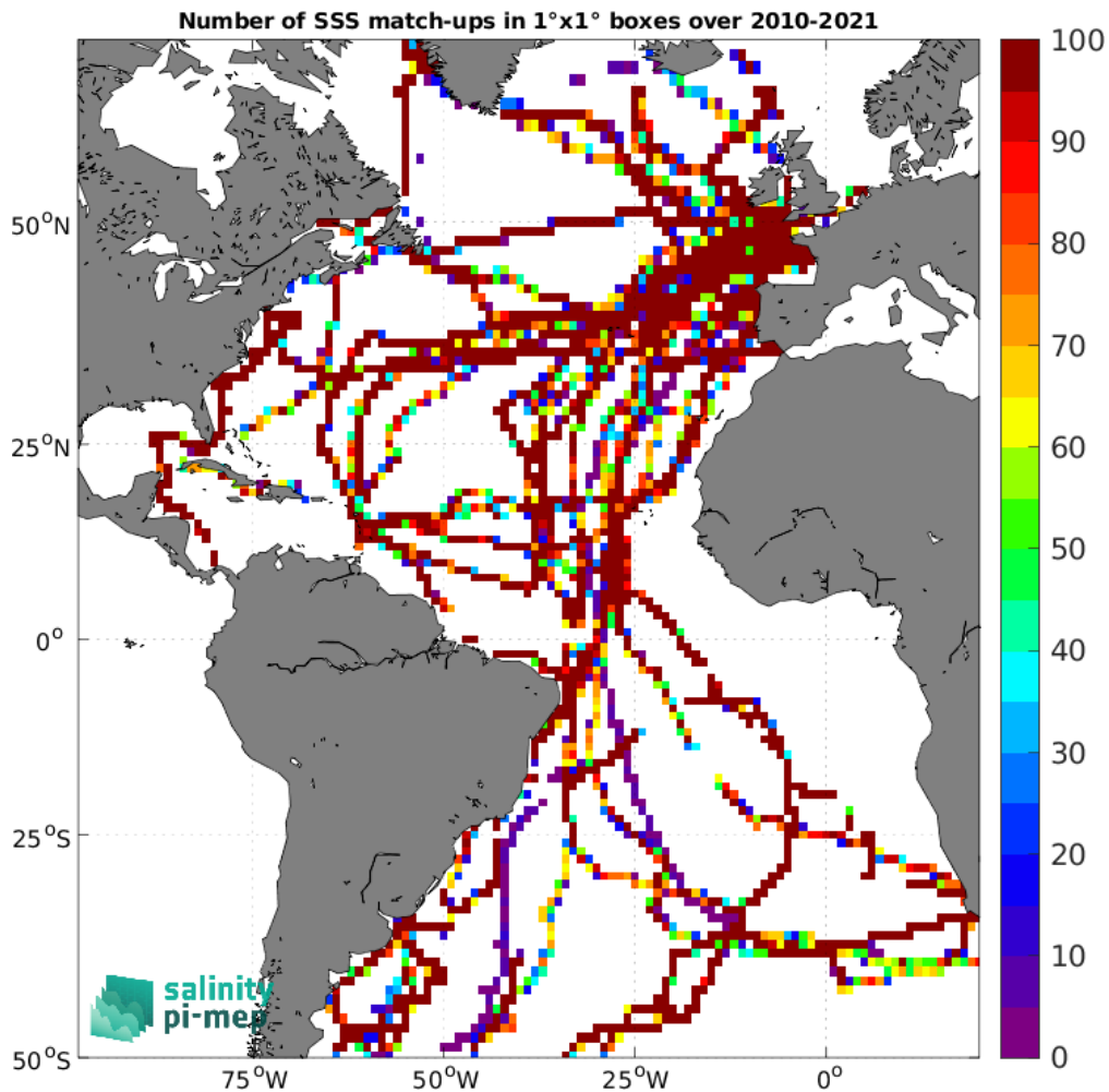
Figure 4: Number of SSS match-ups between TSG (GOSUD-Sailing-ship) SSS and the SMOS SSS L3 v9 - 18 Days (CATDS-CEC-LOCEAN) SSS product for the Atlantic Ocean Pi-MEP region over 1^\circ \times 1^\circ boxes and for the full satellite product period.
