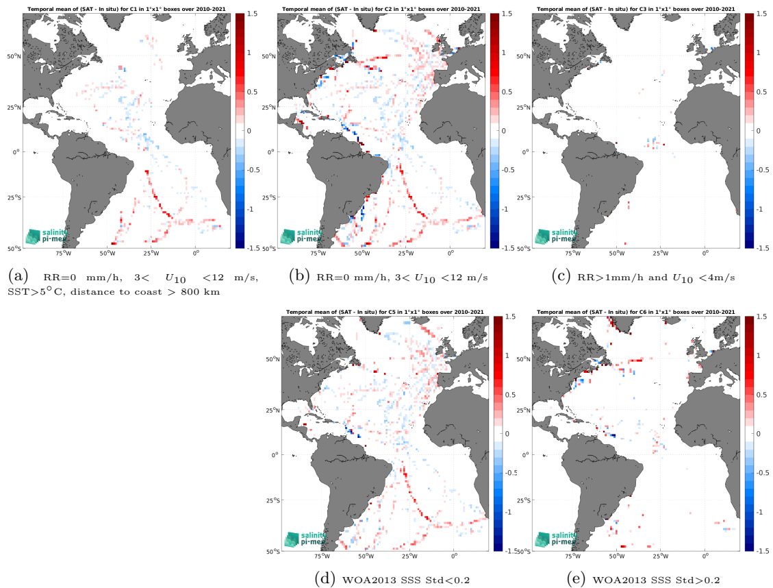
Figure 12: Temporal mean gridded over spatial boxes of size 1^\circ \times 1^\circ of \Delta\text{SSS} (SMOS SSS L3 v9 - 18 Days (CATDS-CEC-LOCEAN) - TSG (GOSUD-Sailing-ship)) for 5 different subdatasets corresponding to:RR=0 mm/h, 3 < U_{10} < 12 m/s, SST>5°C, distance to coast > 800 km (a), RR=0 mm/h, 3 < U_{10} < 12 m/s (b), RR>1mm/h and U_{10} < 4 m/s (c), WOA2013 SSS Std<0.2 (d), WOA2013 SSS Std>0.2 (e).
