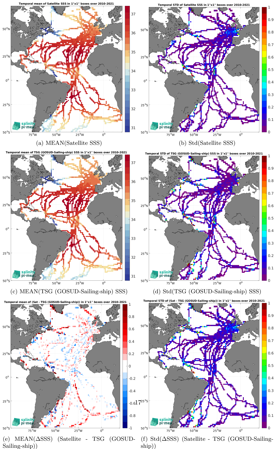
Figure 6: Temporal mean (left) and Std (right) of SSS from SMOS SSS L3 v9 - 18 Days (CATDS-CEC-LOCEAN) (top), TSG (GOSUD-Sailing-ship) (middle), and of \Delta SSS (Satellite - TSG (GOSUD-Sailing-ship)). Only match-up pairs are used to generate these maps.
