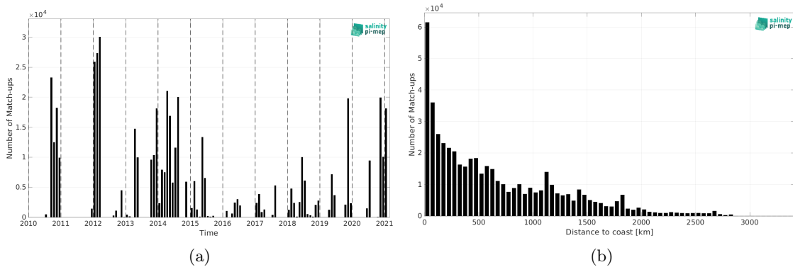
Figure 1: Number of match-ups between TSG (GOSUD-Sailing-ship) and SMOS SSS L3 v9 - 18 Days (CATDS-CEC-LOCEAN) SSS as a function of time (a) and as function of the distance to coast (b) over the Atlantic Ocean Pi-MEP region and for the full satellite product period.
