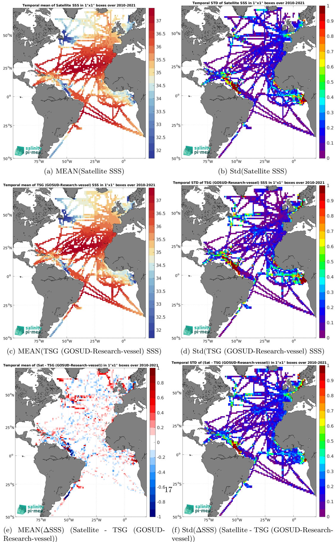
Figure 6: Temporal mean (left) and Std (right) of SSS from SMOS SSS L3 v9 - 18 Days (CATDS-CEC-LOCEAN) (top), TSG (GOSUD-Research-vessel) (middle), and of \Delta SSS (Satellite - TSG (GOSUD-Research-vessel)). Only match-up pairs are used to generate these maps.
