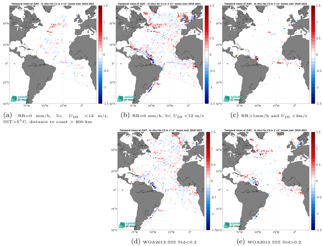
Figure 12: Temporal mean gridded over spatial boxes of size 1^\circ \times 1^\circ of \Delta\text{SSS} (SMOS SSS L3 v9 - 18 Days (CATDS-CEC-LOCEAN) - TSG (GOSUD-Research-vessel)) for 5 different subdatasets corresponding to:RR=0 mm/h, 3 < U_{10} < 12 m/s, SST>5°C, distance to coast > 800 km (a), RR=0 mm/h, 3 < U_{10} < 12 m/s (b), RR>1mm/h and U_{10} < 4 m/s (c), WOA2013 SSS Std<0.2 (d), WOA2013 SSS Std>0.2 (e).
