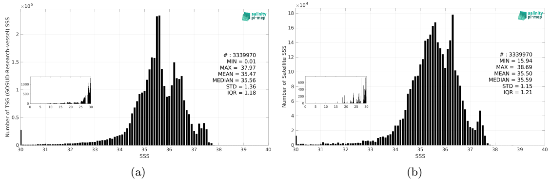
Figure 2: Histograms of SSS from TSG (GOSUD-Research-vessel) (a) and SMOS SSS L3 v9 - 18 Days (CATDS-CEC-LOCEAN) (b) considering all match-up pairs per bins of 0.1 over the Atlantic Ocean Pi-MEP region and for the full satellite product period.
