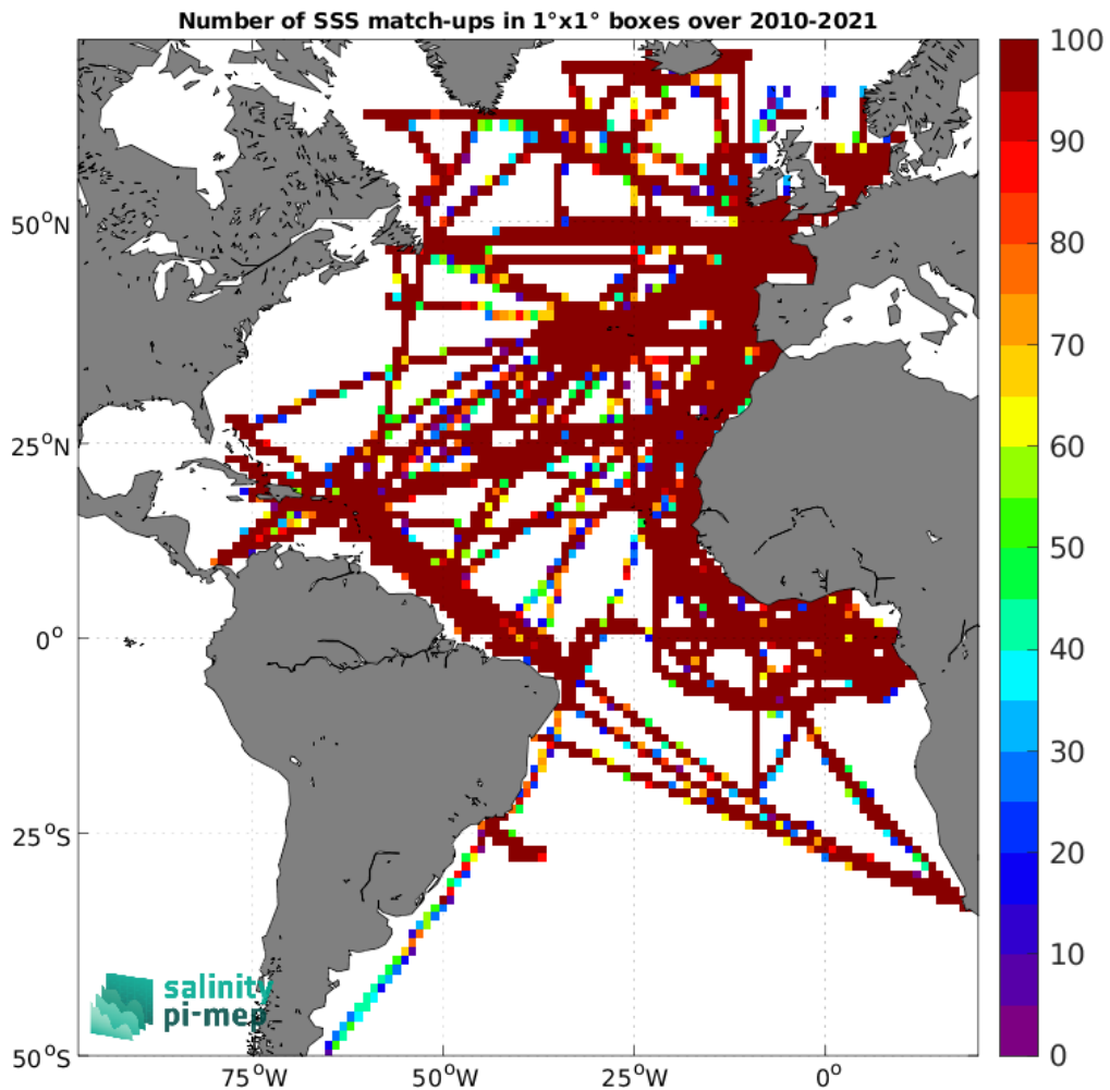
Figure 4: Number of SSS match-ups between TSG (GOSUD-Research-vessel) SSS and the SMOS SSS L3 v9 - 18 Days (CATDS-CEC-LOCEAN) SSS product for the Atlantic Ocean Pi-MEP region over 1^\circ \times 1^\circ boxes and for the full satellite product period.
