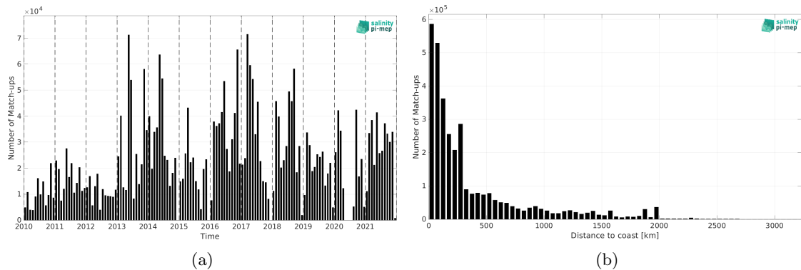
Figure 1: Number of match-ups between TSG (GOSUD-Research-vessel) and SMOS SSS L3 v9 - 18 Days (CATDS-CEC-LOCEAN) SSS as a function of time (a) and as function of the distance to coast (b) over the Atlantic Ocean Pi-MEP region and for the full satellite product period.
