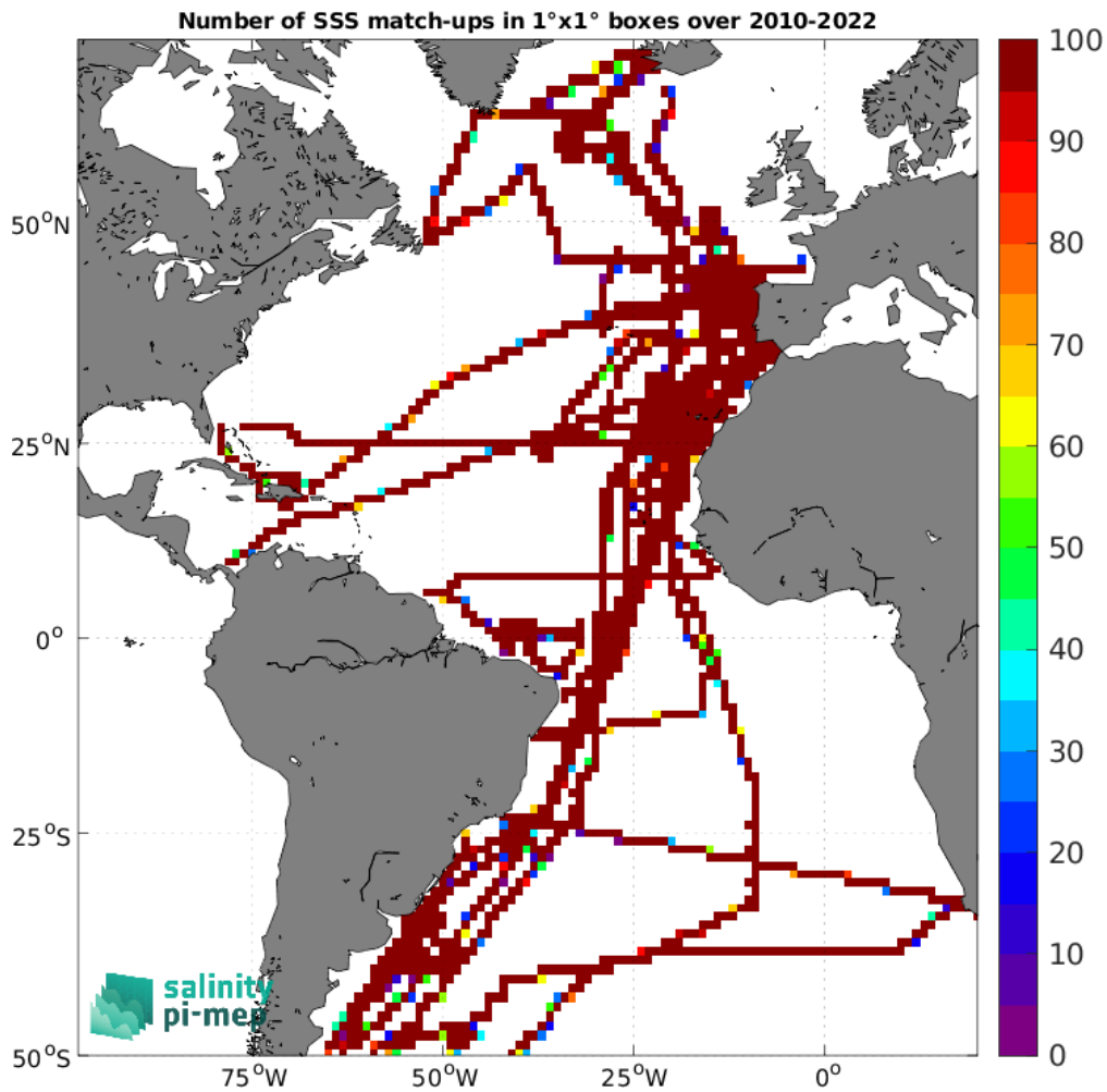
Figure 4: Number of SSS match-ups between TSG (CSIC-UTM) SSS and the SMOS SSS L3 v9 - 18 Days (CATDS-CEC-LOCEAN) SSS product for the Atlantic Ocean Pi-MEP region over 1^\circ \times 1^\circ boxes and for the full satellite product period.
