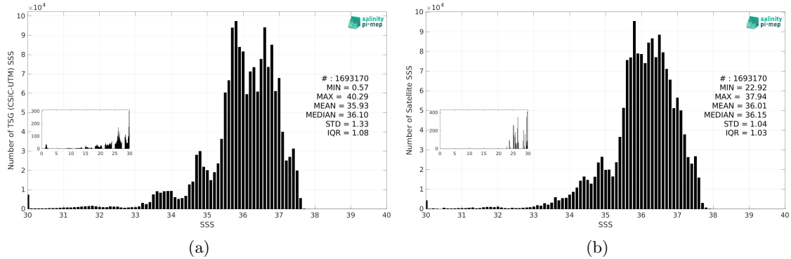
Figure 2: Histograms of SSS from TSG (CSIC-UTM) (a) and SMOS SSS L3 v9 - 18 Days (CATDS-CEC-LOCEAN) (b) considering all match-up pairs per bins of 0.1 over the Atlantic Ocean Pi-MEP region and for the full satellite product period.
