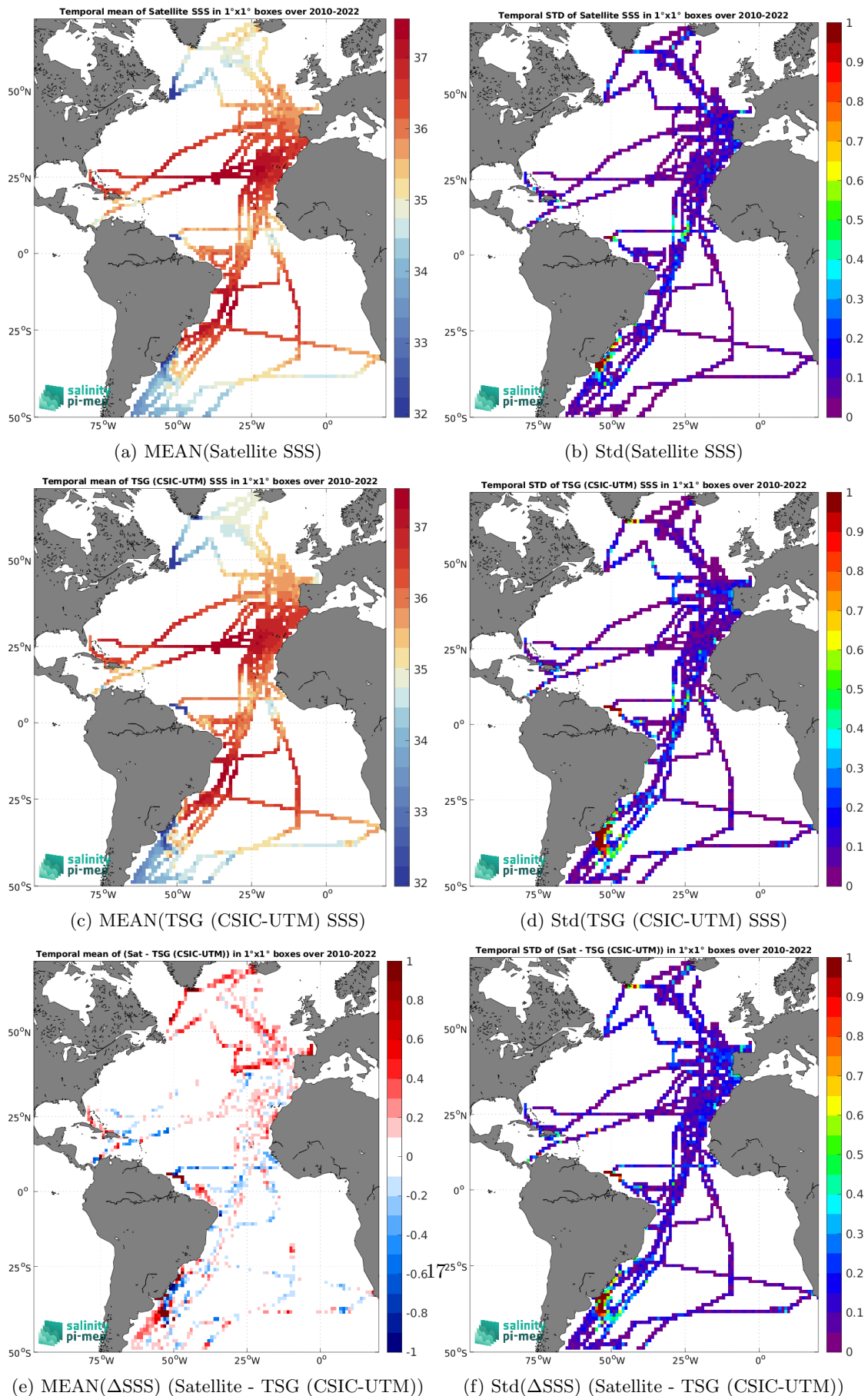
Figure 6: Temporal mean (left) and Std (right) of SSS from SMOS SSS L3 v9 - 18 Days (CATDS-CEC-LOCEAN) (top), TSG (CSIC-UTM) (middle), and of \Delta SSS (Satellite - TSG (CSIC-UTM)). Only match-up pairs are used to generate these maps.
