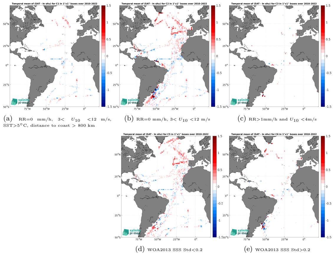
Figure 12: Temporal mean gridded over spatial boxes of size 1^\circ \times 1^\circ of \Delta SSS (SMOS SSS L3 v9 - 18 Days (CATDS-CEC-LOCEAN) - TSG (CSIC-UTM)) for 5 different subdatasets corresponding to:RR=0 mm/h, 3 < U_{10} < 12 m/s, SST >5^\circ\text{C} , distance to coast > 800 km (a), RR=0 mm/h, 3 < U_{10} < 12 m/s (b), RR >1 mm/h and U_{10} < 4 m/s (c), WOA2013 SSS Std <0.2 (d), WOA2013 SSS Std >0.2 (e).
