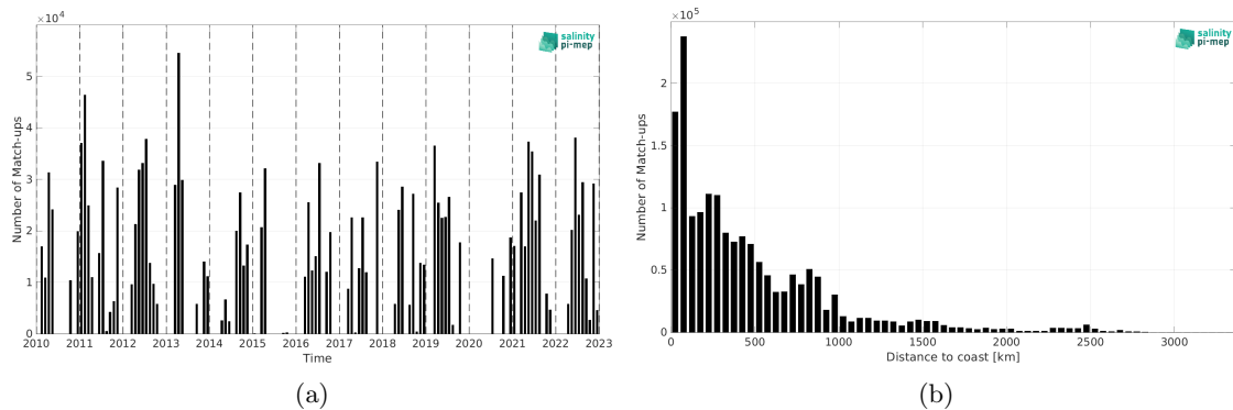
Figure 1: Number of match-ups between TSG (CSIC-UTM) and SMOS SSS L3 v9 - 18 Days (CATDS-CEC-LOCEAN) SSS as a function of time (a) and as function of the distance to coast (b) over the Atlantic Ocean Pi-MEP region and for the full satellite product period.
