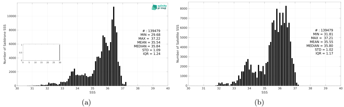
Figure 3: Histograms of SSS from Sairdrone (a) and SMOS SSS L3 v9 - 18 Days (CATDS-CEC-LOCEAN) (b) considering all match-up pairs per bins of 0.1 over the Atlantic Ocean Pi-MEP region and for the full satellite product period.
