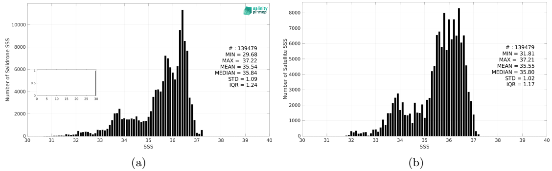
Figure 2: Histograms of SSS from Sairdrone (a) and SMOS SSS L3 v9 - 18 Days (CATDS-CEC-LOCEAN) (b) considering all match-up pairs per bins of 0.1 over the Atlantic Ocean Pi-MEP region and for the full satellite product period.
