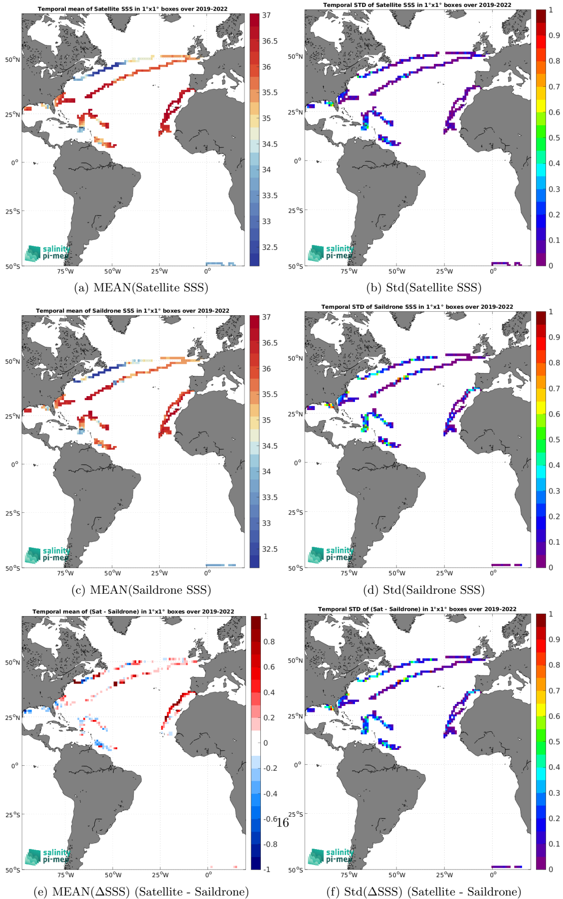
Figure 6: Temporal mean (left) and Std (right) of SSS from SMOS SSS L3 v9 - 18 Days (CATDS-CEC-LOCEAN) (top), Saildrone (middle), and of \Delta SSS (Satellite - Saildrone). Only match-up pairs are used to generate these maps.
