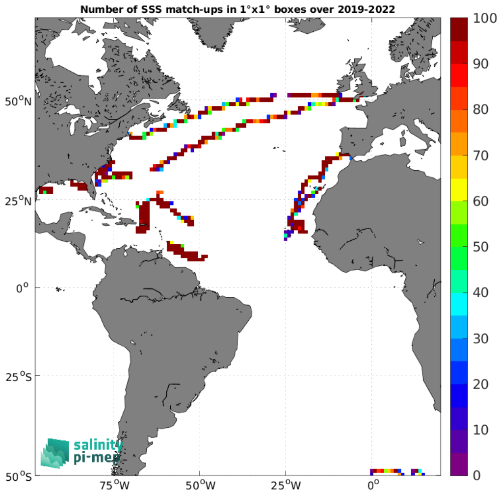
Figure 4: Number of SSS match-ups between Saildrone SSS and the SMOS SSS L3 v9 - 18 Days (CATDS-CEC-LOCEAN) SSS product for the Atlantic Ocean Pi-MEP region over 1^\circ \times 1^\circ boxes and for the full satellite product period.
