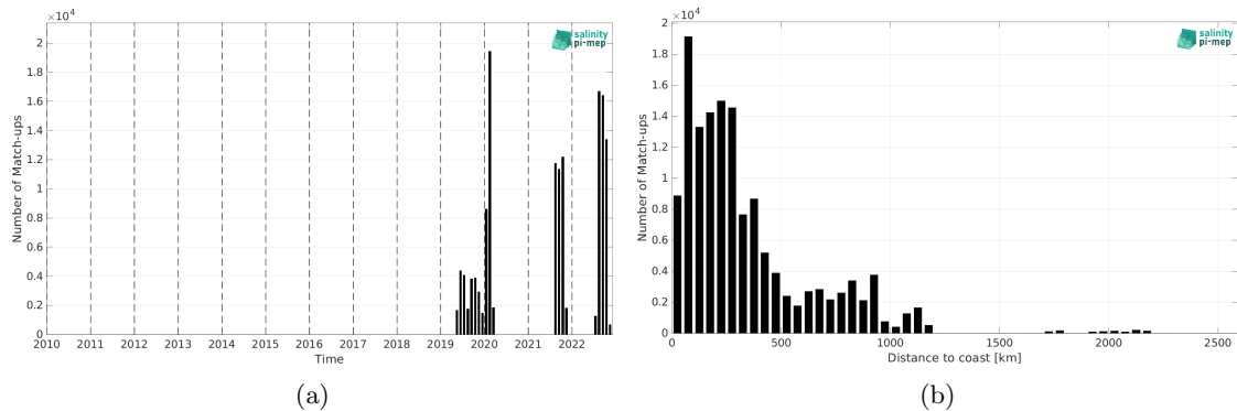
Figure 1: Number of match-ups between Saildrone and SMOS SSS L3 v9 - 18 Days (CATDS-CEC-LOCEAN) SSS as a function of time (a) and as function of the distance to coast (b) over the Atlantic Ocean Pi-MEP region and for the full satellite product period.
