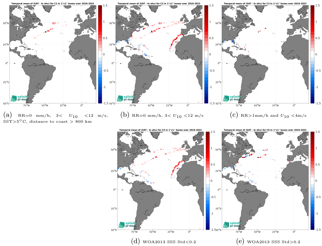
Figure 12: Temporal mean gridded over spatial boxes of size 1^\circ \times 1^\circ of \Delta\text{SSS} (SMOS SSS L3 v9 - 18 Days (CATDS-CEC-LOCEAN) - Sailydrone) for 5 different subdatasets corresponding to:RR=0 mm/h, 3 < U_{10} < 12 m/s, SST >5^\circ\text{C} , distance to coast > 800 km (a), RR=0 mm/h, 3 < U_{10} < 12 m/s (b), RR >1 mm/h and U_{10} < 4 m/s (c), WOA2013 SSS Std <0.2 (d), WOA2013 SSS Std >0.2 (e).
