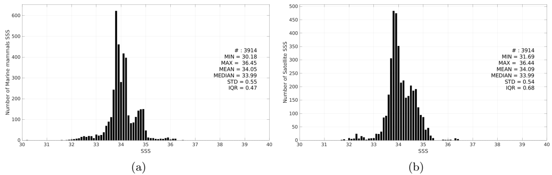
Figure 3: Histograms of SSS from Marine mammals (a) and SMOS SSS L3 v9 - 18 Days (CATDS-CEC-LOCEAN) (b) considering all match-up pairs per bins of 0.1 over the Atlantic Ocean Pi-MEP region and for the full satellite product period.
