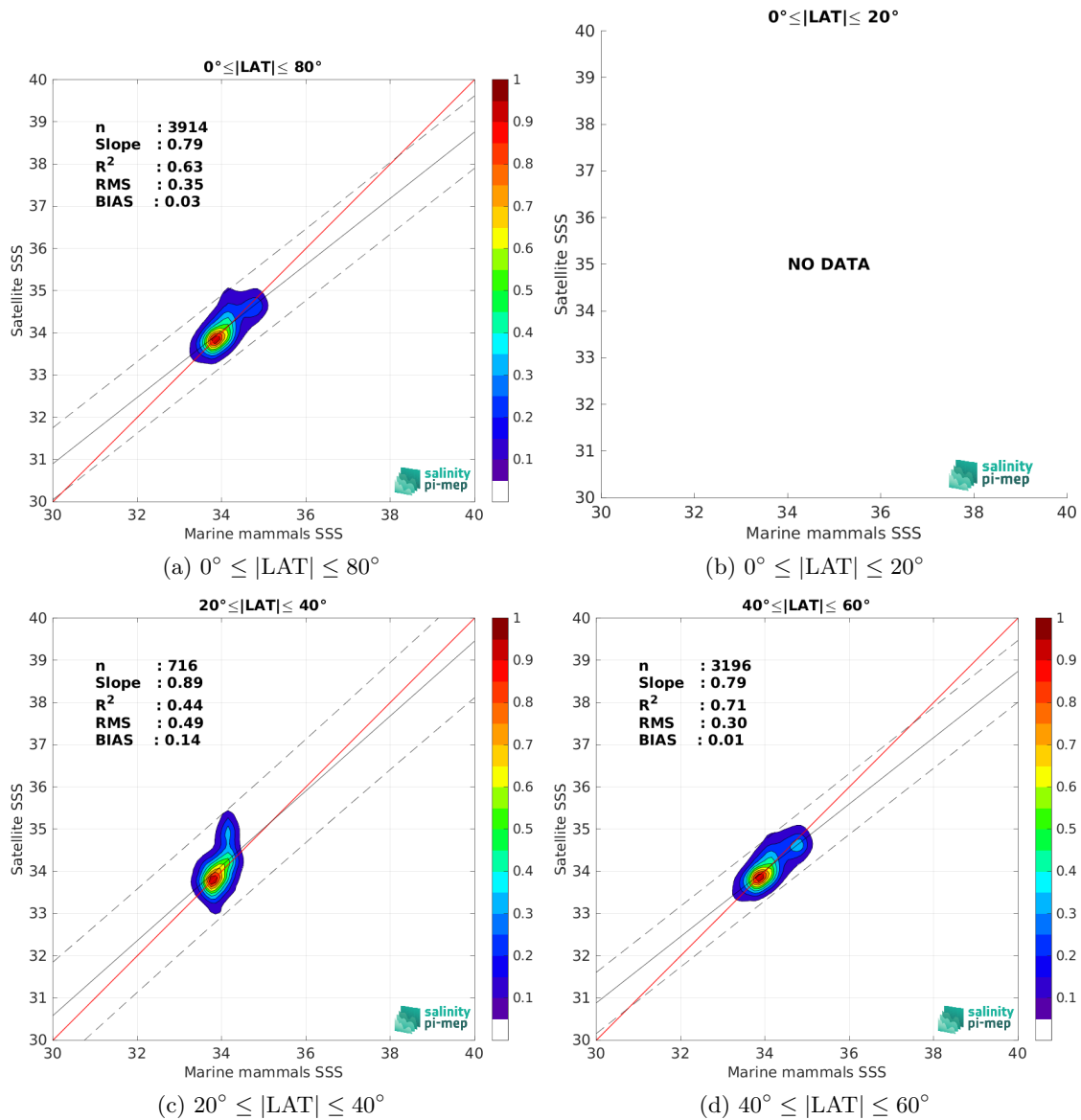
Figure 10: Contour maps of the concentration of SMOS SSS L3 v9 - 18 Days (CATDS-CEC-LOCEAN) SSS (y-axis) versus Marine mammals SSS (x-axis) at match-up pairs for different latitude bands. For each plot, the red line shows x=y . The black thin and dashed lines indicate a linear fit through the data cloud and the \pm 95\% confidence levels, respectively. The number match-up pairs n , the slope and R^2 coefficient of the linear fit, the root mean square (RMS) and the mean bias between satellite and in situ data are indicated for each latitude band in each plots.
