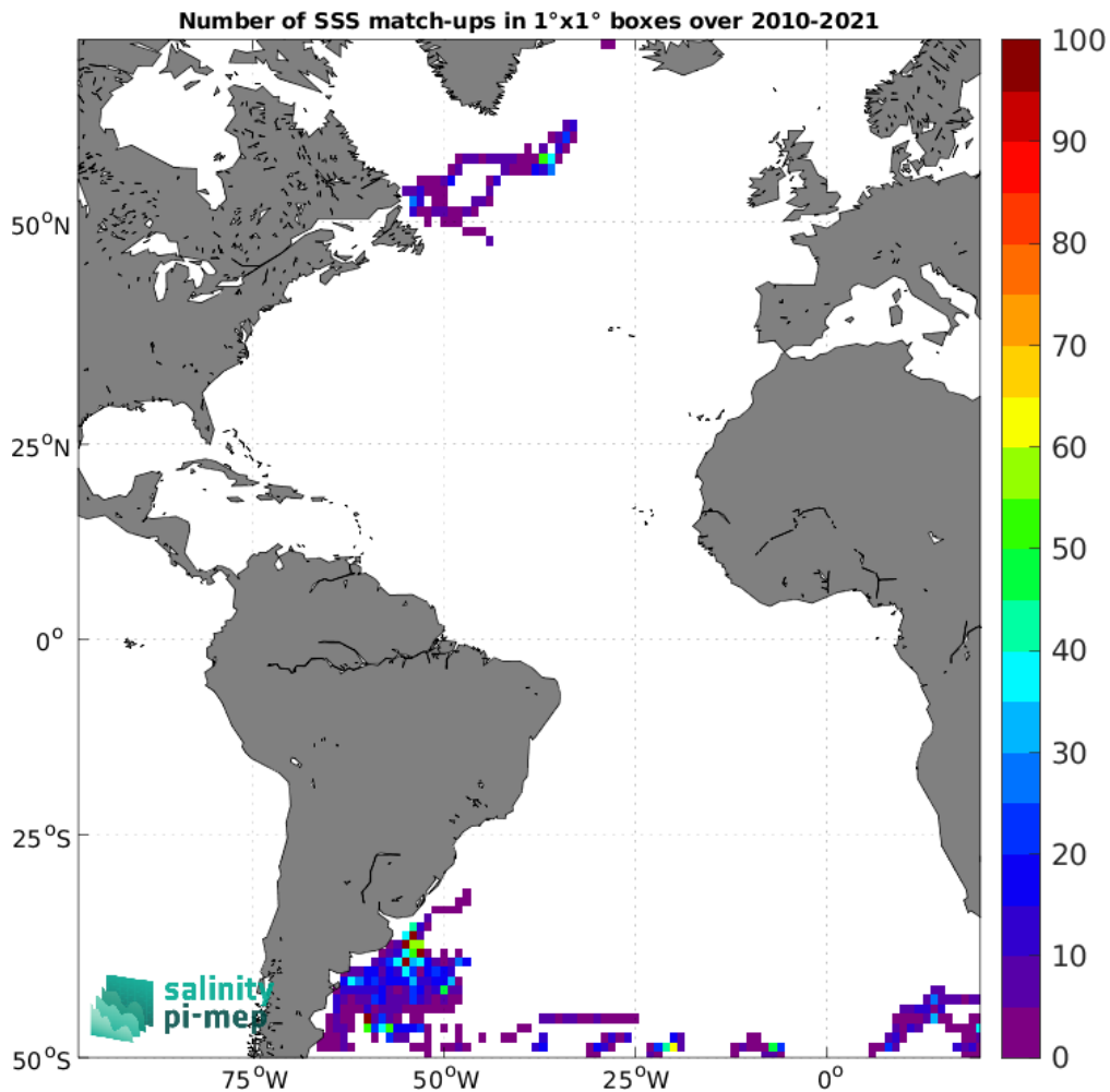
Figure 5: Number of SSS match-ups between Marine mammals SSS and the SMOS SSS L3 v9 - 18 Days (CATDS-CEC-LOCEAN) SSS product for the Atlantic Ocean Pi-MEP region over 1°x1° boxes and for the full satellite product period.
