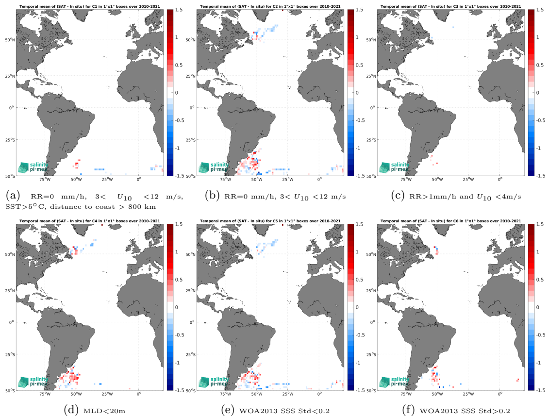
Figure 14: Temporal mean gridded over spatial boxes of size 1^\circ \times 1^\circ of \Delta SSS (SMOS SSS L3 v9 - 18 Days (CATDS-CEC-LOCEAN) - Marine mammals) for 6 different subdatasets corresponding to: RR=0 mm/h, 3 < U_{10} < 12 m/s, SST > 5°C, distance to coast > 800 km (a), RR=0 mm/h, 3 < U_{10} < 12 m/s (b), RR > 1 mm/h and U_{10} < 4 m/s (c), MLD < 20m (d), WOA2013 SSS Std < 0.2 (e), WOA2013 SSS Std > 0.2 (f).
