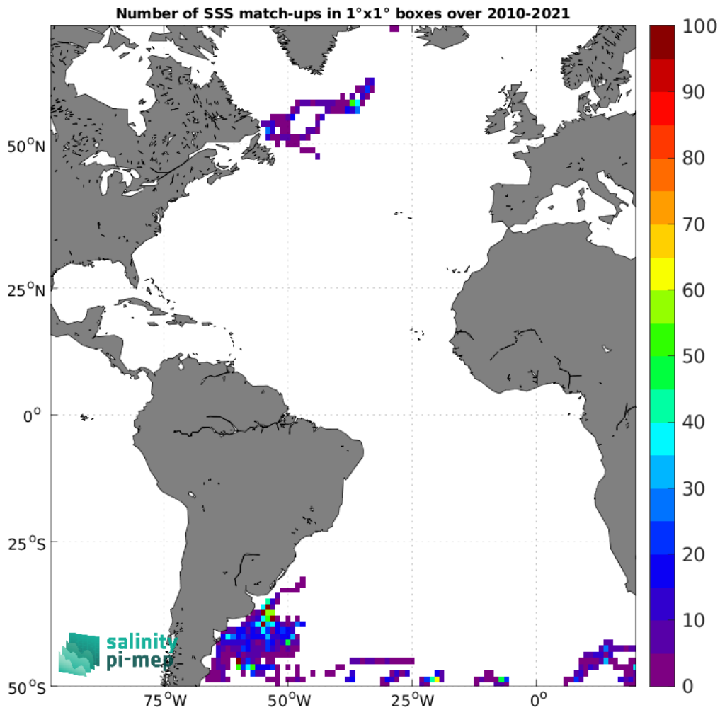
Figure 5: Number of SSS match-ups between Marine mammals SSS and the SMOS SSS L3 v9 - 18 Days (CATDS-CEC-LOCEAN) SSS product for the Atlantic Ocean Pi-MEP region over 1^\circ \times 1^\circ boxes and for the full satellite product period.
