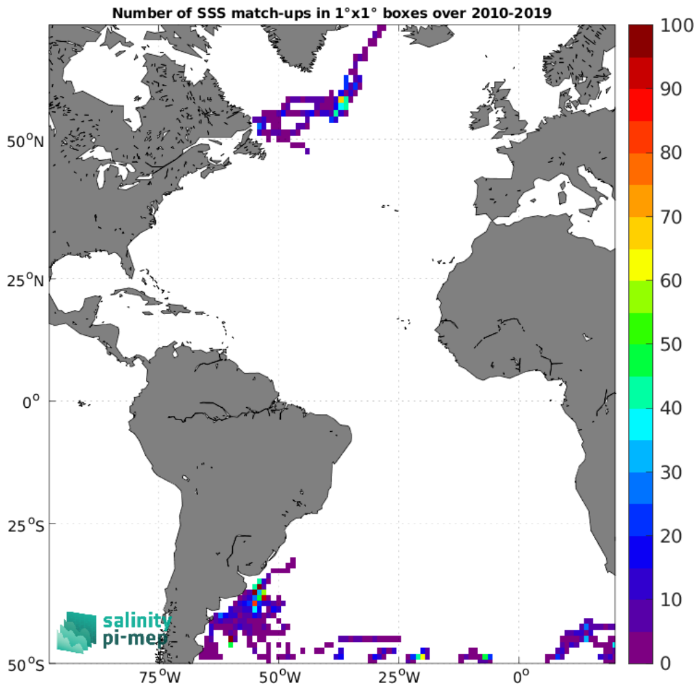
Figure 4: Number of SSS match-ups between Marine mammals SSS and the SMOS SSS L3 v9 - 18 Days (CATDS-CEC-LOCEAN) SSS product for the Atlantic Ocean Pi-MEP region over 1^\circ \times 1^\circ boxes and for the full satellite product period.
