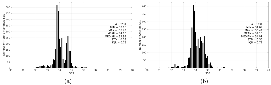
Figure 2: Histograms of SSS from Marine mammals (a) and SMOS SSS L3 v9 - 18 Days (CATDS-CEC-LOCEAN) (b) considering all match-up pairs per bins of 0.1 over the Atlantic Ocean Pi-MEP region and for the full satellite product period.
