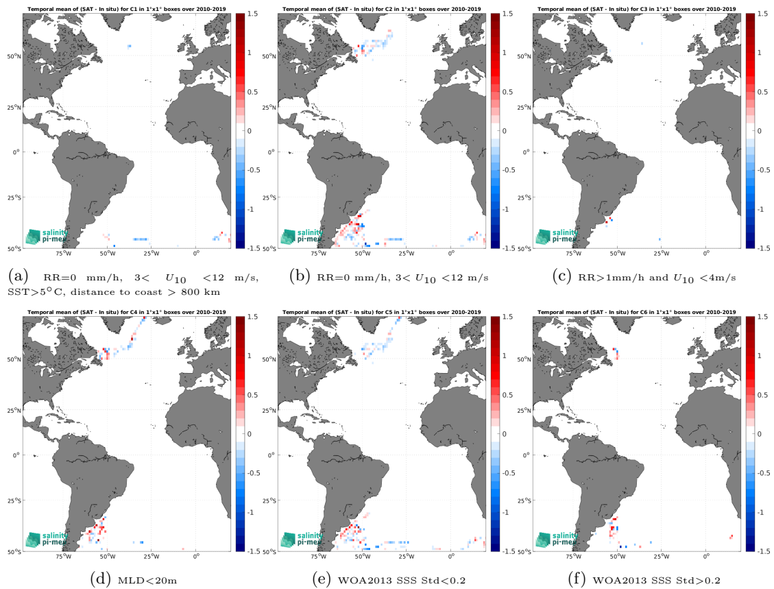
Figure 12: Temporal mean gridded over spatial boxes of size 1^\circ \times 1^\circ of \Delta SSS (SMOS SSS L3 v9 - 18 Days (CATDS-CEC-LOCEAN) - Marine mammals) for 6 different subdatasets corresponding to: RR=0 mm/h, 3 < U_{10} < 12 m/s, SST > 5°C, distance to coast > 800 km (a), RR=0 mm/h, 3 < U_{10} < 12 m/s (b), RR > 1mm/h and U_{10} < 4 m/s (c), MLD < 20m (d), WOA2013 SSS Std < 0.2 (e), WOA2013 SSS Std > 0.2 (f).
