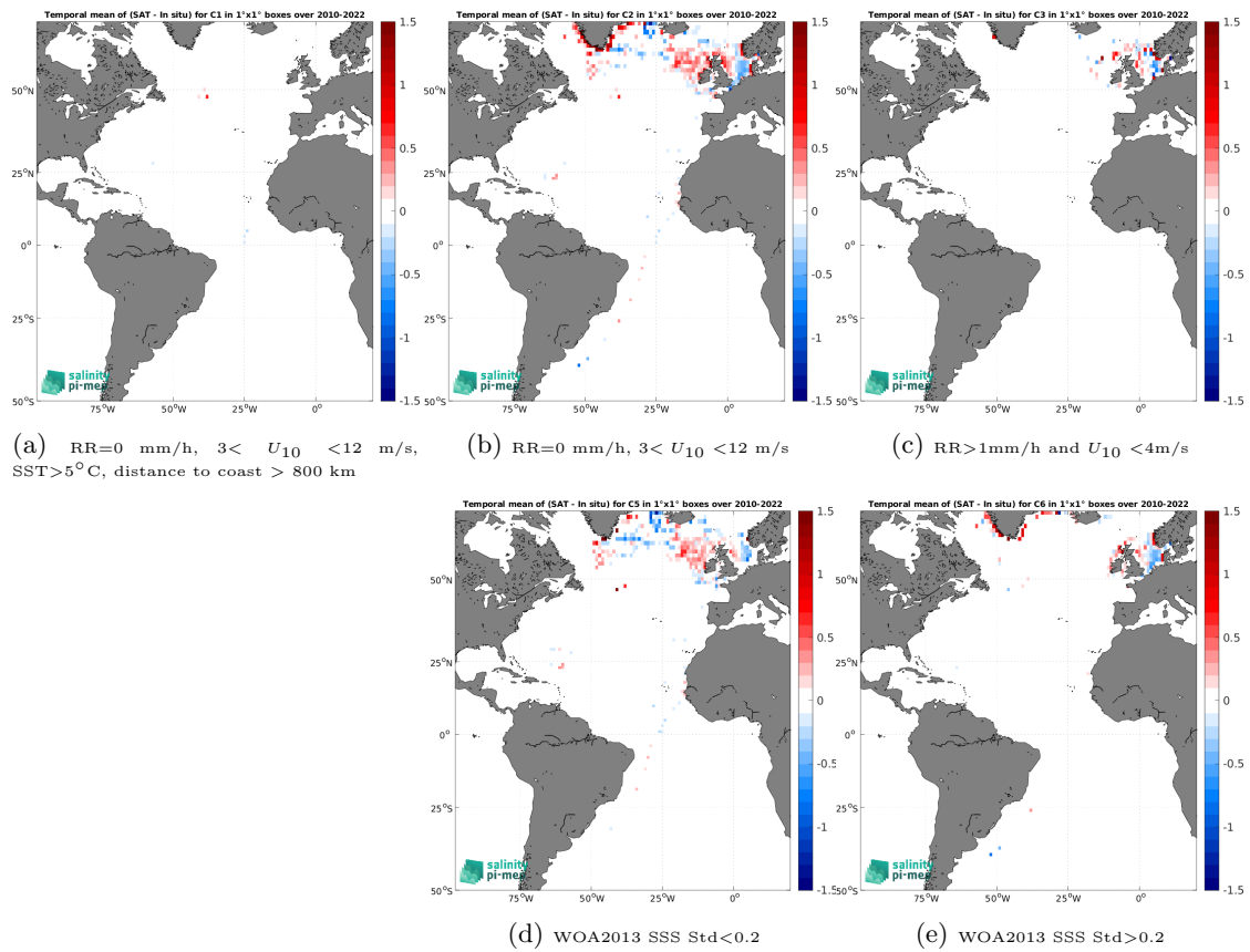
Figure 14: Temporal mean gridded over spatial boxes of size 1^\circ \times 1^\circ of \Delta SSS (SMOS SSS L3 v9 - 18 Days (CATDS-CEC-LOCEAN) - ICES) for 5 different subdatasets corresponding to:RR=0 mm/h, 3 < U_{10} < 12 m/s, SST>5°C, distance to coast > 800 km (a), RR=0 mm/h, 3 < U_{10} < 12 m/s (b), RR>1mm/h and U_{10} < 4 m/s (c), WOA2013 SSS Std<0.2 (d), WOA2013 SSS Std>0.2 (e).
