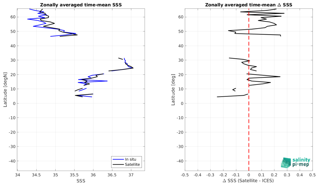
Figure 9: Left panel: Zonal mean SSS from SMOS SSS L3 v9 - 18 Days (CATDS-CEC-LOCEAN) satellite product (black) and from ICES (blue). Right panel: Zonal mean of \Delta SSS (Satellite - ICES) for all the collected Pi-MEP match-up pairs estimated over the full satellite product period.
