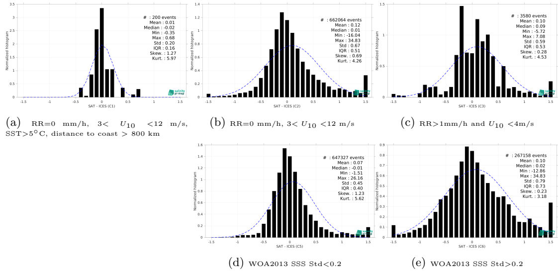
Figure 15: Normalized histogram of \Delta SSS (SMOS SSS L3 v9 - 18 Days (CATDS-CEC-LOCEAN) - ICES) for 5 different subdatasets corresponding to: RR=0 mm/h, 3 < U_{10} < 12 m/s, SST > 5°C, distance to coast > 800 km (a), RR=0 mm/h, 3 < U_{10} < 12 m/s (b), RR > 1mm/h and U_{10} < 4 m/s (c), WOA2013 SSS Std < 0.2 (d), WOA2013 SSS Std > 0.2 (e).
