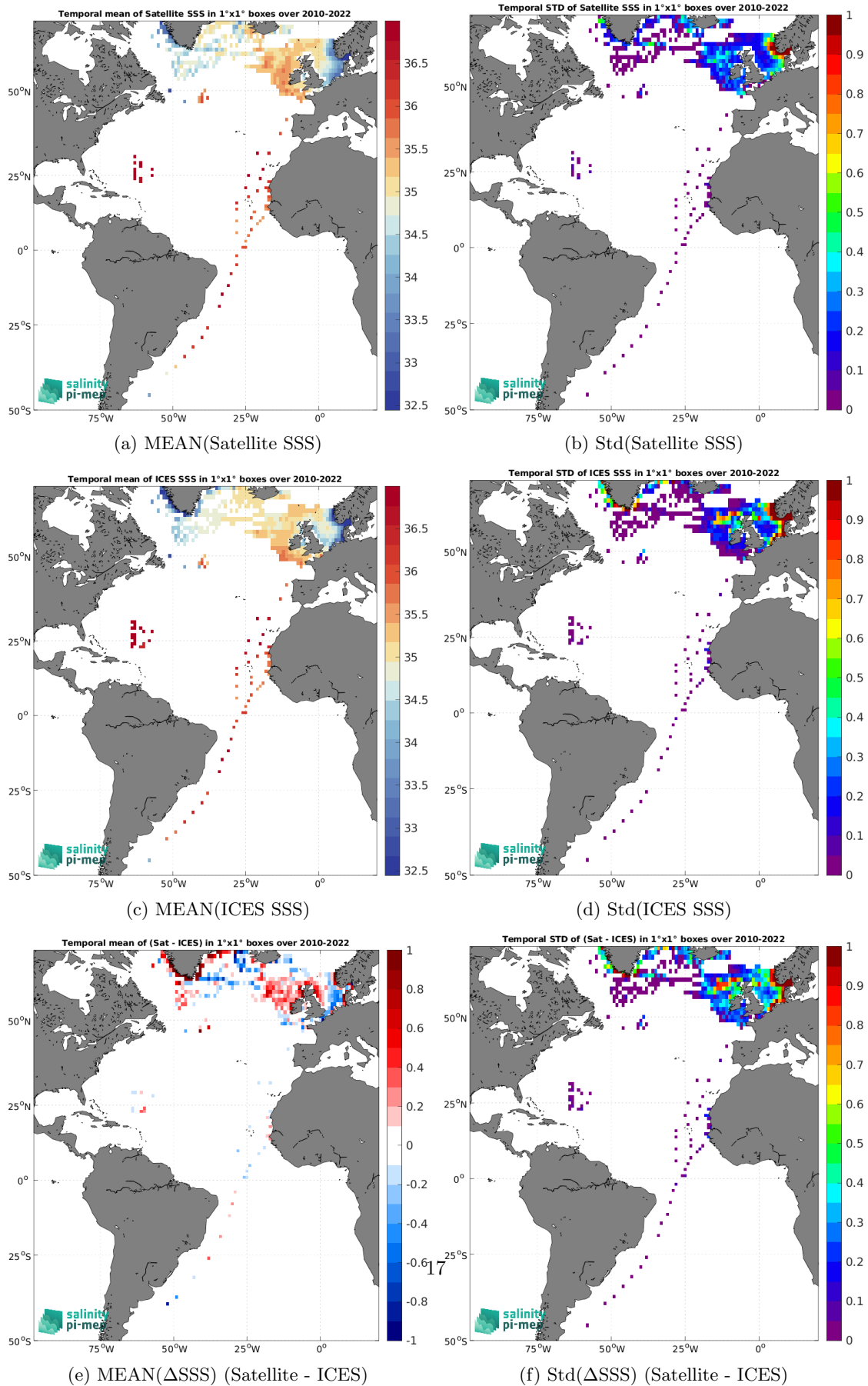
Figure 7: Temporal mean (left) and Std (right) of SSS from SMOS SSS L3 v9 - 18 Days (CATDS-CEC-LOCEAN) (top), ICES (middle), and of \Delta SSS (Satellite - ICES). Only match-up pairs are used to generate these maps.
