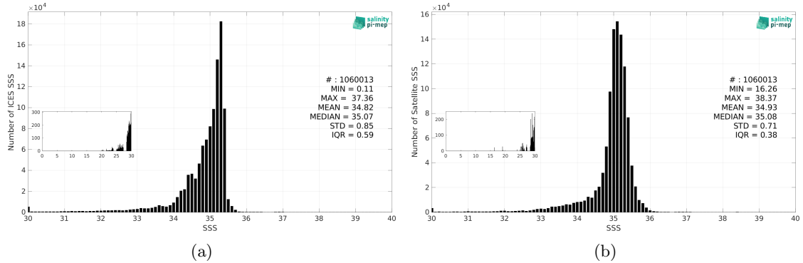
Figure 3: Histograms of SSS from ICES (a) and SMOS SSS L3 v9 - 18 Days (CATDS-CEC-LOCEAN) (b) considering all match-up pairs per bins of 0.1 over the Atlantic Ocean Pi-MEP region and for the full satellite product period.
