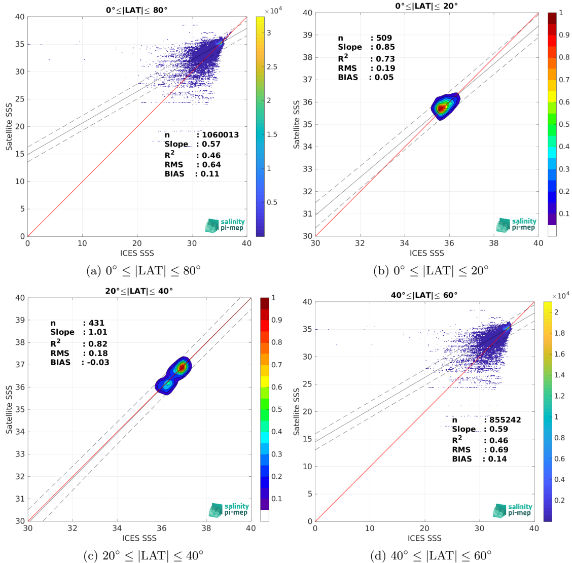
Figure 10: Contour maps of the concentration of SMOS SSS L3 v9 - 18 Days (CATDS-CEC-LOCEAN) SSS (y-axis) versus ICES SSS (x-axis) at match-up pairs for different latitude bands. For each plot, the red line shows x=y . The black thin and dashed lines indicate a linear fit through the data cloud and the \pm 95\% confidence levels, respectively. The number match-up pairs n , the slope and R^2 coefficient of the linear fit, the root mean square (RMS) and the mean bias between satellite and in situ data are indicated for each latitude band in each plots.
