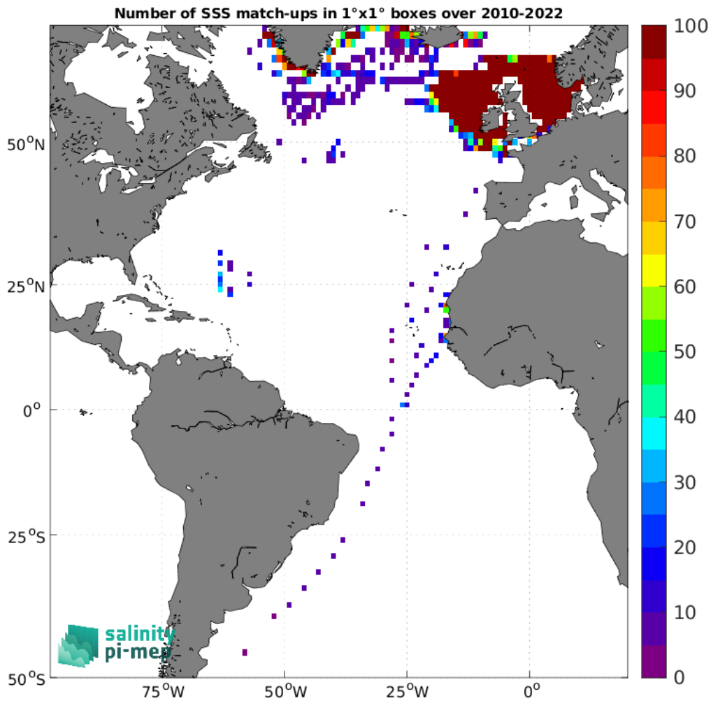
Figure 5: Number of SSS match-ups between ICES SSS and the SMOS SSS L3 v9 - 18 Days (CATDS-CEC-LOCEAN) SSS product for the Atlantic Ocean Pi-MEP region over 1^\circ \times 1^\circ boxes and for the full satellite product period.
