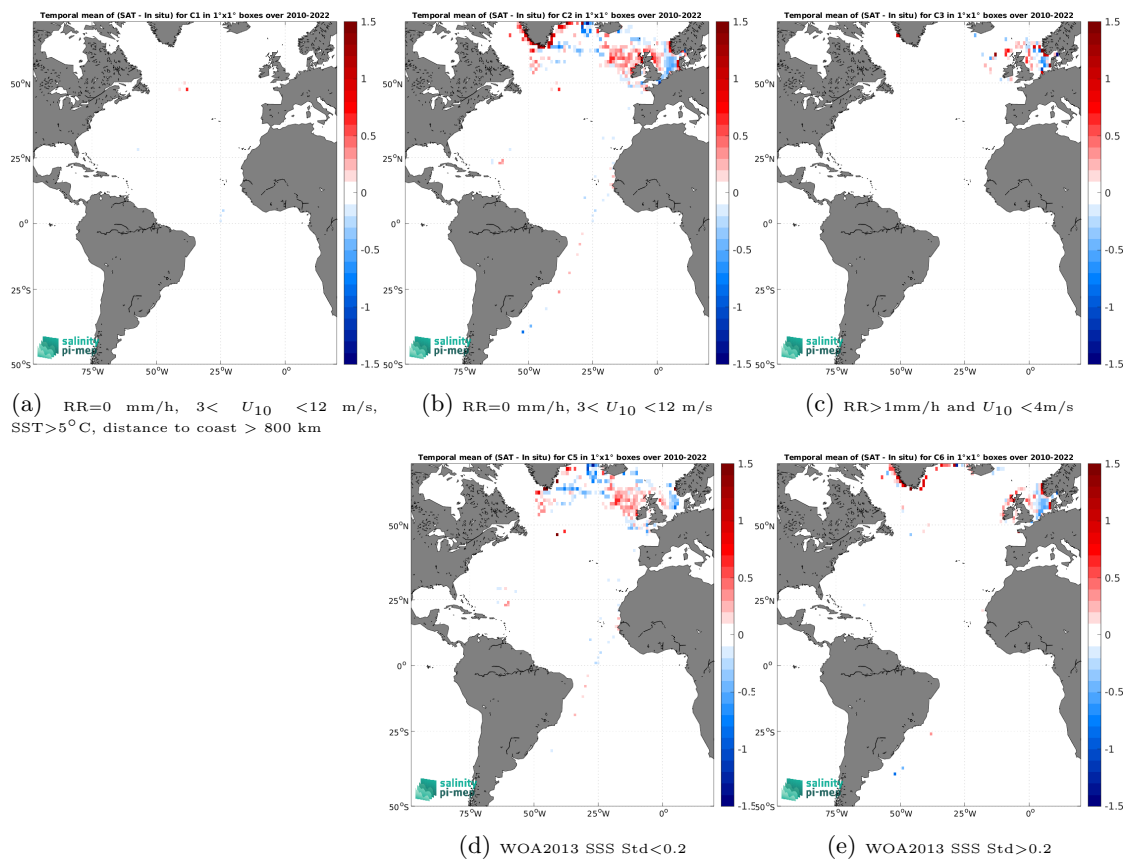
Figure 14: Temporal mean gridded over spatial boxes of size 1^\circ \times 1^\circ of \Delta\text{SSS} (SMOS SSS L3 v9 - 18 Days (CATDS-CEC-LOCEAN) - ICES) for 5 different subdatasets corresponding to:RR=0 mm/h, 3 < U_{10} < 12 m/s, SST>5°C, distance to coast > 800 km (a), RR=0 mm/h, 3 < U_{10} < 12 m/s (b), RR>1mm/h and U_{10} < 4 m/s (c), WOA2013 SSS Std<0.2 (d), WOA2013 SSS Std>0.2 (e).
