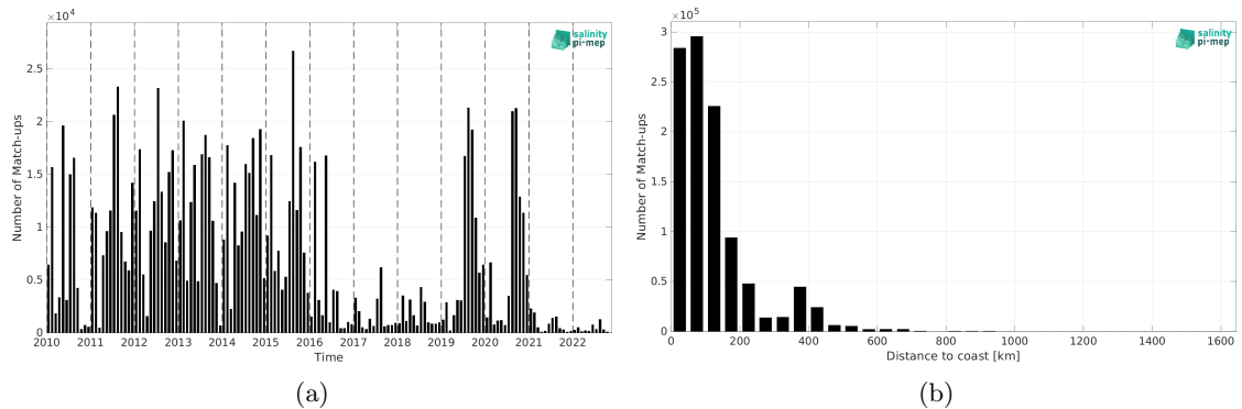
Figure 2: Number of match-ups between ICES and SMOS SSS L3 v9 - 18 Days (CATDS-CEC-LOCEAN) SSS as a function of time (a) and as function of the distance to coast (b) over the Atlantic Ocean Pi-MEP region and for the full satellite product period.
