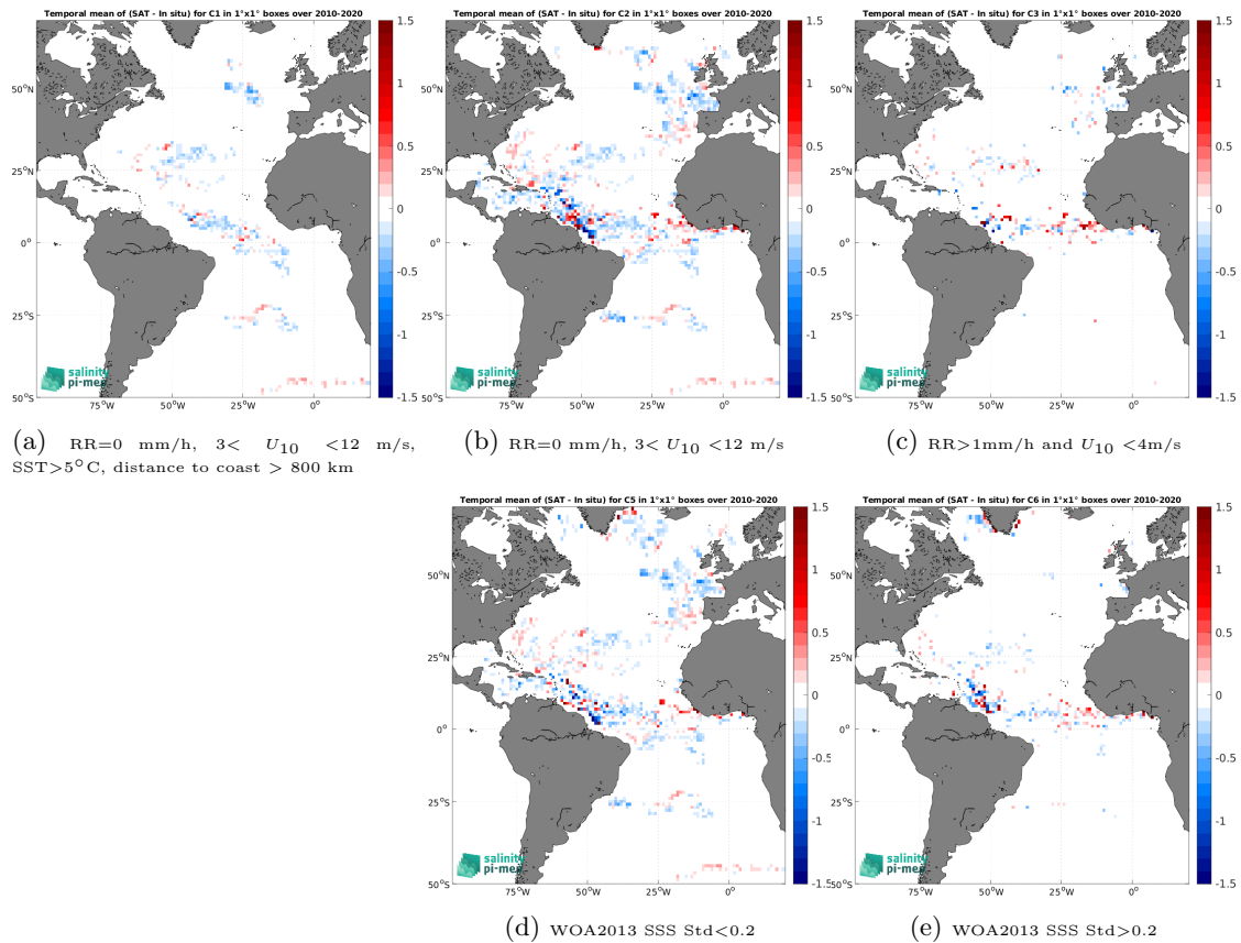
Figure 11: Temporal mean gridded over spatial boxes of size 1^\circ \times 1^\circ of \Delta SSS (SMOS SSS L3 v9 - 18 Days (CATDS-CEC-LOCEAN) - Surface drifters) for 5 different subdatasets corresponding to:RR=0 mm/h, 3 < U_{10} < 12 m/s, SST >5^\circ\text{C} , distance to coast > 800 km (a), RR=0 mm/h, 3 < U_{10} < 12 m/s (b), RR >1 mm/h and U_{10} < 4 m/s (c), WOA2013 SSS Std <0.2 (d), WOA2013 SSS Std >0.2 (e).
