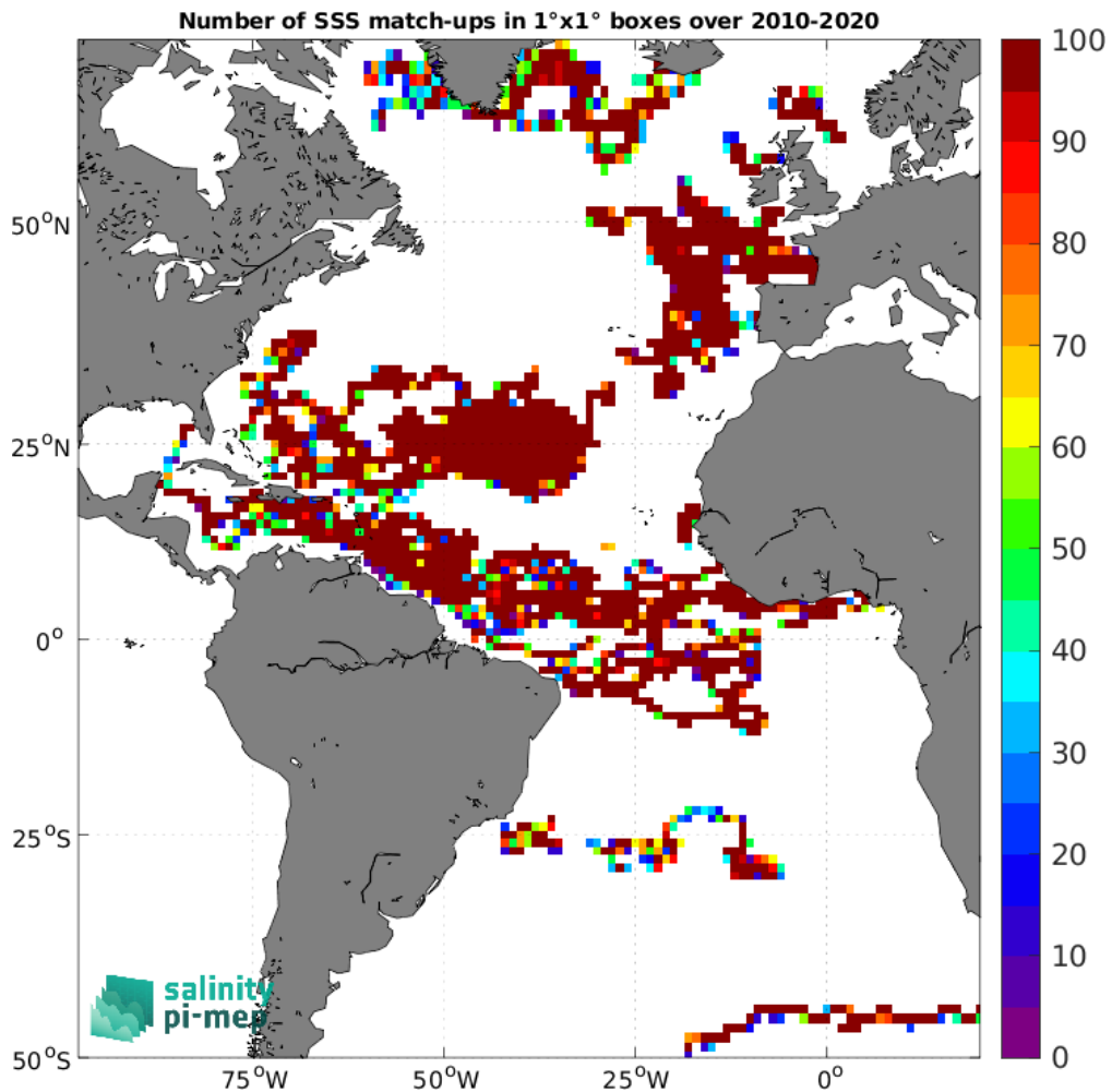
Figure 3: Number of SSS match-ups between Surface drifters SSS and the SMOS SSS L3 v9 - 18 Days (CATDS-CEC-LOCEAN) SSS product for the Atlantic Ocean Pi-MEP region over 1°x1° boxes and for the full satellite product period.
