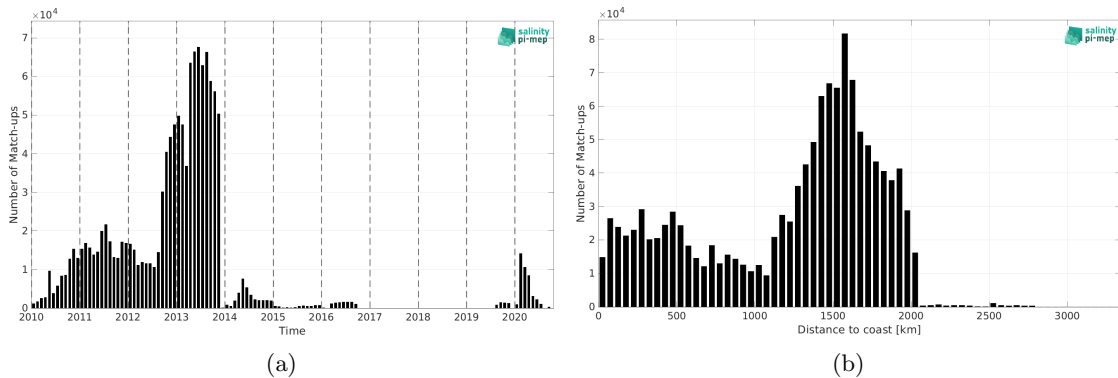
Figure 1: Number of match-ups between Surface drifters and SMOS SSS L3 v9 - 18 Days (CATDS-CEC-LOCEAN) SSS as a function of time (a) and as function of the distance to coast (b) over the Atlantic Ocean Pi-MEP region and for the full satellite product period.
