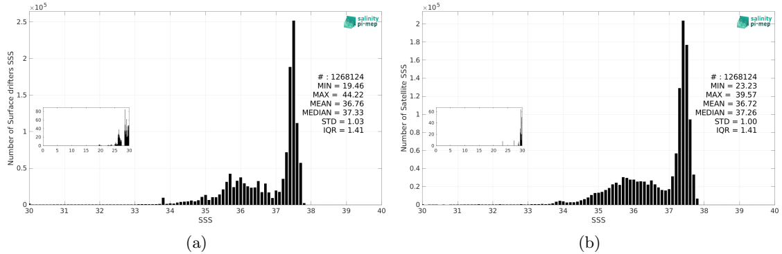
Figure 2: Histograms of SSS from Surface drifters (a) and SMOS SSS L3 v9 - 18 Days (CATDS-CEC-LOCEAN) (b) considering all match-up pairs per bins of 0.1 over the Atlantic Ocean Pi-MEP region and for the full satellite product period.
