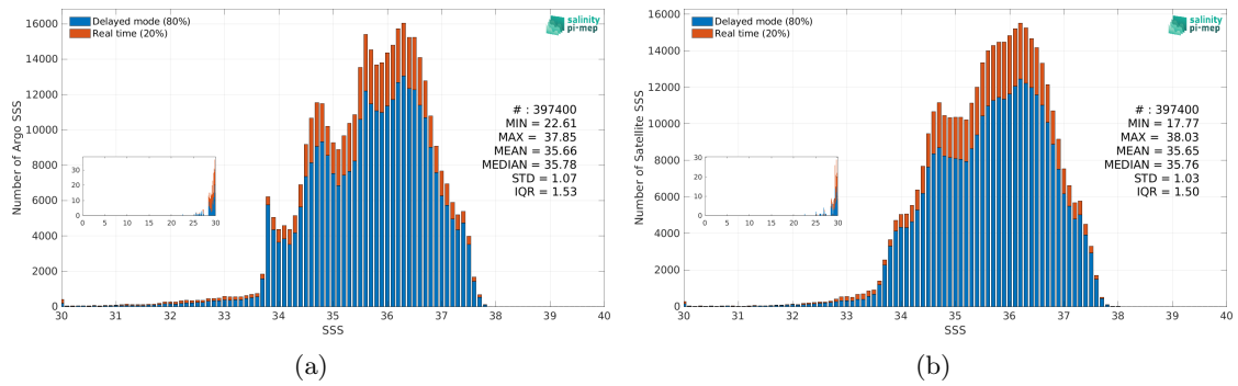
Figure 2: Histograms of SSS from Argo (a) and SMOS SSS L3 v9 - 18 Days (CATDS-CEC-LOCEAN) (b) considering all match-up pairs per bins of 0.1 over the Atlantic Ocean Pi-MEP region and for the full satellite product period.
