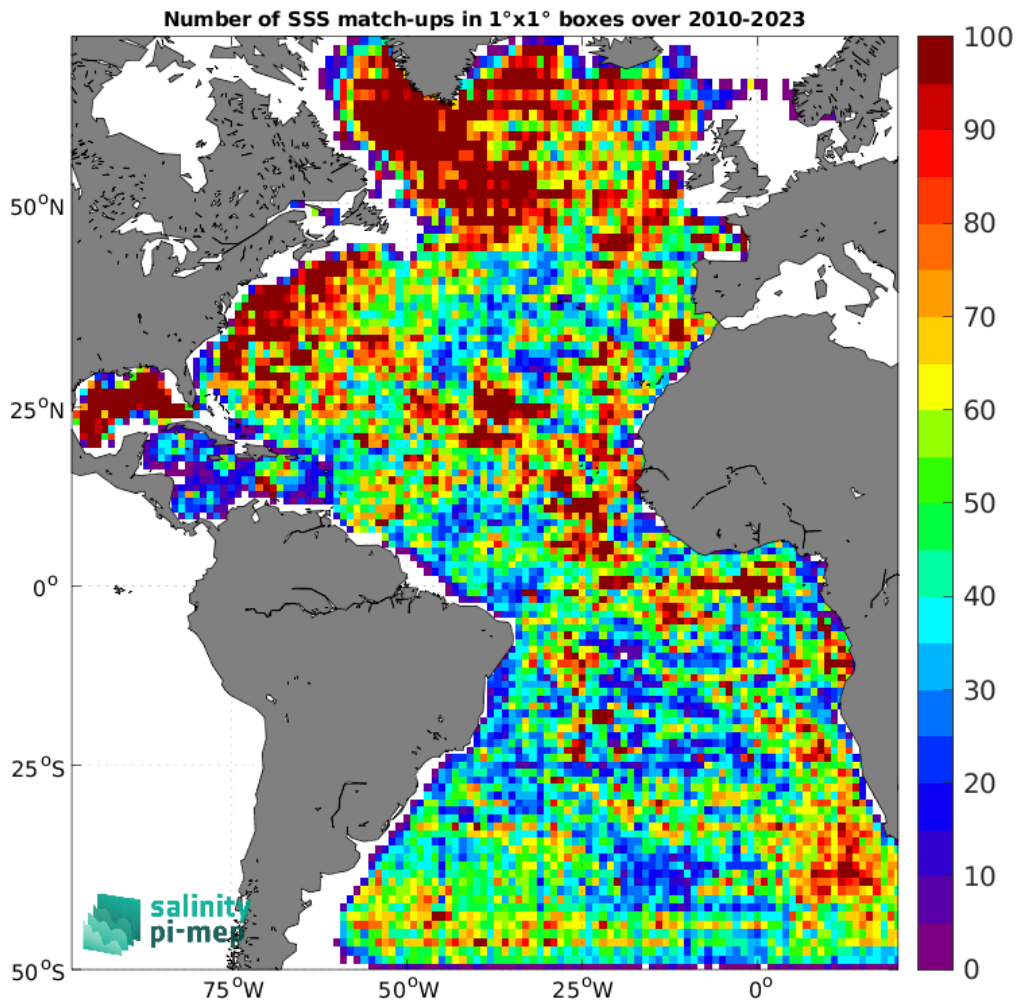
Figure 4: Number of SSS match-ups between Argo SSS and the SMOS SSS L3 v9 - 18 Days (CATDS-CEC-LOCEAN) SSS product for the Atlantic Ocean Pi-MEP region over 1^\circ \times 1^\circ boxes and for the full satellite product period.
