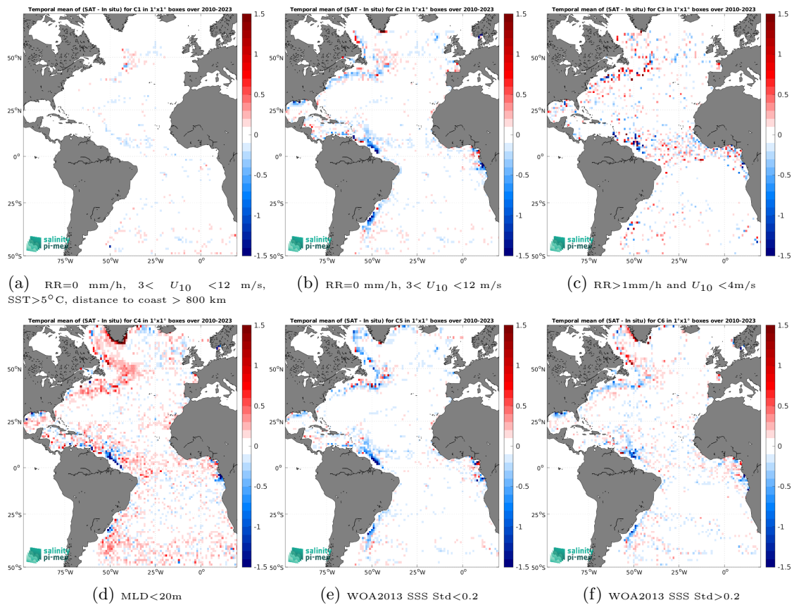
Figure 12: Temporal mean gridded over spatial boxes of size 1^\circ \times 1^\circ of \Delta SSS (SMOS SSS L3 v9 - 18 Days (CATDS-CEC-LOCEAN) - Argo) for 6 different subdatasets corresponding to:RR=0 mm/h, 3 < U_{10} < 12 m/s, SST >5^\circ C, distance to coast > 800 km (a), RR=0 mm/h, 3 < U_{10} < 12 m/s (b), RR >1 mm/h and U_{10} < 4 m/s (c),MLD <20 m (d),WOA2013 SSS Std <0.2 (e),WOA2013 SSS Std >0.2 (f).
