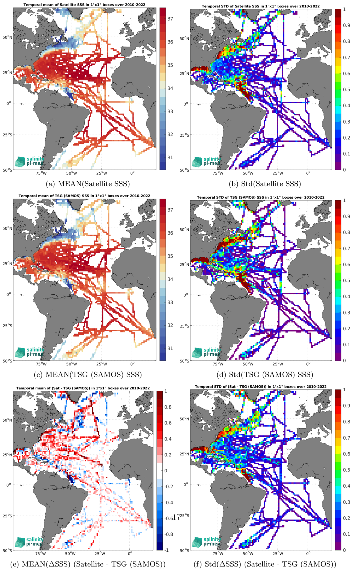
Figure 6: Temporal mean (left) and Std (right) of SSS from SMOS SSS L3 v8 - 9 Days (CATDS-CEC-LOCEAN) (top), TSG (SAMOS) (middle), and of \Delta SSS (Satellite - TSG (SAMOS)). Only match-up pairs are used to generate these maps.
