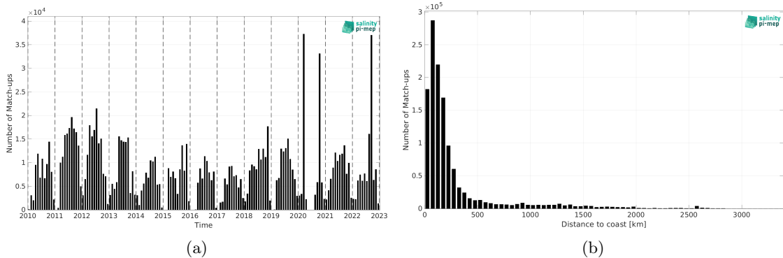
Figure 1: Number of match-ups between TSG (SAMOS) and SMOS SSS L3 v8 - 9 Days (CATDS-CEC-LOCEAN) SSS as a function of time (a) and as function of the distance to coast (b) over the Atlantic Ocean Pi-MEP region and for the full satellite product period.
