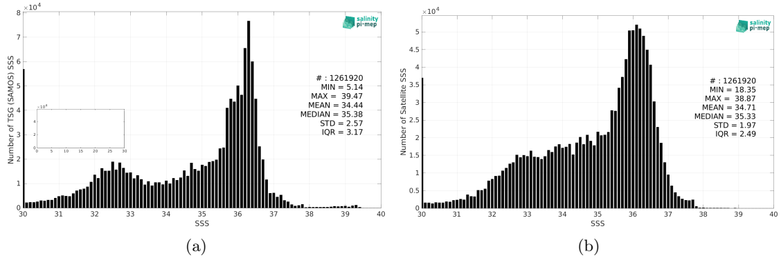
Figure 2: Histograms of SSS from TSG (SAMOS) (a) and SMOS SSS L3 v8 - 9 Days (CATDS-CEC-LOCEAN) (b) considering all match-up pairs per bins of 0.1 over the Atlantic Ocean Pi-MEP region and for the full satellite product period.
