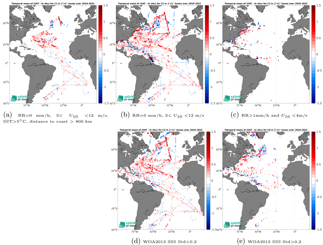
Figure 12: Temporal mean gridded over spatial boxes of size 1^\circ \times 1^\circ of \Delta SSS (SMOS SSS L3 v8 - 9 Days (CATDS-CEC-LOCEAN) - TSG (SAMOS)) for 5 different subdatasets corresponding to:RR=0 mm/h, 3 < U_{10} < 12 m/s, SST >5^\circ\text{C} , distance to coast > 800 km (a), RR=0 mm/h, 3 < U_{10} < 12 m/s (b), RR >1 mm/h and U_{10} < 4 m/s (c), WOA2013 SSS Std <0.2 (d), WOA2013 SSS Std >0.2 (e).
