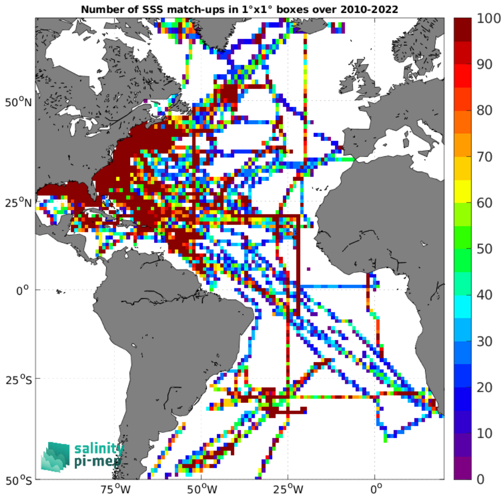
Figure 4: Number of SSS match-ups between TSG (SAMOS) SSS and the SMOS SSS L3 v8 - 9 Days (CATDS-CEC-LOCEAN) SSS product for the Atlantic Ocean Pi-MEP region over 1^\circ \times 1^\circ boxes and for the full satellite product period.
