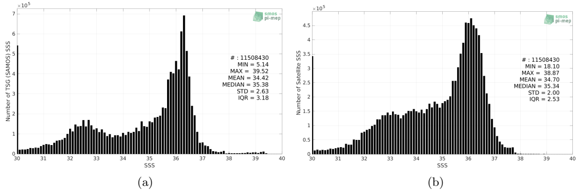
Figure 2: Histograms of SSS from TSG (SAMOS) (a) and SMOS SSS L3 v8 - 9 Days (CATDS-CECOS-LOCEAN) (b) considering all match-up pairs per bins of 0.1 over the Atlantic Ocean Pi-MEP region and for the full satellite product period.
