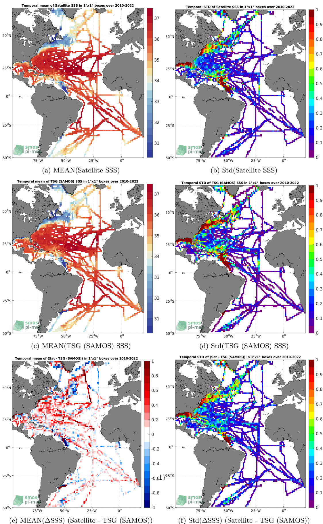
Figure 6: Temporal mean (left) and Std (right) of SSS from SMOS SSS L3 v8 - 9 Days (CATDS-CECOS-LOCEAN) (top), TSG (SAMOS) (middle), and of \Delta SSS (Satellite - TSG (SAMOS)). Only match-up pairs are used to generate these maps.
