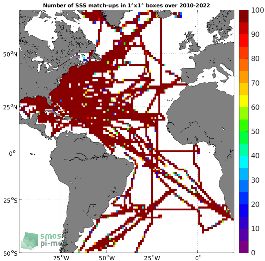
Figure 4: Number of SSS match-ups between TSG (SAMOS) SSS and the SMOS SSS L3 v8 - 9 Days (CATDS-CECOS-LOCEAN) SSS product for the Atlantic Ocean Pi-MEP region over 1°x1° boxes and for the full satellite product period.
