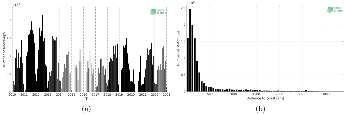
Figure 1: Number of match-ups between TSG (SAMOS) and SMOS SSS L3 v8 - 9 Days (CATDS-CECOS-LOCEAN) SSS as a function of time (a) and as function of the distance to coast (b) over the Atlantic Ocean Pi-MEP region and for the full satellite product period.
