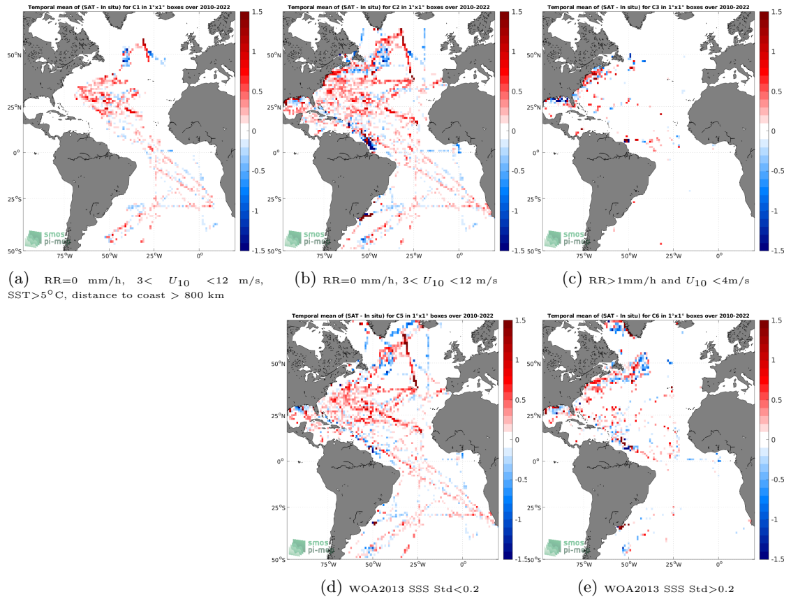
Figure 12: Temporal mean gridded over spatial boxes of size 1^\circ \times 1^\circ of \Delta SSS (SMOS SSS L3 v8 - 9 Days (CATDS-CECOS-LOCEAN) - TSG (SAMOS)) for 5 different subdatasets corresponding to:RR=0 mm/h, 3 < U_{10} < 12 m/s, SST >5^\circ\text{C} , distance to coast > 800 km (a), RR=0 mm/h, 3 < U_{10} < 12 m/s (b), RR >1 mm/h and U_{10} < 4 m/s (c), WOA2013 SSS Std <0.2 (d), WOA2013 SSS Std >0.2 (e).
