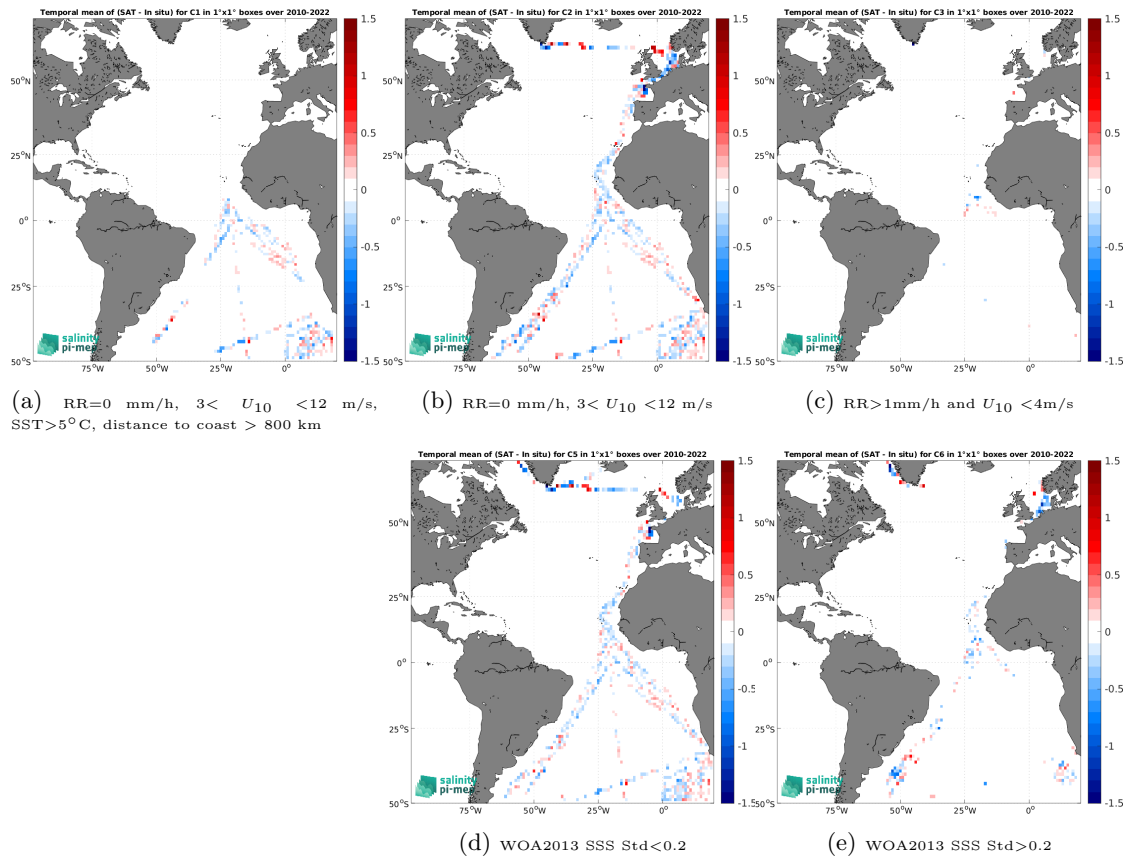
Figure 12: Temporal mean gridded over spatial boxes of size 1^\circ \times 1^\circ of \Delta SSS (SMOS SSS L3 v8 - 9 Days (CATDS-CEC-LOCEAN) - TSG (Polarstern)) for 5 different subdatasets corresponding to:RR=0 mm/h, 3 < U_{10} < 12 m/s, SST >5^\circ\text{C} , distance to coast > 800 km (a), RR=0 mm/h, 3 < U_{10} < 12 m/s (b), RR >1 mm/h and U_{10} < 4 m/s (c), WOA2013 SSS Std <0.2 (d), WOA2013 SSS Std >0.2 (e).
