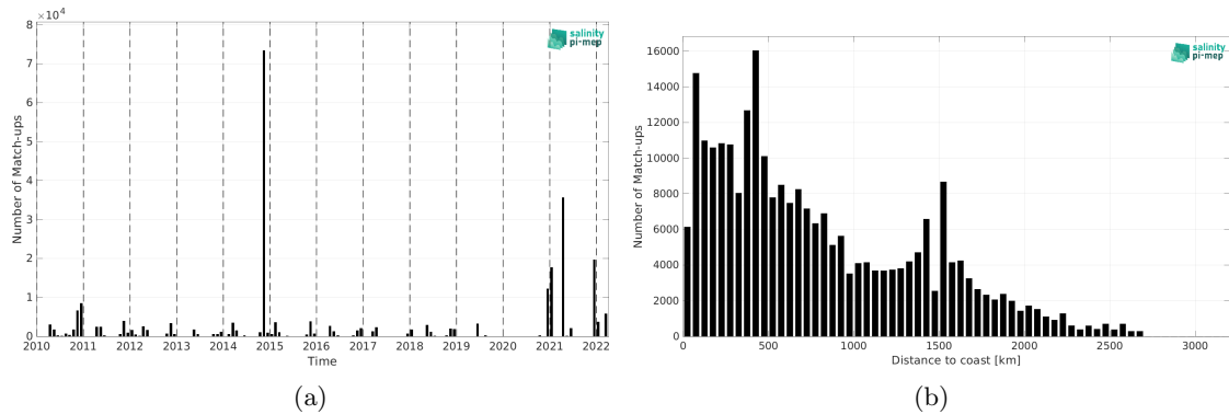
Figure 1: Number of match-ups between TSG (Polarstern) and SMOS SSS L3 v8 - 9 Days (CATDS-CEC-LOCEAN) SSS as a function of time (a) and as function of the distance to coast (b) over the Atlantic Ocean Pi-MEP region and for the full satellite product period.
