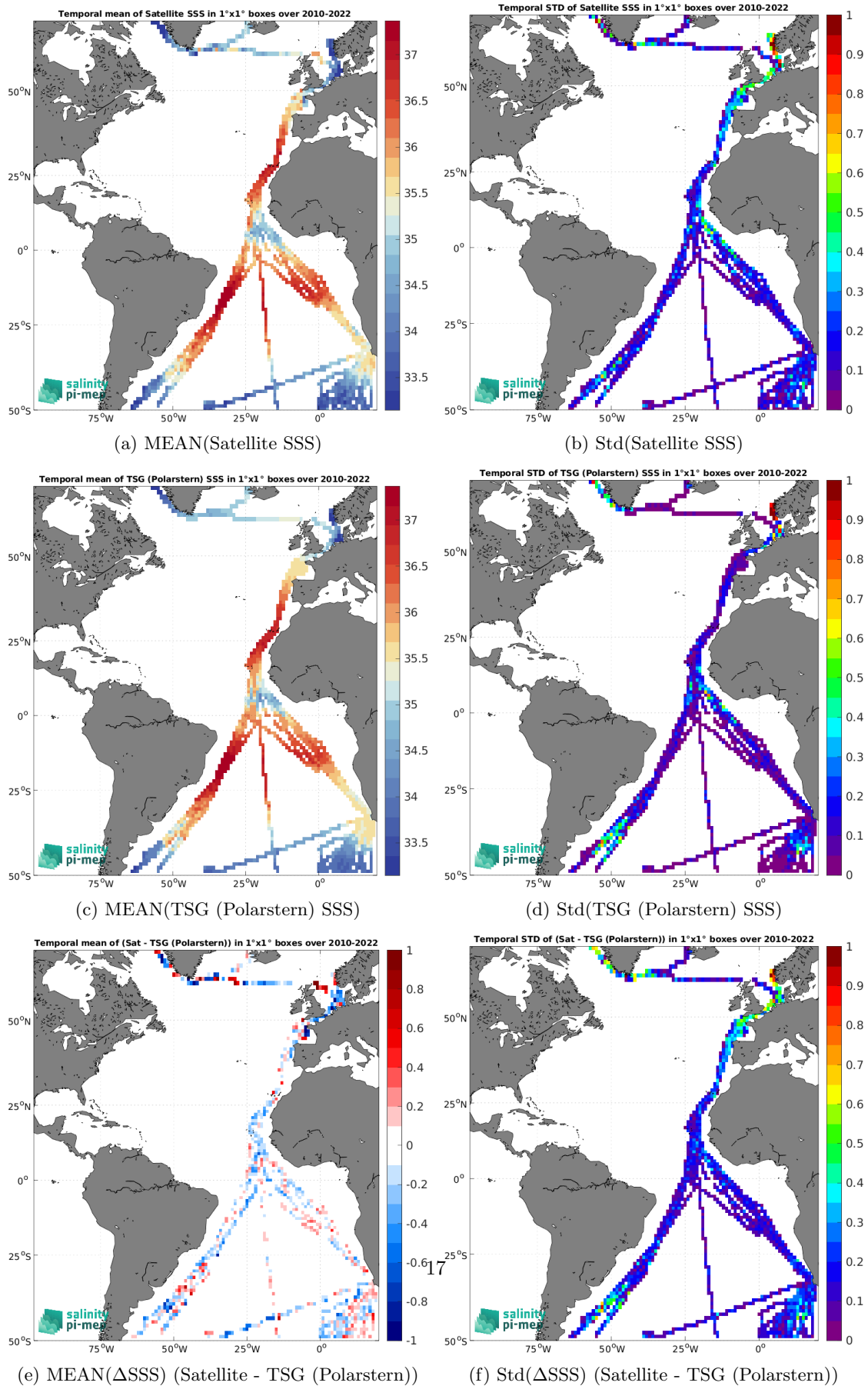
Figure 6: Temporal mean (left) and Std (right) of SSS from SMOS SSS L3 v8 - 9 Days (CATDS-CEC-LOCEAN) (top), TSG (Polarstern) (middle), and of \Delta SSS (Satellite - TSG (Polarstern)). Only match-up pairs are used to generate these maps.
