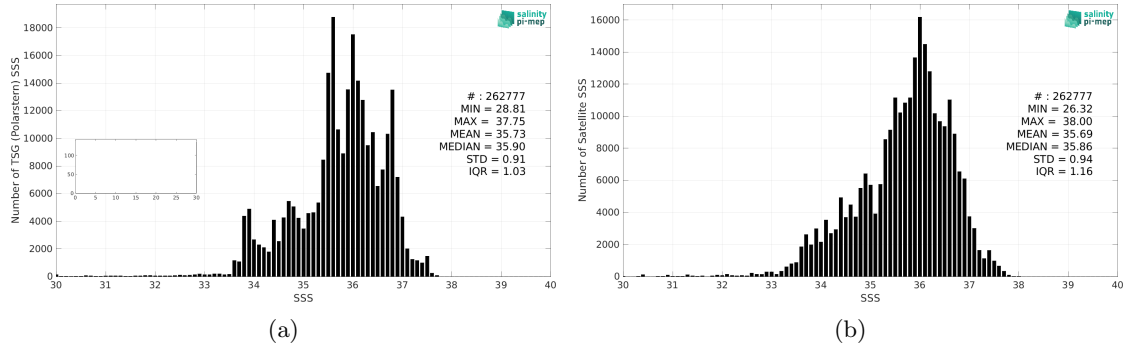
Figure 2: Histograms of SSS from TSG (Polarstern) (a) and SMOS SSS L3 v8 - 9 Days (CATDS-CEC-LOCEAN) (b) considering all match-up pairs per bins of 0.1 over the Atlantic Ocean Pi-MEP region and for the full satellite product period.
