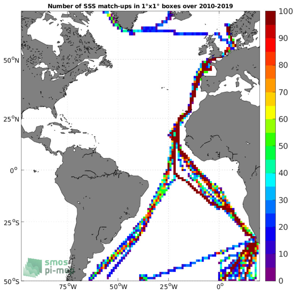
Figure 4: Number of SSS match-ups between TSG (Polarstern) SSS and the SMOS SSS L3 v8 - 9 Days (CATDS-CECOS-LOCEAN) SSS product for the Atlantic Ocean Pi-MEP region over 1°x1° boxes and for the full satellite product period.
