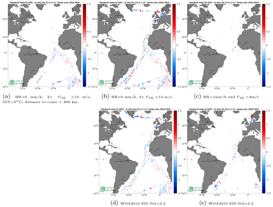
Figure 12: Temporal mean gridded over spatial boxes of size 1^\circ \times 1^\circ of \Delta SSS (SMOS SSS L3 v8 - 9 Days (CATDS-CECOS-LOCEAN) - TSG (Polarstern)) for 5 different subdatasets corresponding to:RR=0 mm/h, 3 < U_{10} < 12 m/s, SST >5^\circ C, distance to coast > 800 km (a), RR=0 mm/h, 3 < U_{10} < 12 m/s (b), RR >1 mm/h and U_{10} < 4 m/s (c), WOA2013 SSS Std <0.2 (d), WOA2013 SSS Std >0.2 (e).
