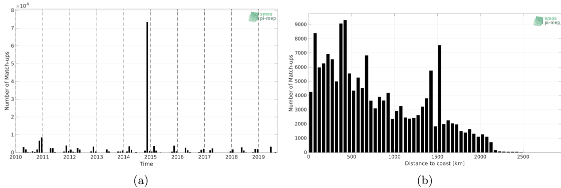
Figure 1: Number of match-ups between TSG (Polarstern) and SMOS SSS L3 v8 - 9 Days (CATDS-CECOS-LOCEAN) SSS as a function of time (a) and as function of the distance to coast (b) over the Atlantic Ocean Pi-MEP region and for the full satellite product period.
