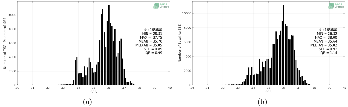
Figure 2: Histograms of SSS from TSG (Polarstern) (a) and SMOS SSS L3 v8 - 9 Days (CATDS-CECOS-LOCEAN) (b) considering all match-up pairs per bins of 0.1 over the Atlantic Ocean Pi-MEP region and for the full satellite product period.
