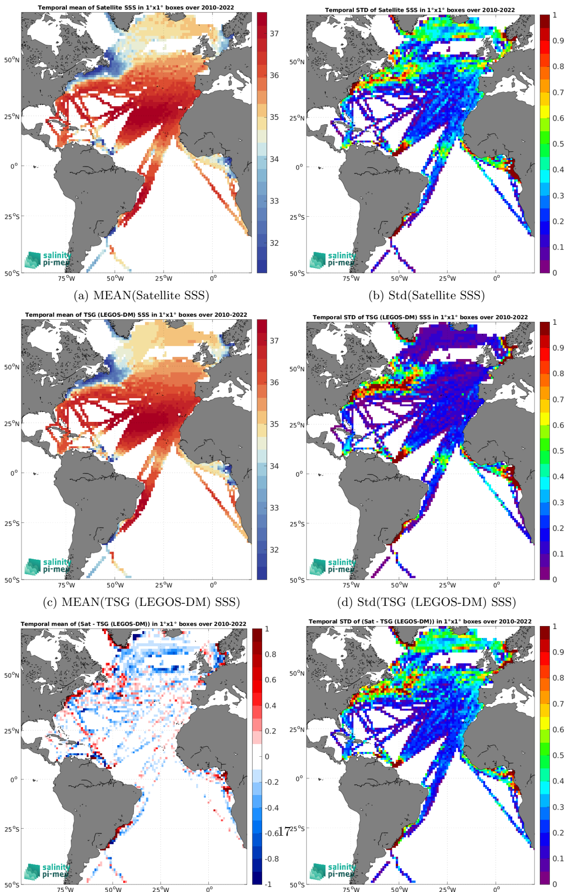
Figure 6: Temporal mean (left) and Std (right) of SSS from SMOS SSS L3 v8 - 9 Days (CATDS-CEC-LOCEAN) (top), TSG (LEGOS-DM) (middle), and of \Delta SSS (Satellite - TSG (LEGOS-DM)). Only match-up pairs are used to generate these maps.
