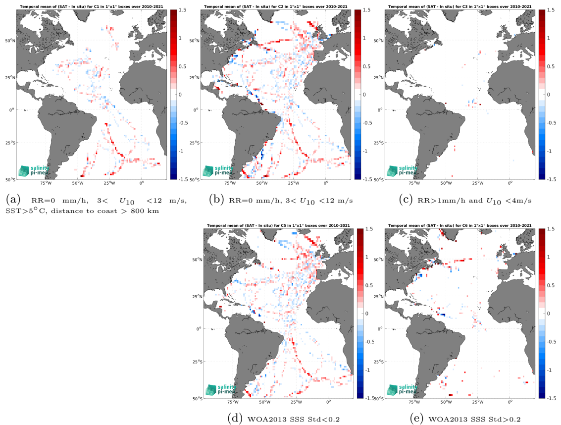
Figure 12: Temporal mean gridded over spatial boxes of size 1^\circ \times 1^\circ of \Delta\text{SSS} (SMOS SSS L3 v8 - 9 Days (CATDS-CEC-LOCEAN) - TSG (GOSUD-Sailing-ship)) for 5 different subdatasets corresponding to:RR=0 mm/h, 3 < U_{10} < 12 m/s, SST >5^\circ\text{C} , distance to coast > 800 km (a), RR=0 mm/h, 3 < U_{10} < 12 m/s (b), RR >1 mm/h and U_{10} < 4 m/s (c), WOA2013 SSS Std <0.2 (d), WOA2013 SSS Std >0.2 (e).
