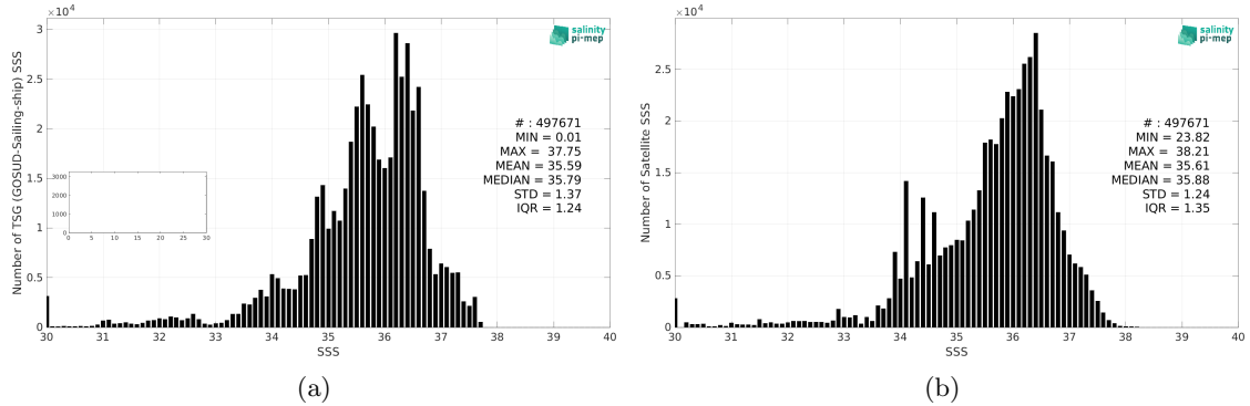
Figure 2: Histograms of SSS from TSG (GOSUD-Sailing-ship) (a) and SMOS SSS L3 v8 - 9 Days (CATDS-CEC-LOCEAN) (b) considering all match-up pairs per bins of 0.1 over the Atlantic Ocean Pi-MEP region and for the full satellite product period.
