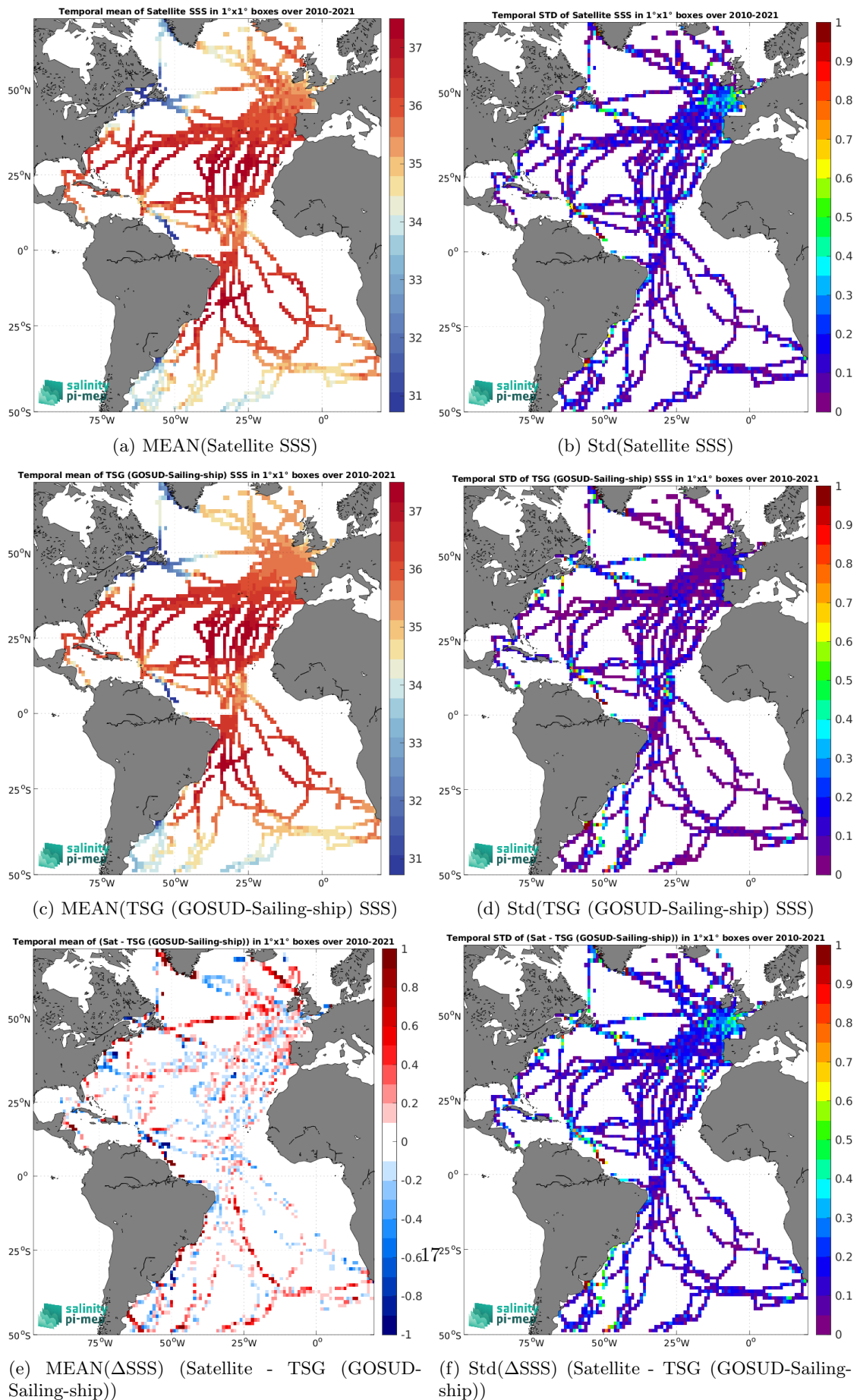
Figure 6: Temporal mean (left) and Std (right) of SSS from SMOS SSS L3 v8 - 9 Days (CATDS-CEC-LOCEAN) (top), TSG (GOSUD-Sailing-ship) (middle), and of \Delta SSS (Satellite - TSG (GOSUD-Sailing-ship)). Only match-up pairs are used to generate these maps.
