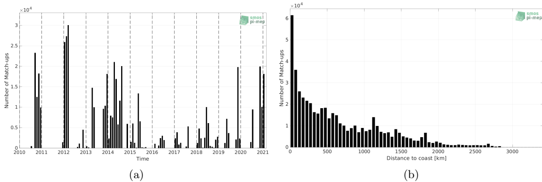
Figure 1: Number of match-ups between TSG (GOSUD-Sailing-ship) and SMOS SSS L3 v8 - 9 Days (CATDS-CECOS-LOCEAN) SSS as a function of time (a) and as function of the distance to coast (b) over the Atlantic Ocean Pi-MEP region and for the full satellite product period.
