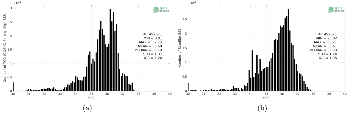
Figure 2: Histograms of SSS from TSG (GOSUD-Sailing-ship) (a) and SMOS SSS L3 v8 - 9 Days (CATDS-CECOS-LOCEAN) (b) considering all match-up pairs per bins of 0.1 over the Atlantic Ocean Pi-MEP region and for the full satellite product period.
