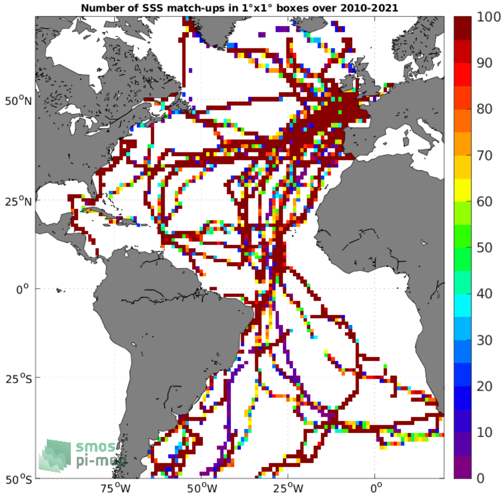
Figure 4: Number of SSS match-ups between TSG (GOSUD-Sailing-ship) SSS and the SMOS SSS L3 v8 - 9 Days (CATDS-CECOS-LOCEAN) SSS product for the Atlantic Ocean Pi-MEP region over 1^\circ \times 1^\circ boxes and for the full satellite product period.
