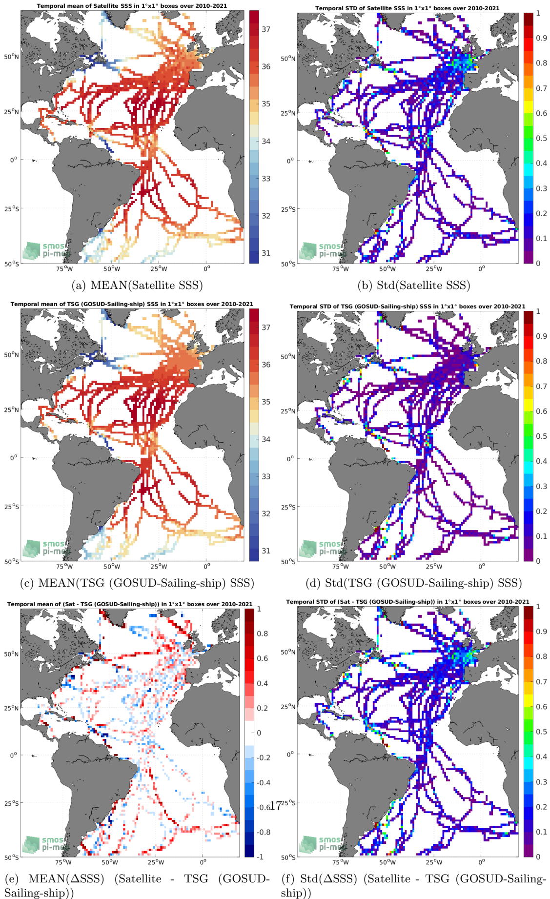
Figure 6: Temporal mean (left) and Std (right) of SSS from SMOS SSS L3 v8 - 9 Days (CATDS-CECOS-LOCEAN) (top), TSG (GOSUD-Sailing-ship) (middle), and of \Delta SSS (Satellite - TSG (GOSUD-Sailing-ship)). Only match-up pairs are used to generate these maps.
