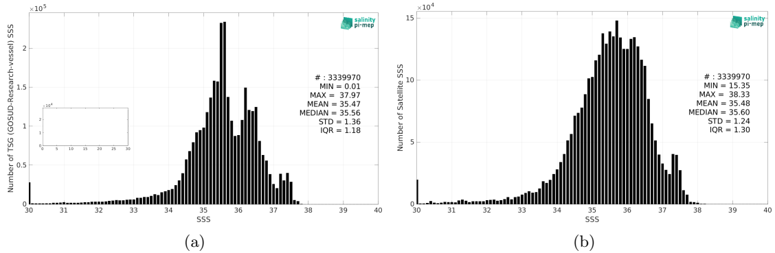
Figure 2: Histograms of SSS from TSG (GOSUD-Research-vessel) (a) and SMOS SSS L3 v8 - 9 Days (CATDS-CEC-LOCEAN) (b) considering all match-up pairs per bins of 0.1 over the Atlantic Ocean Pi-MEP region and for the full satellite product period.
