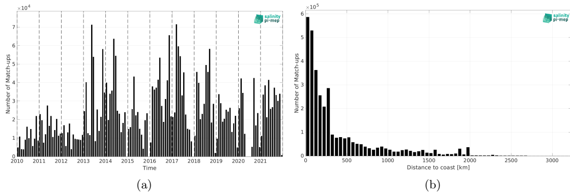
Figure 1: Number of match-ups between TSG (GOSUD-Research-vessel) and SMOS SSS L3 v8 - 9 Days (CATDS-CEC-LOCEAN) SSS as a function of time (a) and as function of the distance to coast (b) over the Atlantic Ocean Pi-MEP region and for the full satellite product period.
