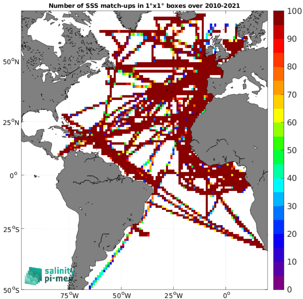
Figure 4: Number of SSS match-ups between TSG (GOSUD-Research-vessel) SSS and the SMOS SSS L3 v8 - 9 Days (CATDS-CEC-LOCEAN) SSS product for the Atlantic Ocean Pi-MEP region over 1°x1° boxes and for the full satellite product period.
