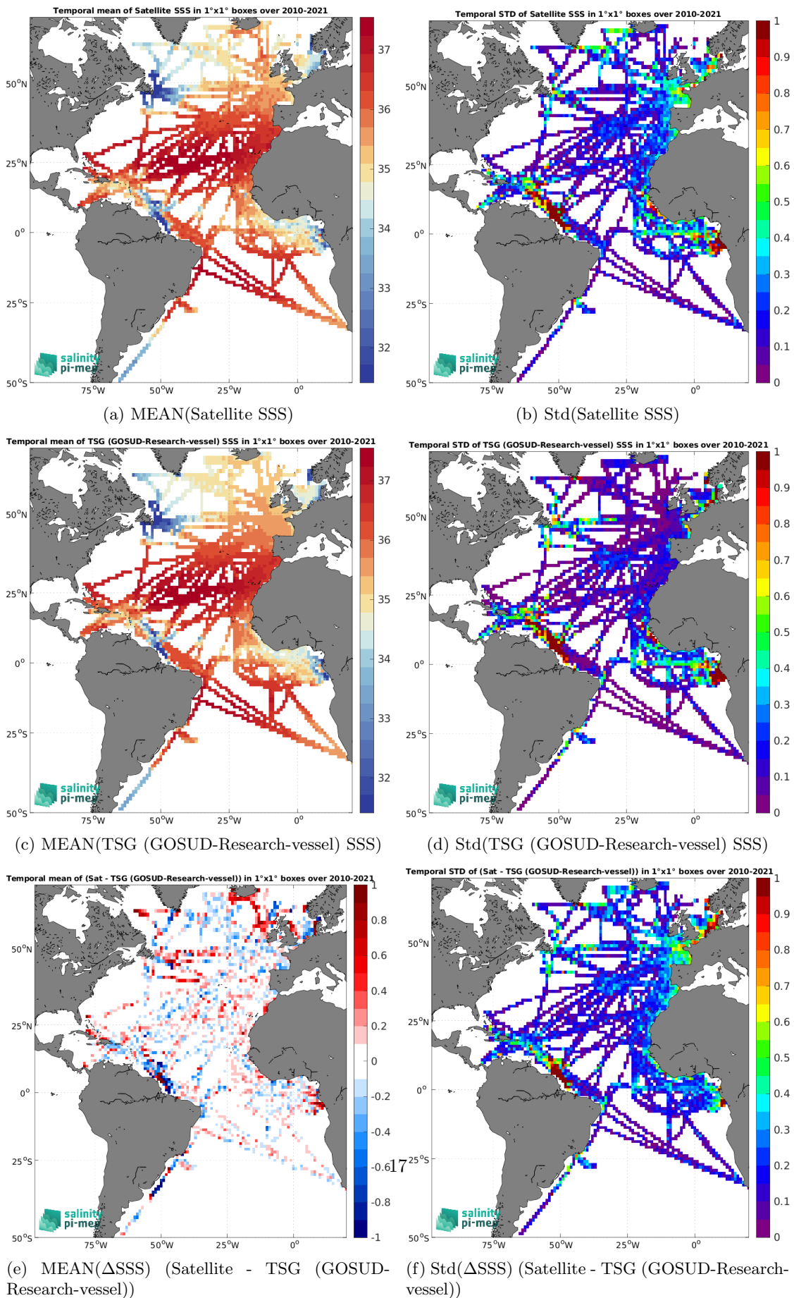
Figure 6: Temporal mean (left) and Std (right) of SSS from SMOS SSS L3 v8 - 9 Days (CATDS-CEC-LOCEAN) (top), TSG (GOSUD-Research-vessel) (middle), and of \Delta SSS (Satellite - TSG (GOSUD-Research-vessel)). Only match-up pairs are used to generate these maps.
