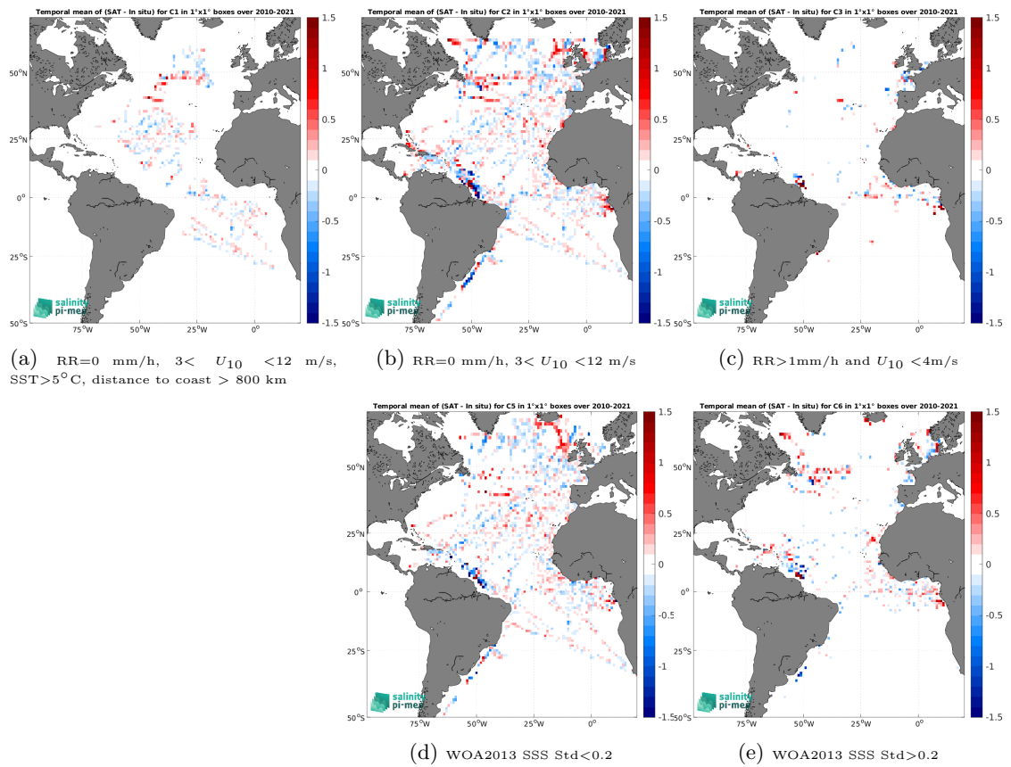
Figure 12: Temporal mean gridded over spatial boxes of size 1^\circ \times 1^\circ of \Delta\text{SSS} (SMOS SSS L3 v8 - 9 Days (CATDS-CEC-LOCEAN) - TSG (GOSUD-Research-vessel)) for 5 different subdatasets corresponding to:RR=0 mm/h, 3 < U_{10} < 12 m/s, SST>5°C, distance to coast > 800 km (a), RR=0 mm/h, 3 < U_{10} < 12 m/s (b), RR>1mm/h and U_{10} < 4 m/s (c), WOA2013 SSS Std<0.2 (d), WOA2013 SSS Std>0.2 (e).
