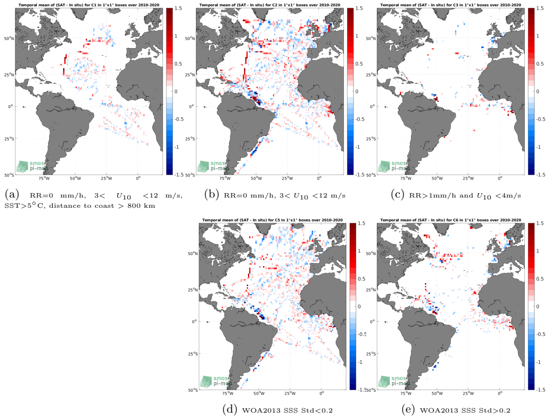
Figure 12: Temporal mean gridded over spatial boxes of size 1^\circ \times 1^\circ of \Delta\text{SSS} (SMOS SSS L3 v8 - 9 Days (CATDS-CECOS-LOCEAN) - TSG (GOSUD-Research-vessel)) for 5 different subdatasets corresponding to:RR=0 mm/h, 3 < U_{10} < 12 m/s, SST>5°C, distance to coast > 800 km (a), RR=0 mm/h, 3 < U_{10} < 12 m/s (b), RR>1mm/h and U_{10} < 4 m/s (c), WOA2013 SSS Std<0.2 (d), WOA2013 SSS Std>0.2 (e).
