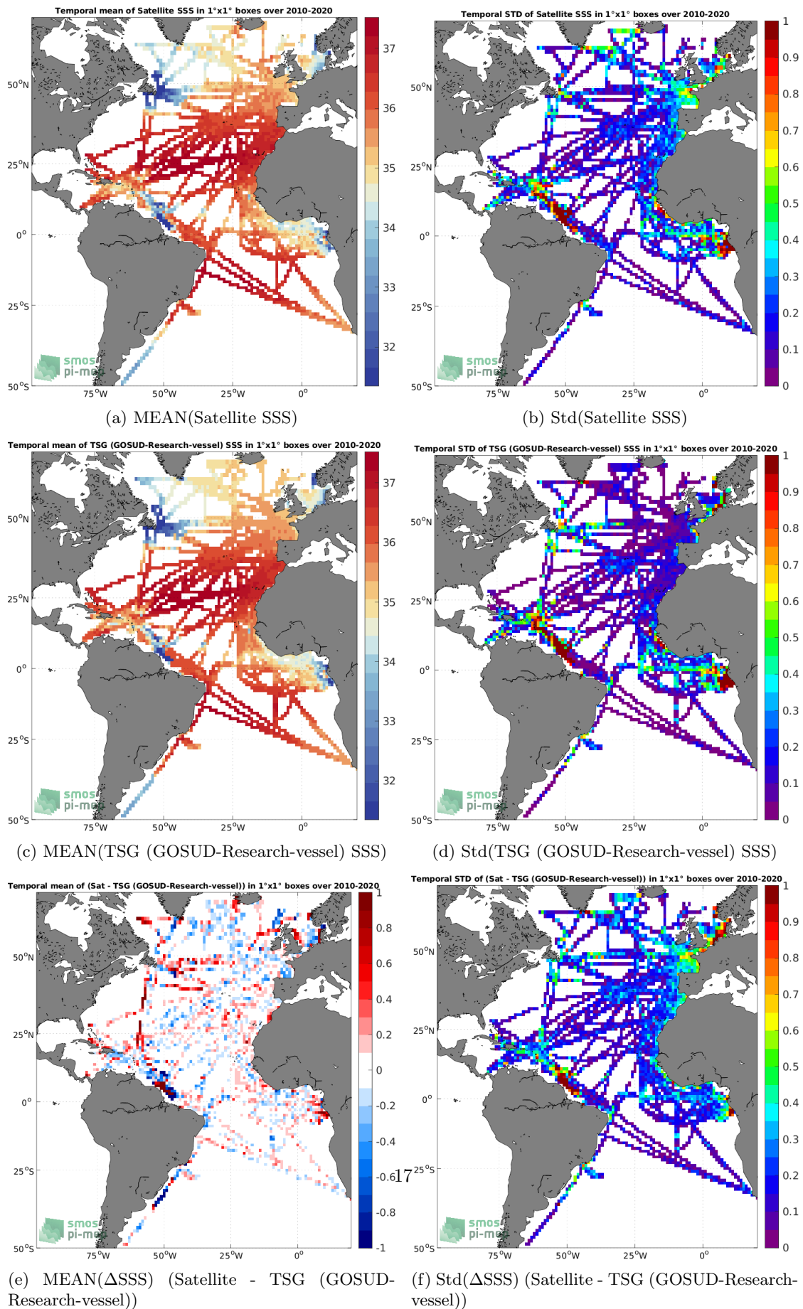
Figure 6: Temporal mean (left) and Std (right) of SSS from SMOS SSS L3 v8 - 9 Days (CATDS-CECOS-LOCEAN) (top), TSG (GOSUD-Research-vessel) (middle), and of \Delta SSS (Satellite - TSG (GOSUD-Research-vessel)). Only match-up pairs are used to generate these maps.
