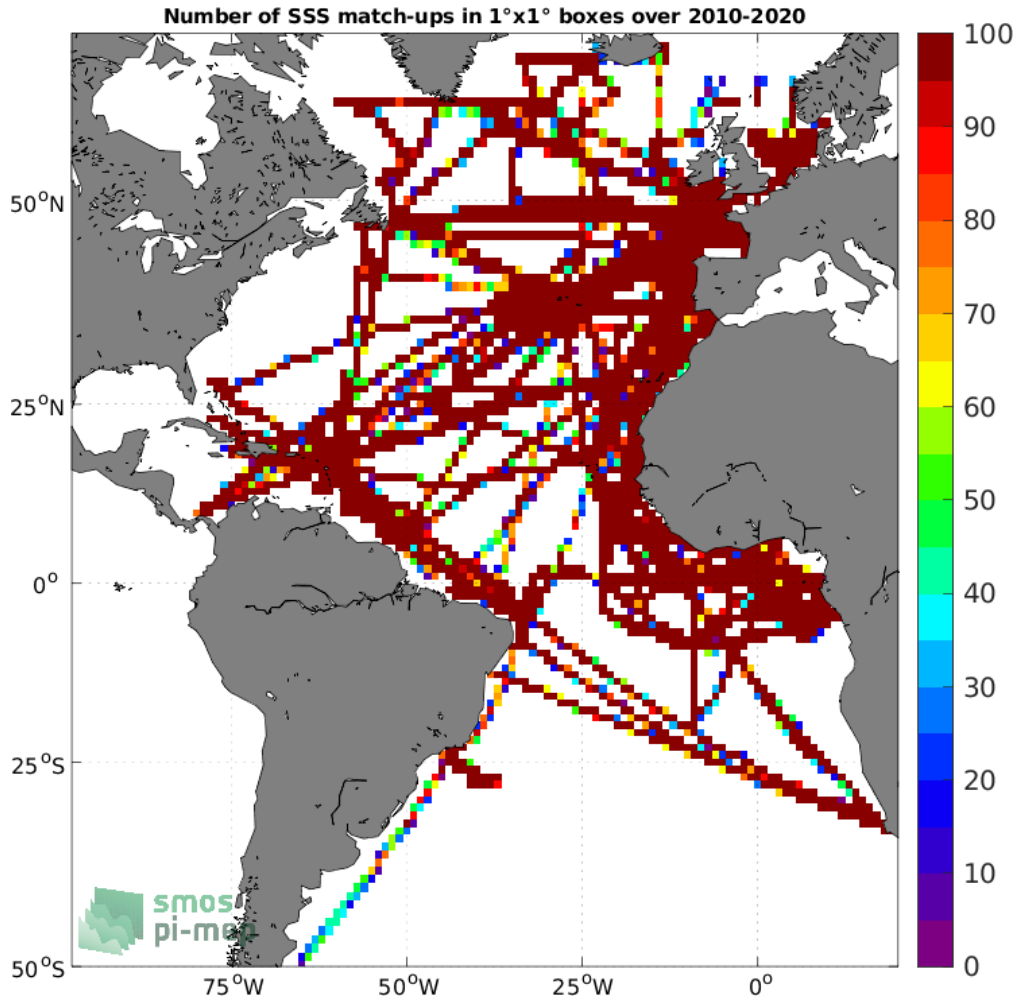
Figure 4: Number of SSS match-ups between TSG (GOSUD-Research-vessel) SSS and the SMOS SSS L3 v8 - 9 Days (CATDS-CECOS-LOCEAN) SSS product for the Atlantic Ocean Pi-MEP region over 1^{\circ} \times 1^{\circ} boxes and for the full satellite product period.
