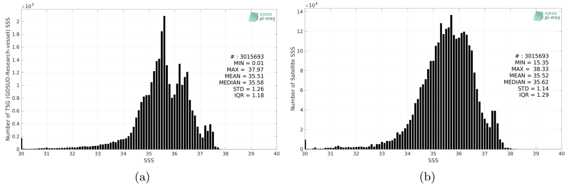
Figure 2: Histograms of SSS from TSG (GOSUD-Research-vessel) (a) and SMOS SSS L3 v8 - 9 Days (CATDS-CECOS-LOCEAN) (b) considering all match-up pairs per bins of 0.1 over the Atlantic Ocean Pi-MEP region and for the full satellite product period.
