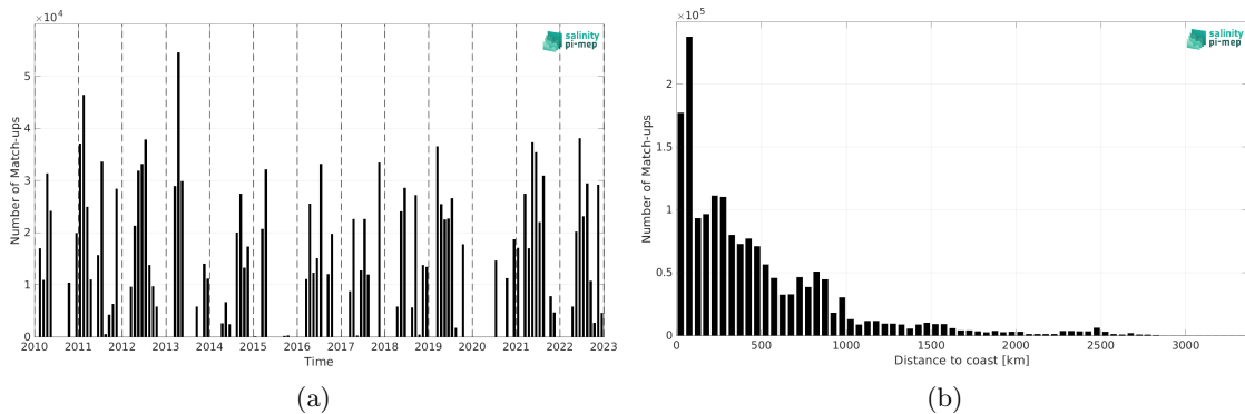
Figure 1: Number of match-ups between TSG (CSIC-UTM) and SMOS SSS L3 v8 - 9 Days (CATDS-CEC-LOCEAN) SSS as a function of time (a) and as function of the distance to coast (b) over the Atlantic Ocean Pi-MEP region and for the full satellite product period.
