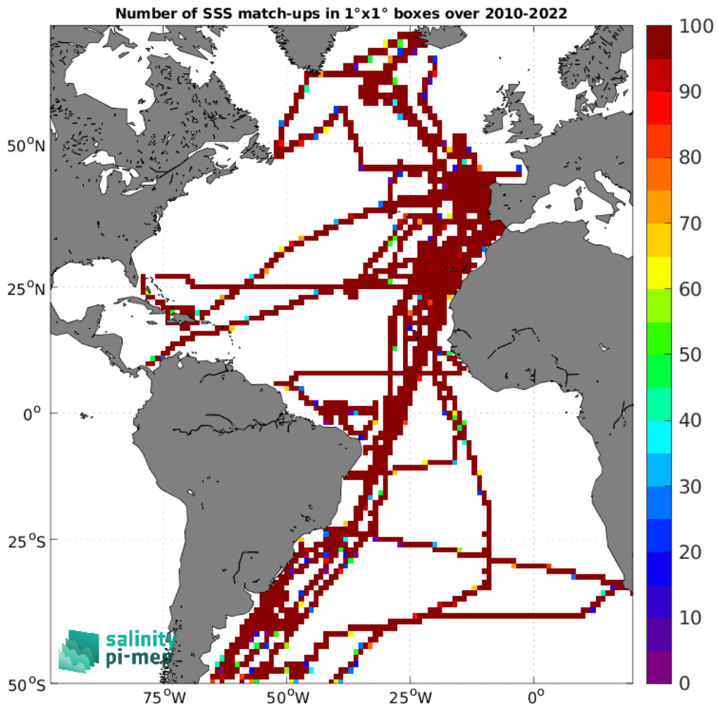
Figure 4: Number of SSS match-ups between TSG (CSIC-UTM) SSS and the SMOS SSS L3 v8 - 9 Days (CATDS-CEC-LOCEAN) SSS product for the Atlantic Ocean Pi-MEP region over 1^\circ \times 1^\circ boxes and for the full satellite product period.
