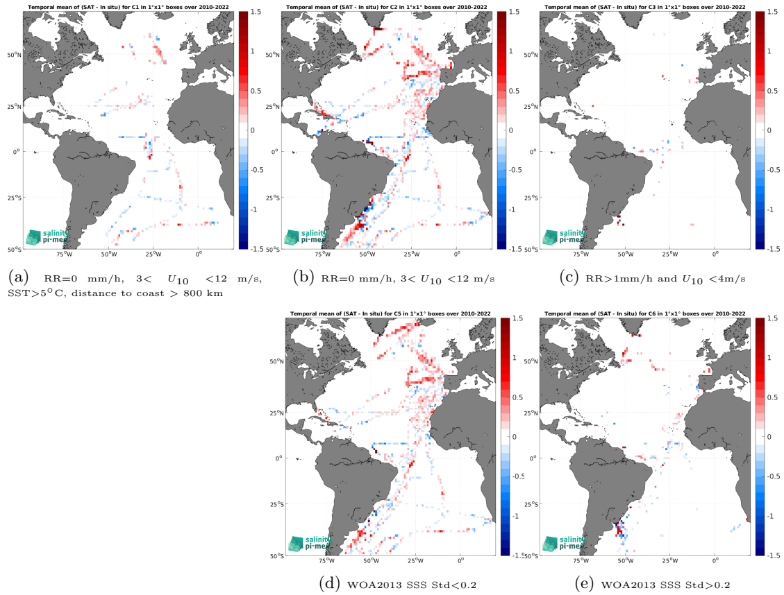
Figure 12: Temporal mean gridded over spatial boxes of size 1^\circ \times 1^\circ of \Delta SSS (SMOS SSS L3 v8 - 9 Days (CATDS-CEC-LOCEAN) - TSG (CSIC-UTM)) for 5 different subdatasets corresponding to:RR=0 mm/h, 3 < U_{10} < 12 m/s, SST >5^\circ\text{C} , distance to coast > 800 km (a), RR=0 mm/h, 3 < U_{10} < 12 m/s (b), RR >1 mm/h and U_{10} < 4 m/s (c), WOA2013 SSS Std <0.2 (d), WOA2013 SSS Std >0.2 (e).
