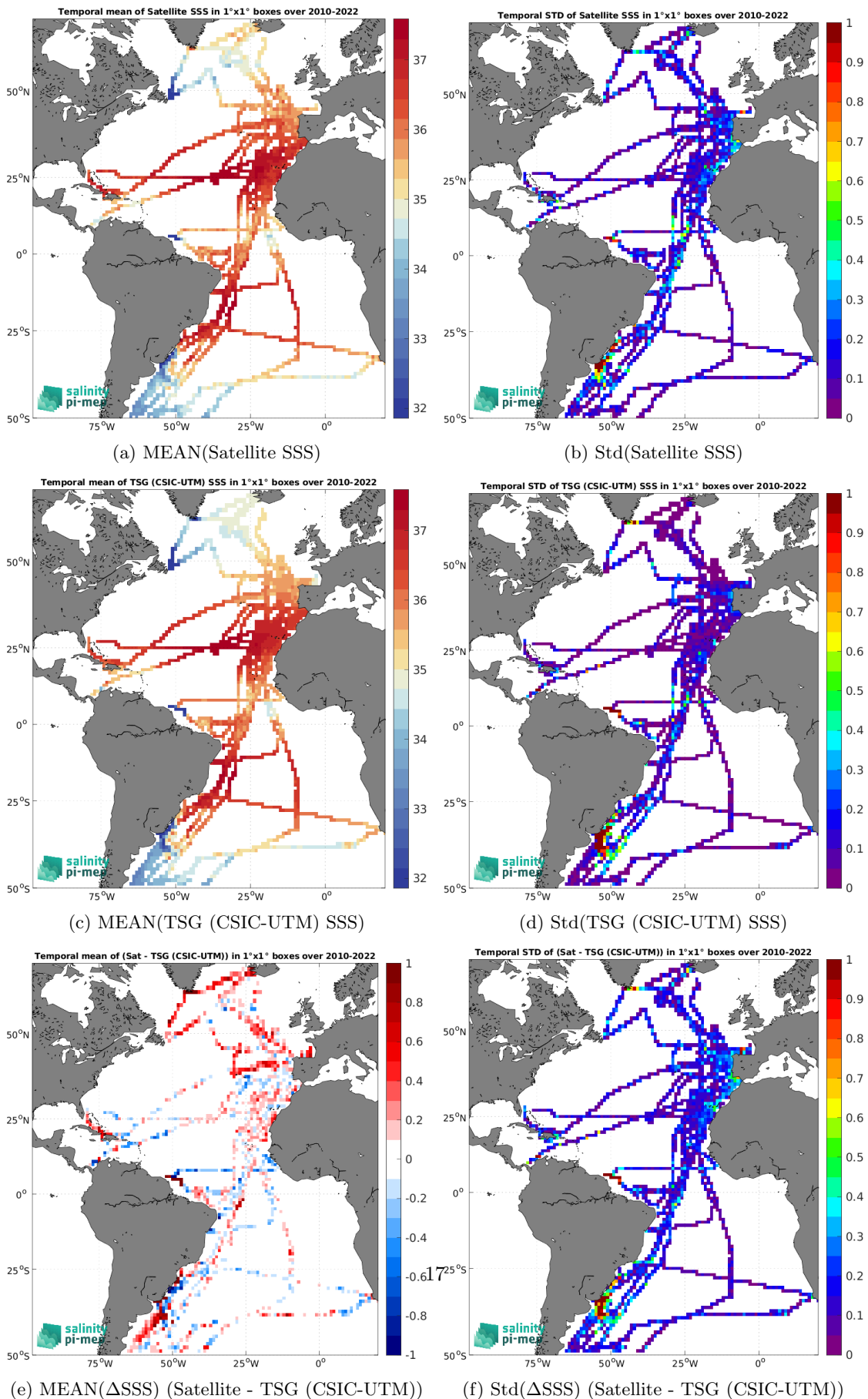
Figure 6: Temporal mean (left) and Std (right) of SSS from SMOS SSS L3 v8 - 9 Days (CATDS-CEC-LOCEAN) (top), TSG (CSIC-UTM) (middle), and of \Delta SSS (Satellite - TSG (CSIC-UTM)). Only match-up pairs are used to generate these maps.
