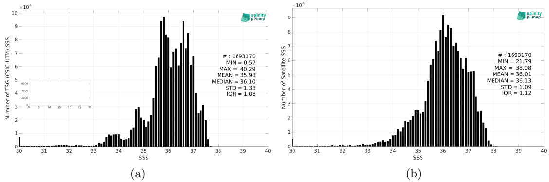
Figure 2: Histograms of SSS from TSG (CSIC-UTM) (a) and SMOS SSS L3 v8 - 9 Days (CATDS-CEC-LOCEAN) (b) considering all match-up pairs per bins of 0.1 over the Atlantic Ocean Pi-MEP region and for the full satellite product period.
