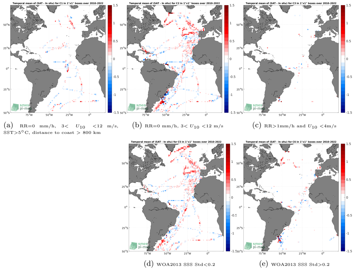
Figure 12: Temporal mean gridded over spatial boxes of size 1^\circ \times 1^\circ of \Delta SSS (SMOS SSS L3 v8 - 9 Days (CATDS-CECOS-LOCEAN) - TSG (CSIC-UTM)) for 5 different subdatasets corresponding to:RR=0 mm/h, 3 < U_{10} < 12 m/s, SST >5^\circ\text{C} , distance to coast > 800 km (a), RR=0 mm/h, 3 < U_{10} < 12 m/s (b), RR >1 mm/h and U_{10} < 4 m/s (c), WOA2013 SSS Std <0.2 (d), WOA2013 SSS Std >0.2 (e).
