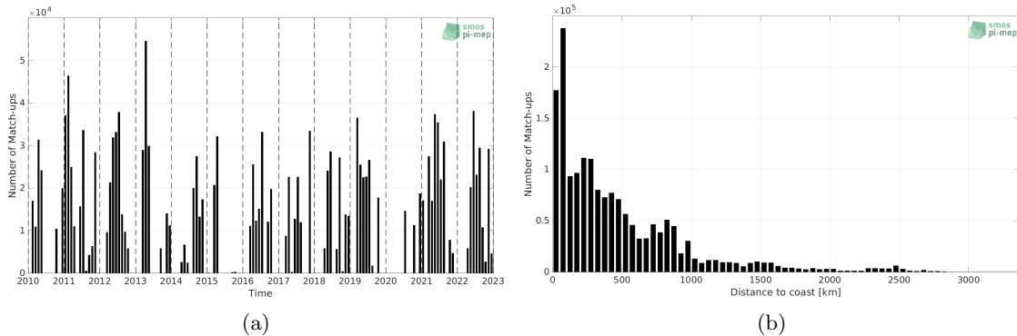
Figure 1: Number of match-ups between TSG (CSIC-UTM) and SMOS SSS L3 v8 - 9 Days (CATDS-CECOS-LOCEAN) SSS as a function of time (a) and as function of the distance to coast (b) over the Atlantic Ocean Pi-MEP region and for the full satellite product period.
