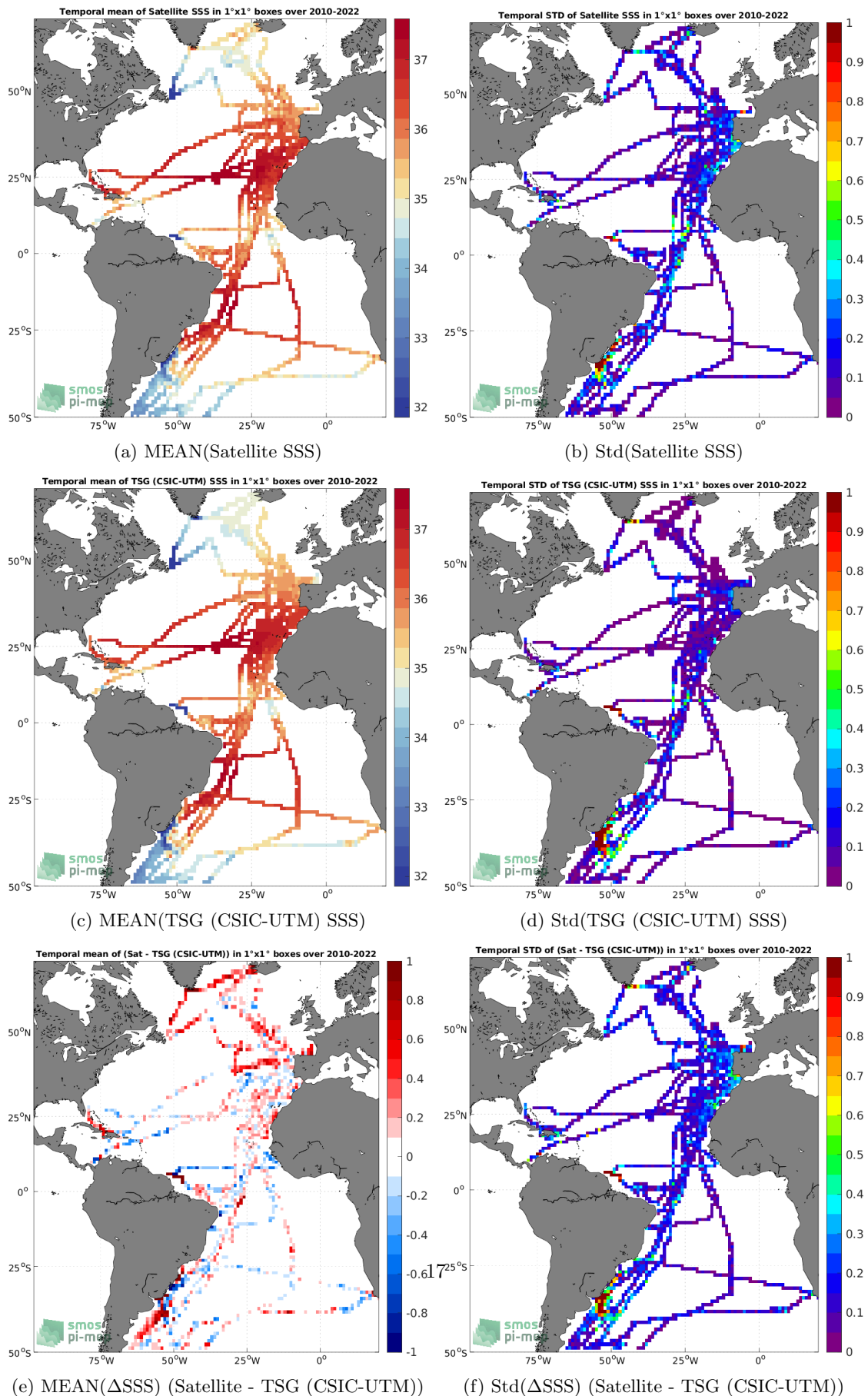
Figure 6: Temporal mean (left) and Std (right) of SSS from SMOS SSS L3 v8 - 9 Days (CATDS-CECOS-LOCEAN) (top), TSG (CSIC-UTM) (middle), and of \Delta SSS (Satellite - TSG (CSIC-UTM)). Only match-up pairs are used to generate these maps.
