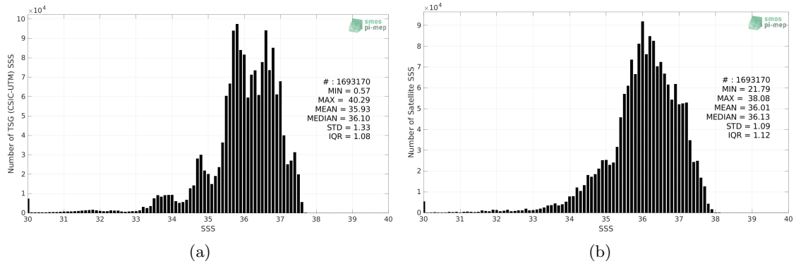
Figure 2: Histograms of SSS from TSG (CSIC-UTM) (a) and SMOS SSS L3 v8 - 9 Days (CATDS-CECOS-LOCEAN) (b) considering all match-up pairs per bins of 0.1 over the Atlantic Ocean Pi-MEP region and for the full satellite product period.
