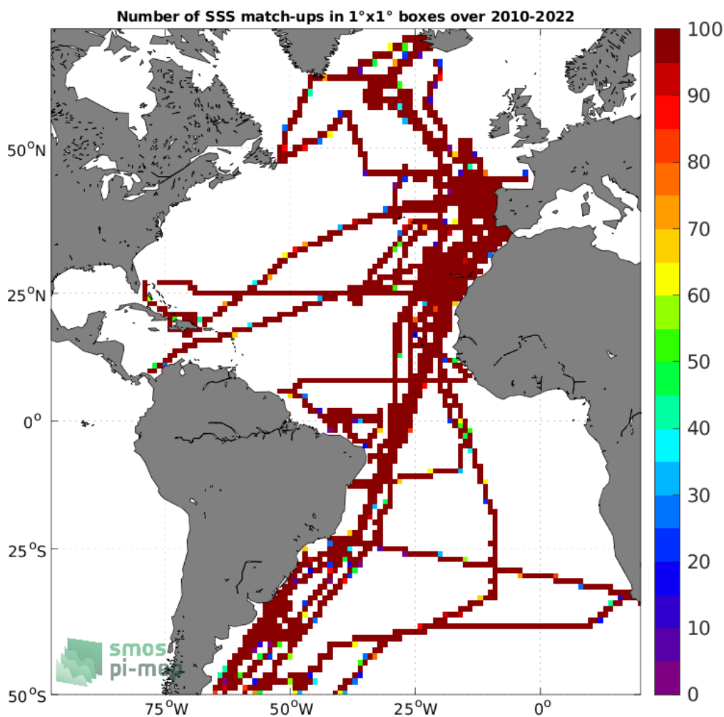
Figure 4: Number of SSS match-ups between TSG (CSIC-UTM) SSS and the SMOS SSS L3 v8 - 9 Days (CATDS-CECOS-LOCEAN) SSS product for the Atlantic Ocean Pi-MEP region over 1^\circ \times 1^\circ boxes and for the full satellite product period.
