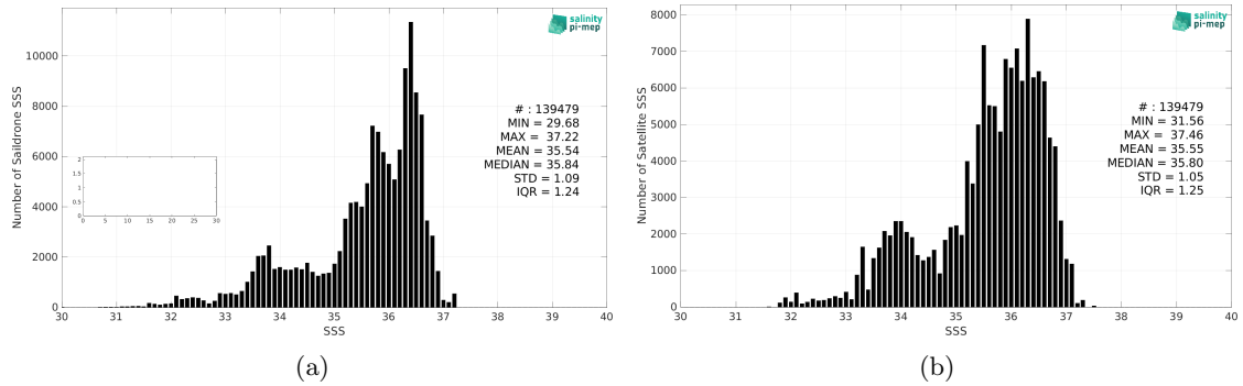
Figure 2: Histograms of SSS from Sairdrone (a) and SMOS SSS L3 v8 - 9 Days (CATDS-CEC-LOCEAN) (b) considering all match-up pairs per bins of 0.1 over the Atlantic Ocean Pi-MEP region and for the full satellite product period.
