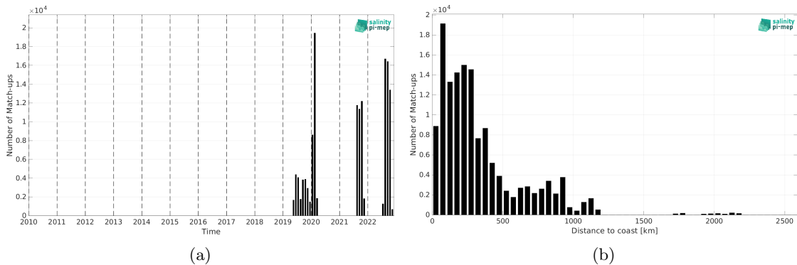
Figure 1: Number of match-ups between Saildrone and SMOS SSS L3 v8 - 9 Days (CATDS-CEC-LOCEAN) SSS as a function of time (a) and as function of the distance to coast (b) over the Atlantic Ocean Pi-MEP region and for the full satellite product period.
