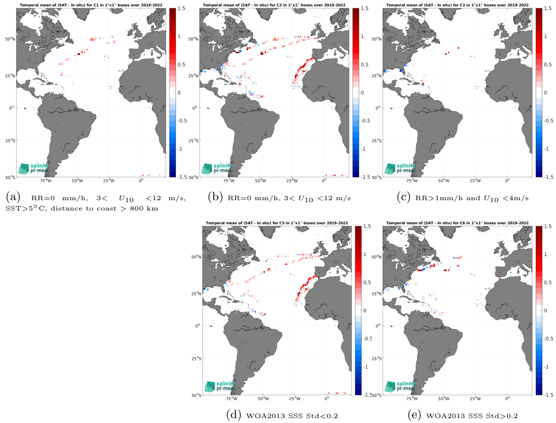
Figure 12: Temporal mean gridded over spatial boxes of size 1^\circ \times 1^\circ of \Delta\text{SSS} (SMOS SSS L3 v8 - 9 Days (CATDS-CEC-LOCEAN) - Saildrone) for 5 different subdatasets corresponding to:RR=0 mm/h, 3 < U_{10} < 12 m/s, SST >5^\circ\text{C} , distance to coast > 800 km (a), RR=0 mm/h, 3 < U_{10} < 12 m/s (b), RR >1 mm/h and U_{10} < 4 m/s (c), WOA2013 SSS Std <0.2 (d), WOA2013 SSS Std >0.2 (e).
