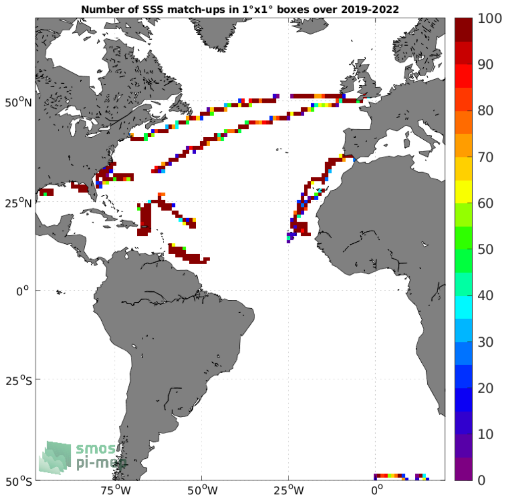
Figure 4: Number of SSS match-ups between Saildrone SSS and the SMOS SSS L3 v8 - 9 Days (CATDS-CECOS-LOCEAN) SSS product for the Atlantic Ocean Pi-MEP region over 1°x1° boxes and for the full satellite product period.
