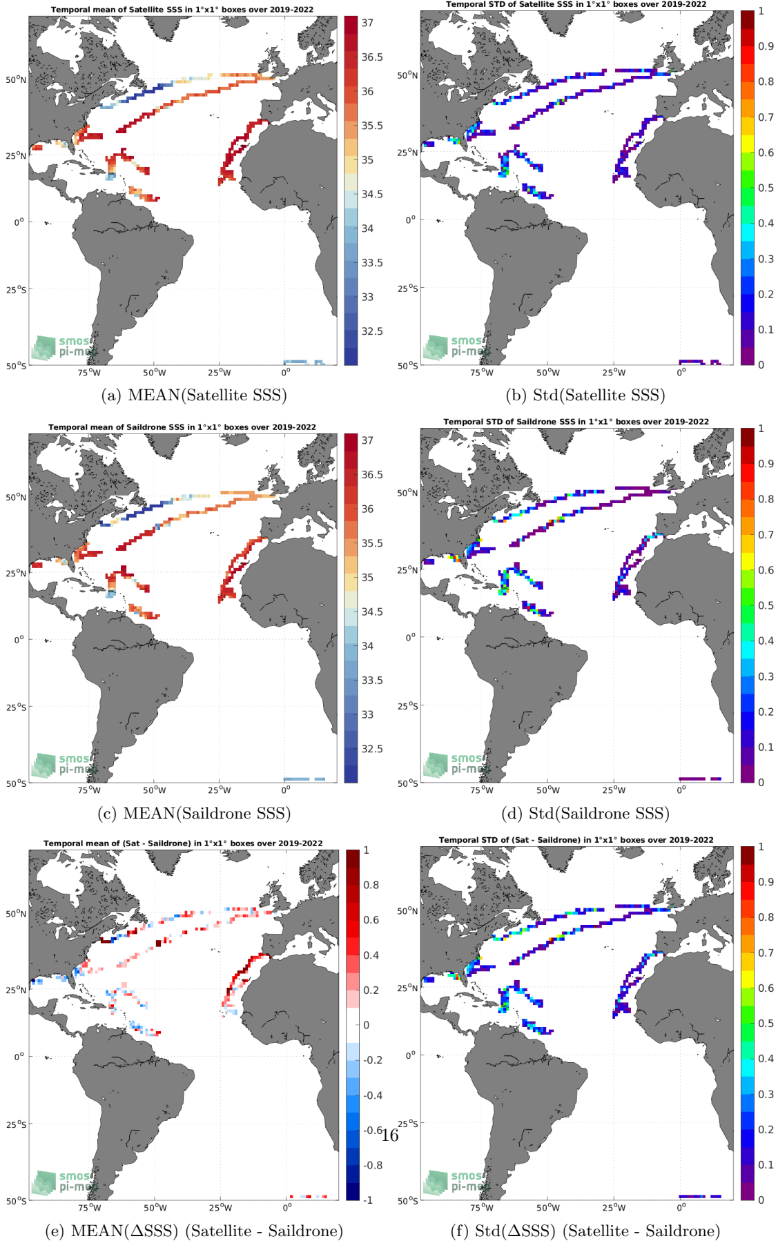
(e) MEAN( \Delta SSS) (Satellite - Saildrone) (f) Std( \Delta SSS) (Satellite - Saildrone) Figure 6: Temporal mean (left) and Std (right) of SSS from SMOS SSS L3 v8 - 9 Days (CATDS-CECOS-LOCEAN) (top), Saildrone (middle), and of \Delta SSS (Satellite - Saildrone). Only match-up pairs are used to generate these maps.
