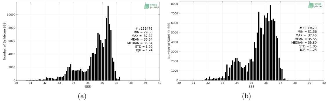
Figure 2: Histograms of SSS from Saildrone (a) and SMOS SSS L3 v8 - 9 Days (CATDS-CECOS-LOCEAN) (b) considering all match-up pairs per bins of 0.1 over the Atlantic Ocean Pi-MEP region and for the full satellite product period.
