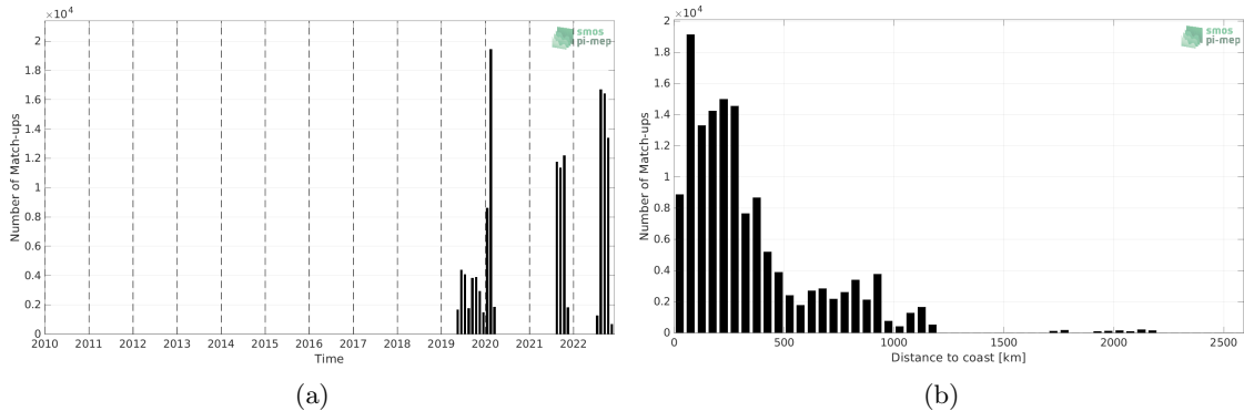
Figure 1: Number of match-ups between Saildrone and SMOS SSS L3 v8 - 9 Days (CATDS-CECOS-LOCEAN) SSS as a function of time (a) and as function of the distance to coast (b) over the Atlantic Ocean Pi-MEP region and for the full satellite product period.
