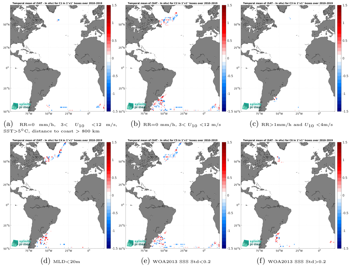
Figure 12: Temporal mean gridded over spatial boxes of size 1^\circ \times 1^\circ of \Delta\text{SSS} (SMOS SSS L3 v8 - 9 Days (CATDS-CEC-LOCEAN) - Marine mammals) for 6 different subdatasets corresponding to: RR=0 mm/h, 3 < U_{10} < 12 m/s, SST > 5^\circ\text{C} , distance to coast > 800 km (a), RR=0 mm/h, 3 < U_{10} < 12 m/s (b), RR > 1 mm/h and U_{10} < 4 m/s (c), MLD < 20 m (d), WOA2013 SSS Std < 0.2 (e), WOA2013 SSS Std > 0.2 (f).
