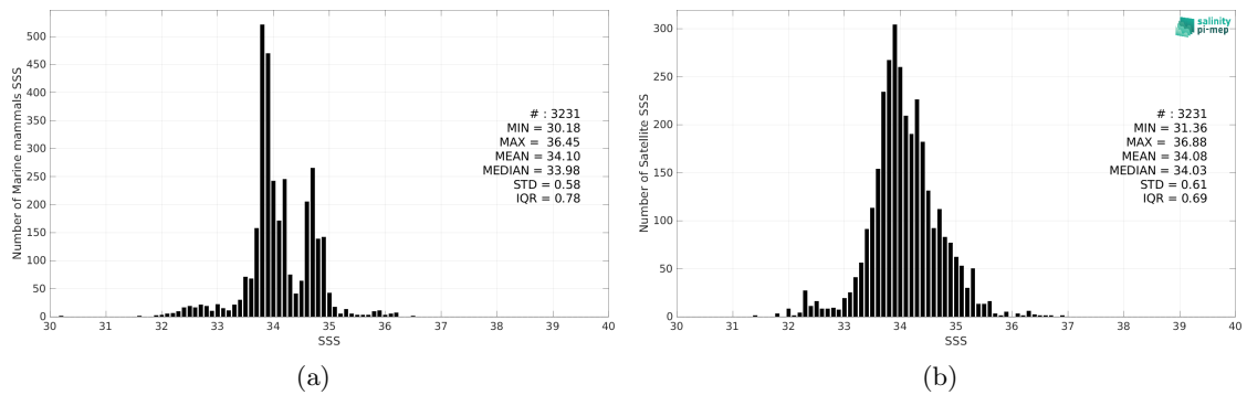
Figure 2: Histograms of SSS from Marine mammals (a) and SMOS SSS L3 v8 - 9 Days (CATDS-CEC-LOCEAN) (b) considering all match-up pairs per bins of 0.1 over the Atlantic Ocean Pi-MEP region and for the full satellite product period.
