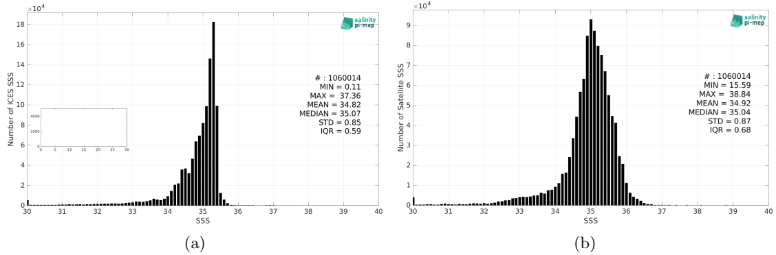
Figure 2: Histograms of SSS from ICES (a) and SMOS SSS L3 v8 - 9 Days (CATDS-CEC-LOCEAN) (b) considering all match-up pairs per bins of 0.1 over the Atlantic Ocean Pi-MEP region and for the full satellite product period.
