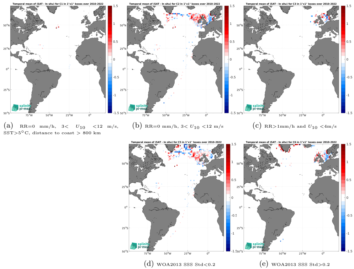
Figure 12: Temporal mean gridded over spatial boxes of size 1^\circ \times 1^\circ of \Delta SSS (SMOS SSS L3 v8 - 9 Days (CATDS-CEC-LOCEAN) - ICES) for 5 different subdatasets corresponding to:RR=0 mm/h, 3 < U_{10} < 12 m/s, SST >5^\circ\text{C} , distance to coast > 800 km (a), RR=0 mm/h, 3 < U_{10} < 12 m/s (b), RR >1 mm/h and U_{10} < 4 m/s (c), WOA2013 SSS Std <0.2 (d), WOA2013 SSS Std >0.2 (e).
