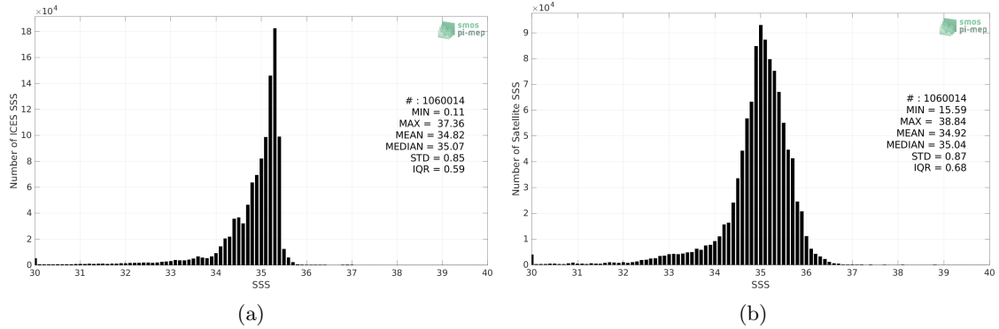
Figure 2: Histograms of SSS from ICES (a) and SMOS SSS L3 v8 - 9 Days (CATDS-CECOS-LOCEAN) (b) considering all match-up pairs per bins of 0.1 over the Atlantic Ocean Pi-MEP region and for the full satellite product period.
