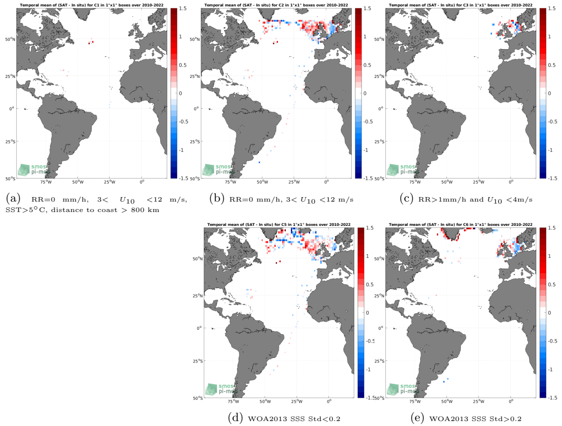
Figure 12: Temporal mean gridded over spatial boxes of size 1^\circ \times 1^\circ of \Delta SSS (SMOS SSS L3 v8 - 9 Days (CATDS-CECOS-LOCEAN) - ICES) for 5 different subdatasets corresponding to:RR=0 mm/h, 3 < U_{10} < 12 m/s, SST >5^\circ\text{C} , distance to coast > 800 km (a), RR=0 mm/h, 3 < U_{10} < 12 m/s (b), RR >1 mm/h and U_{10} < 4 m/s (c), WOA2013 SSS Std <0.2 (d), WOA2013 SSS Std >0.2 (e).
