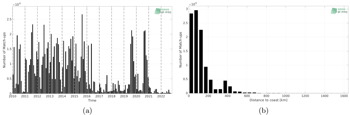
Figure 1: Number of match-ups between ICES and SMOS SSS L3 v8 - 9 Days (CATDS-CECOS-LOCEAN) SSS as a function of time (a) and as function of the distance to coast (b) over the Atlantic Ocean Pi-MEP region and for the full satellite product period.
