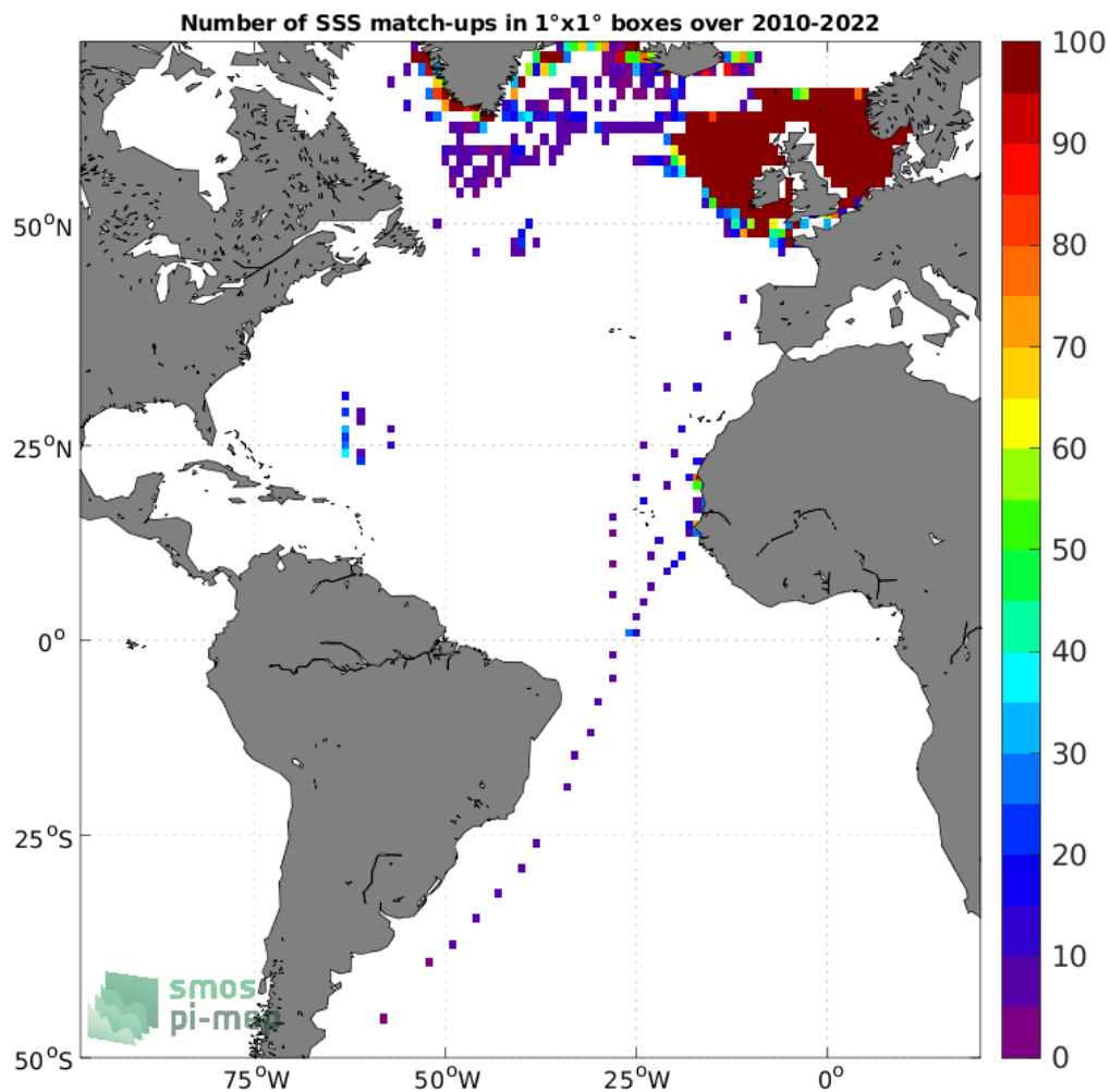
Figure 4: Number of SSS match-ups between ICES SSS and the SMOS SSS L3 v8 - 9 Days (CATDS-CECOS-LOCEAN) SSS product for the Atlantic Ocean Pi-MEP region over 1°x1° boxes and for the full satellite product period.
