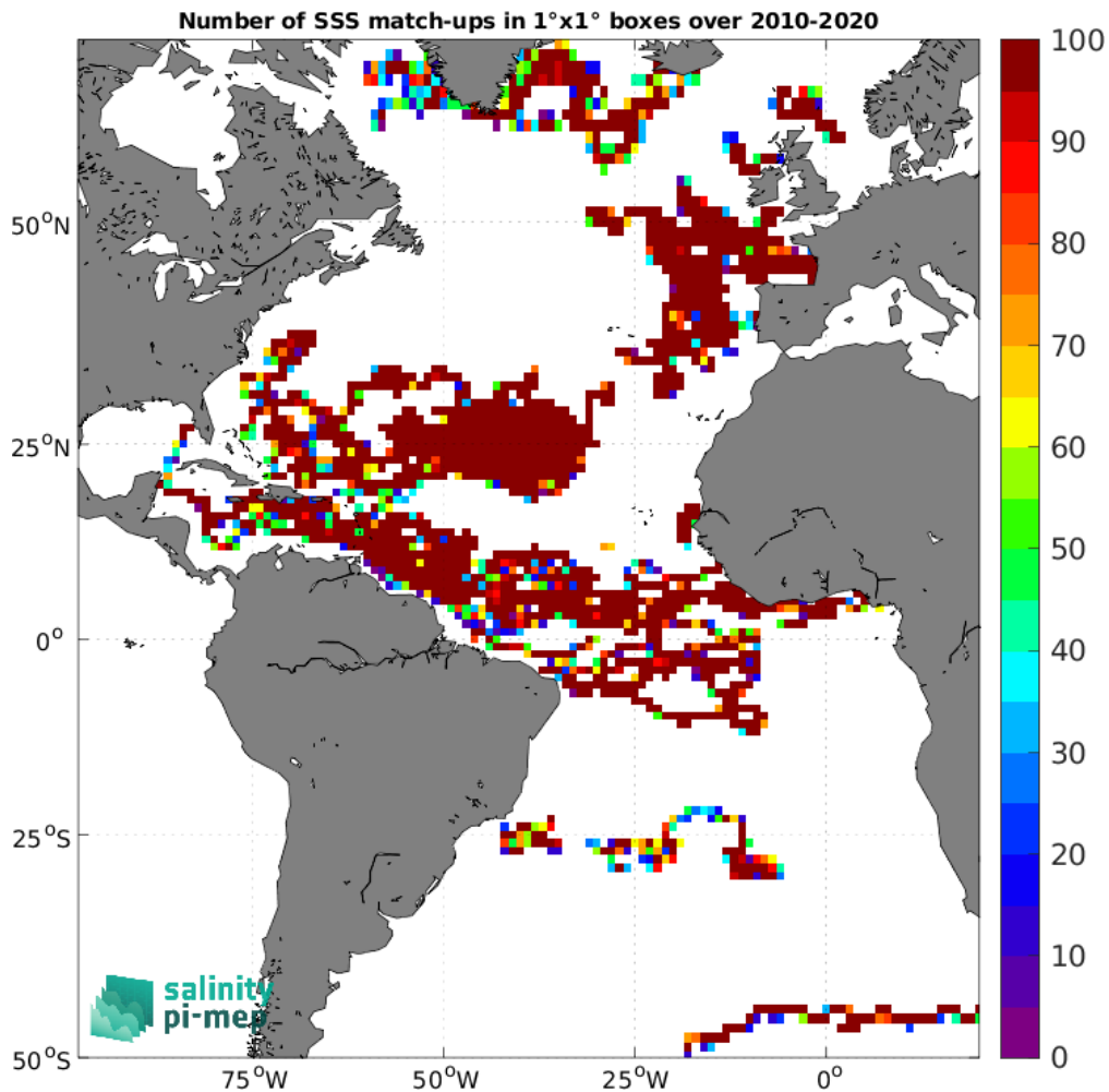
Figure 3: Number of SSS match-ups between Surface drifters SSS and the SMOS SSS L3 v8 - 9 Days (CATDS-CEC-LOCEAN) SSS product for the Atlantic Ocean Pi-MEP region over 1°x1° boxes and for the full satellite product period.
