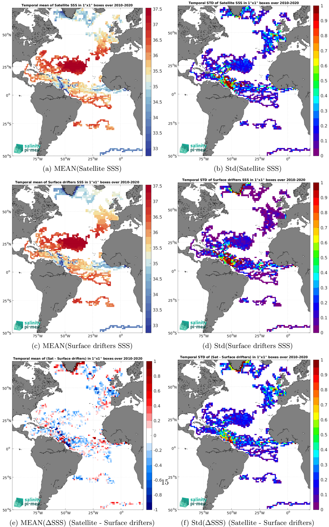
Figure 5: Temporal mean (left) and Std (right) of SSS from SMOS SSS L3 v8 - 9 Days (CATDS-CEC-LOCEAN) (top), Surface drifters (middle), and of \Delta SSS (Satellite - Surface drifters). Only match-up pairs are used to generate these maps.
