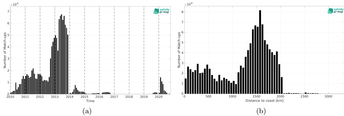
Figure 1: Number of match-ups between Surface drifters and SMOS SSS L3 v8 - 9 Days (CATDS-CEC-LOCEAN) SSS as a function of time (a) and as function of the distance to coast (b) over the Atlantic Ocean Pi-MEP region and for the full satellite product period.
