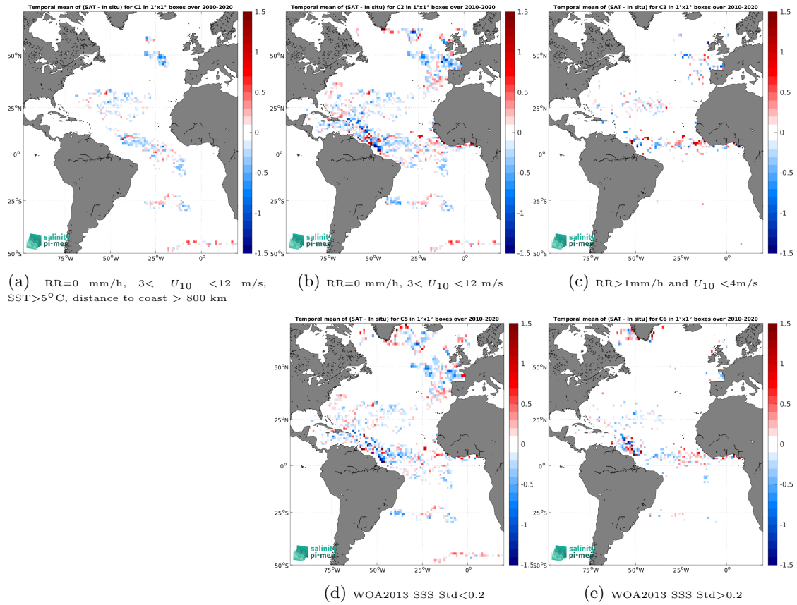
Figure 11: Temporal mean gridded over spatial boxes of size 1^\circ \times 1^\circ of \Delta\text{SSS} (SMOS SSS L3 v8 - 9 Days (CATDS-CEC-LOCEAN) - Surface drifters) for 5 different subdatasets corresponding to:RR=0 mm/h, 3 < U_{10} < 12 m/s, SST >5^\circ\text{C} , distance to coast > 800 km (a), RR=0 mm/h, 3 < U_{10} < 12 m/s (b), RR >1 mm/h and U_{10} < 4 m/s (c), WOA2013 SSS Std <0.2 (d), WOA2013 SSS Std >0.2 (e).
