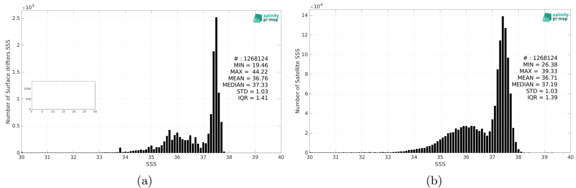
Figure 2: Histograms of SSS from Surface drifters (a) and SMOS SSS L3 v8 - 9 Days (CATDS-CEC-LOCEAN) (b) considering all match-up pairs per bins of 0.1 over the Atlantic Ocean Pi-MEP region and for the full satellite product period.
