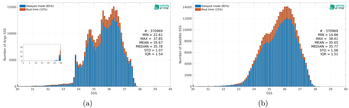
Figure 2: Histograms of SSS from Argo (a) and SMOS SSS L3 v8 - 9 Days (CATDS-CEC-LOCEAN) (b) considering all match-up pairs per bins of 0.1 over the Atlantic Ocean Pi-MEP region and for the full satellite product period.
