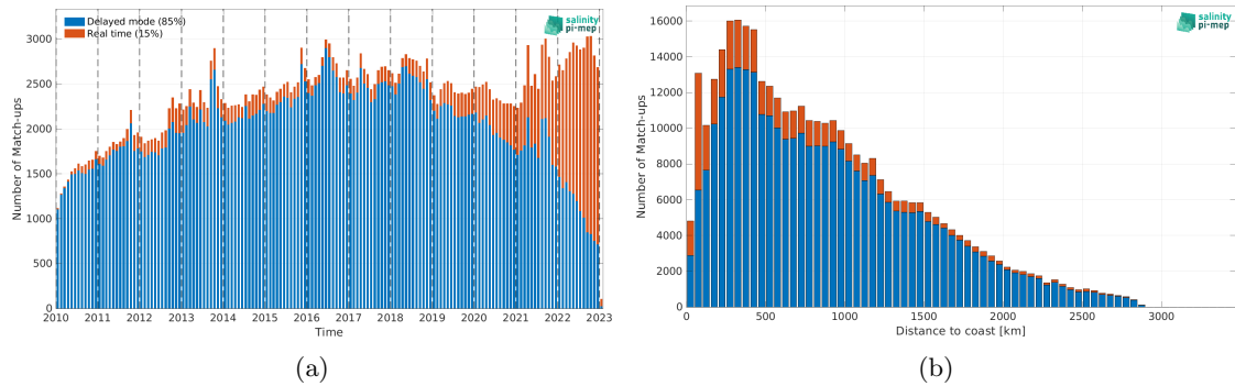
Figure 1: Number of match-ups between Argo and SMOS SSS L3 v8 - 9 Days (CATDS-CEC-LOCEAN) SSS as a function of time (a) and as function of the distance to coast (b) over the Atlantic Ocean Pi-MEP region and for the full satellite product period.
