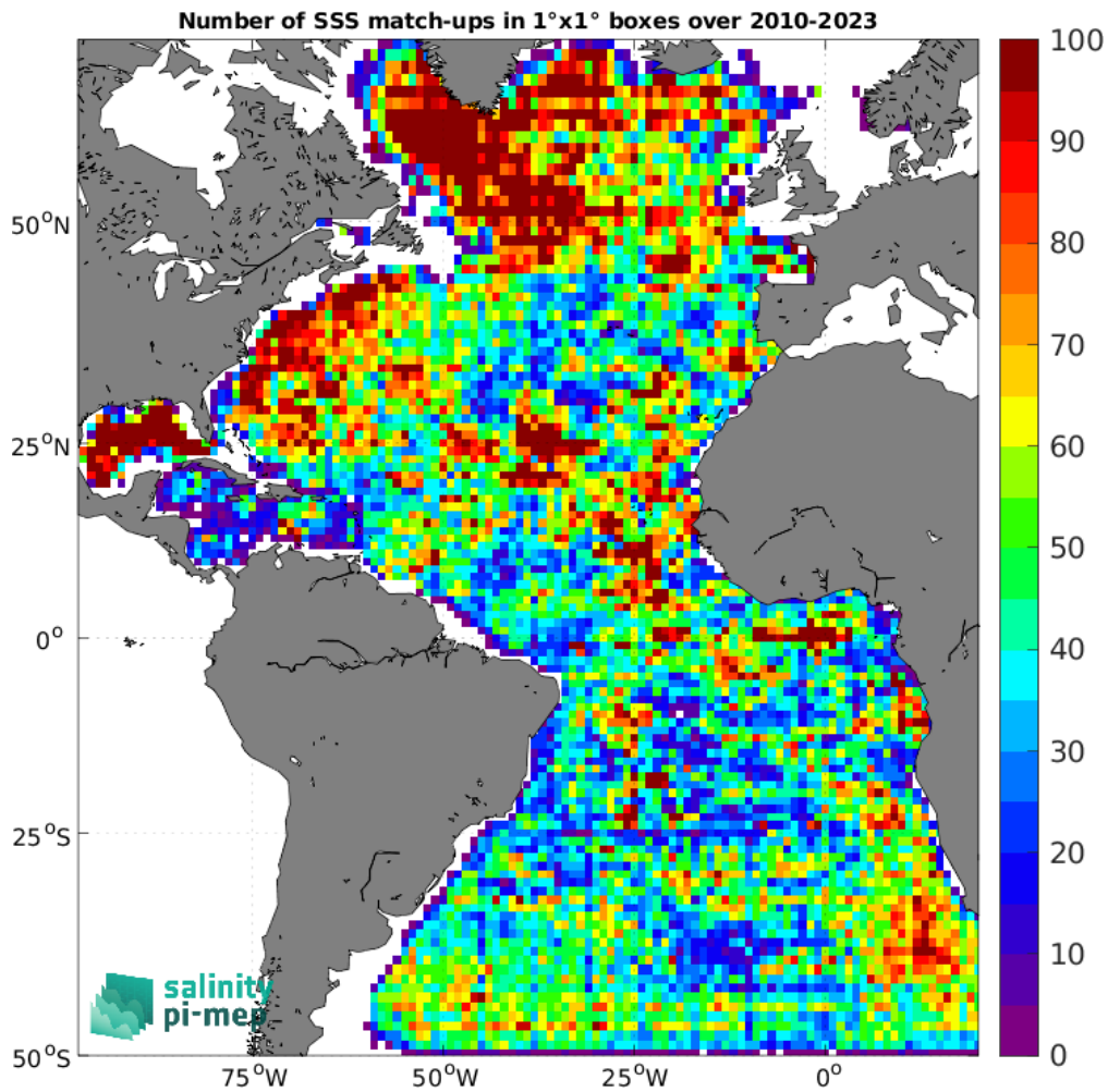
Figure 4: Number of SSS match-ups between Argo SSS and the SMOS SSS L3 v8 - 9 Days (CATDS-CEC-LOCEAN) SSS product for the Atlantic Ocean Pi-MEP region over 1^\circ \times 1^\circ boxes and for the full satellite product period.
